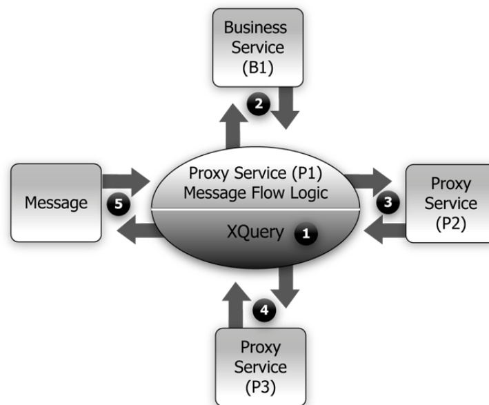
Figure 39-3 Test Scenario Example
