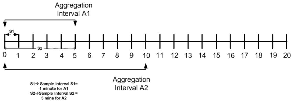
Figure 45–2 Illustration of Aggregation Interval and Sampling Interval
