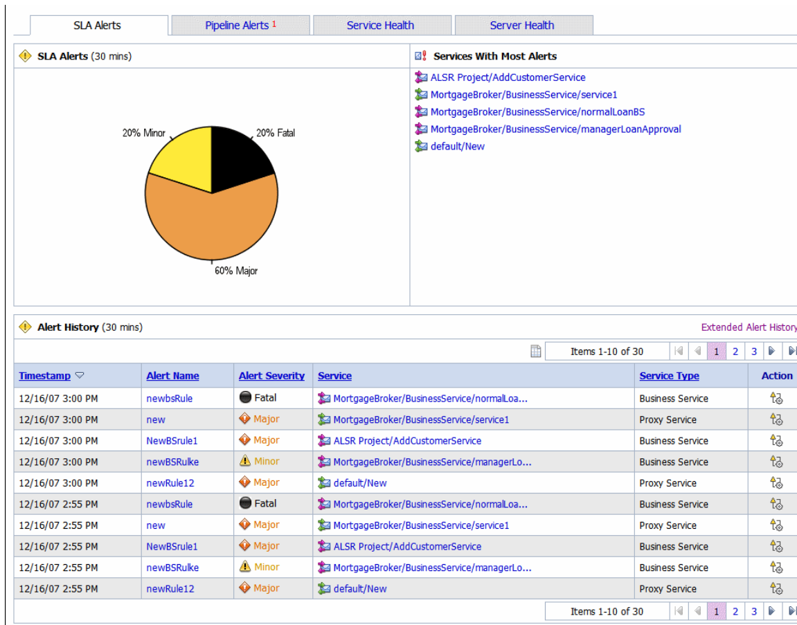
Figure 45–7 Oracle Service Bus Dashboard for SLA Alerts
