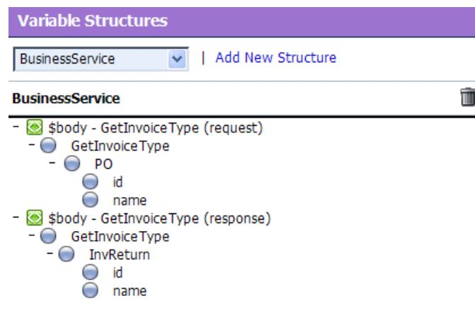
Figure 36–9 Variable Structures—Business Service
