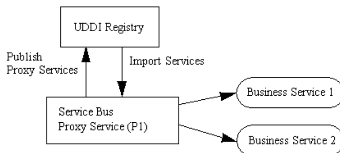
Figure 40–3 Proxy Service Communication with a UDDI Registry
