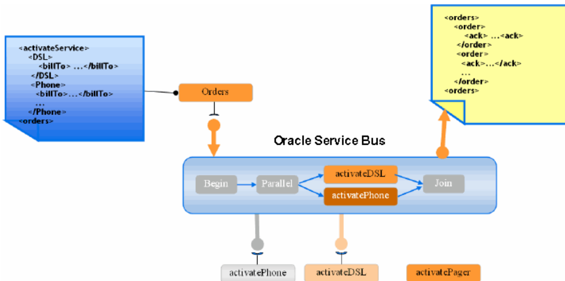
Figure 37–1 Static Split-Join – Known number of service requests
