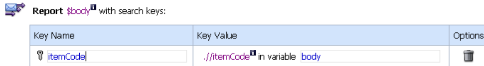
Figure 46–3 Key Name and Value
