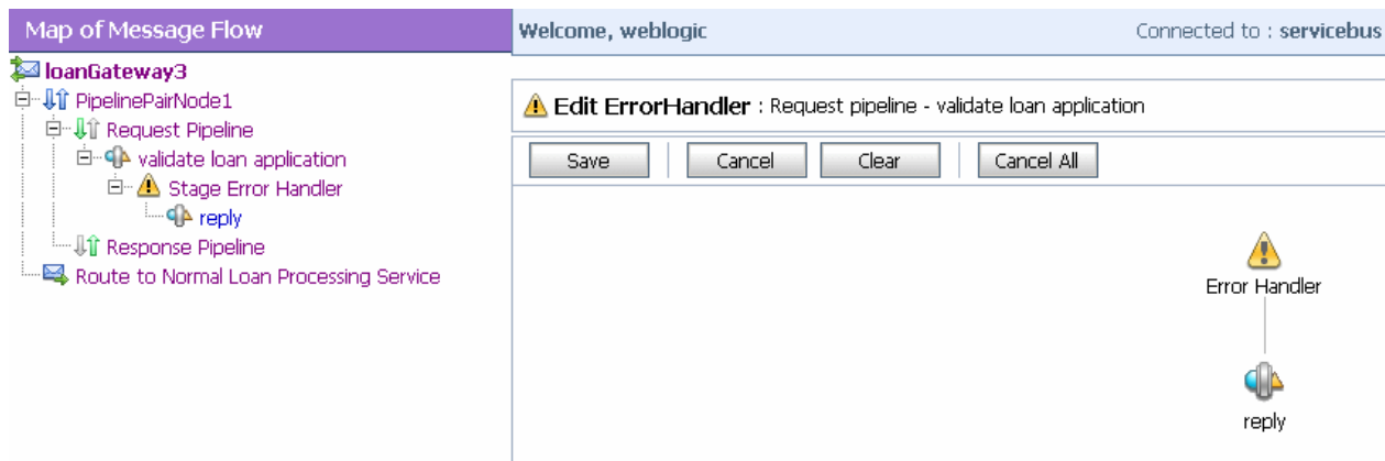
Figure 36–2 Error Handler Message Flow
