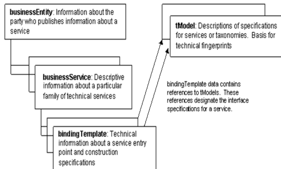
Figure 40–2 UDDI Entities Representing Organizations and Services
