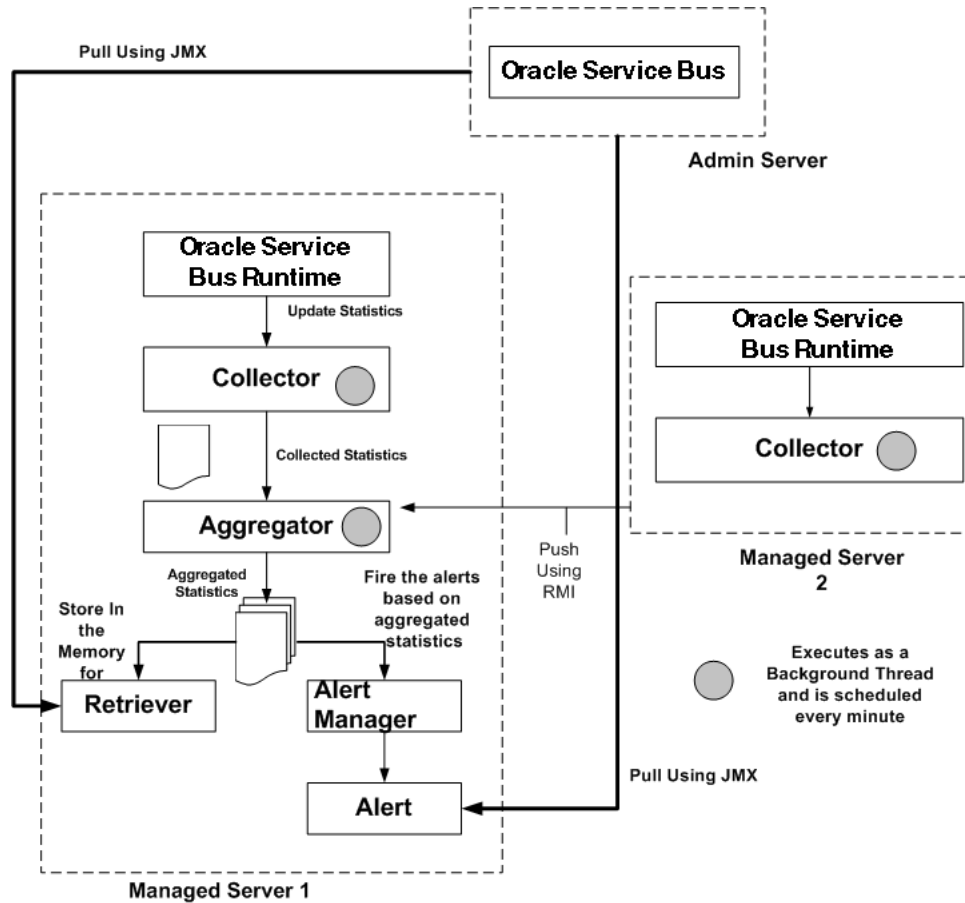
Figure 45–1 Monitoring Framework in Oracle Service Bus
