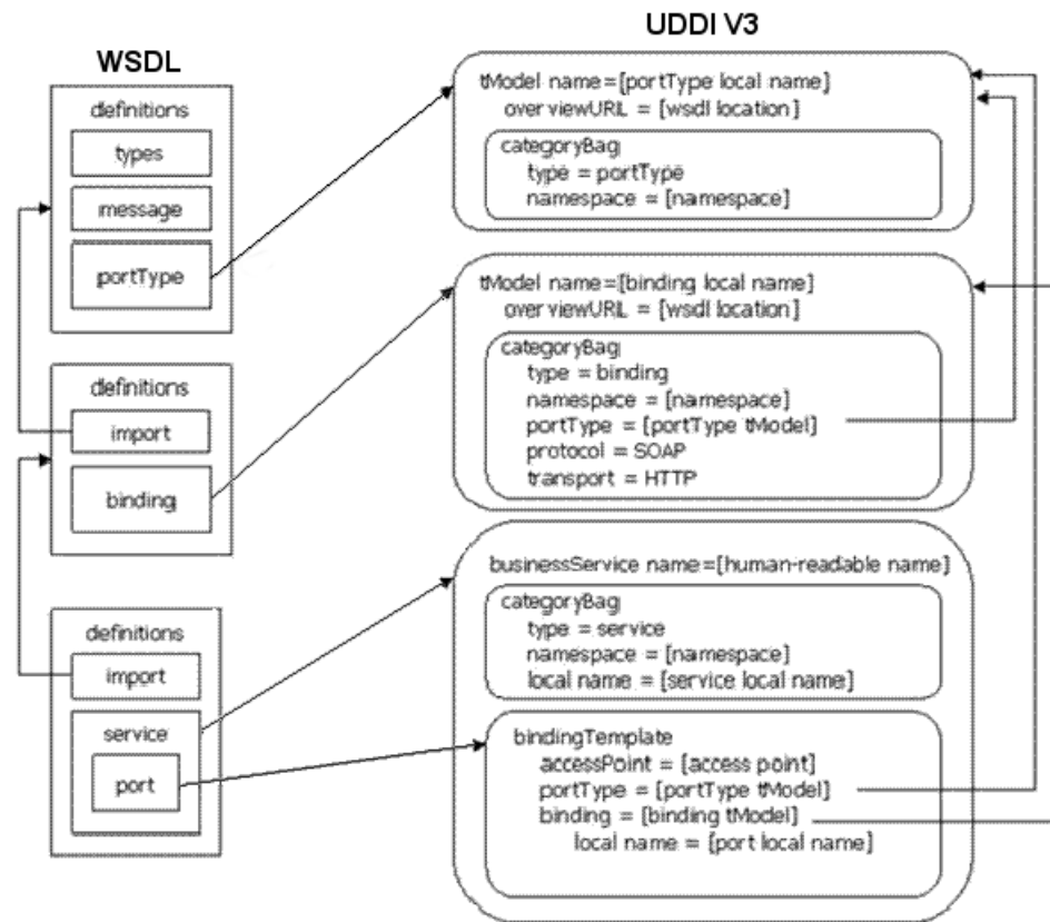
Figure 40–6 WSDL Service to UDDI Mapping
