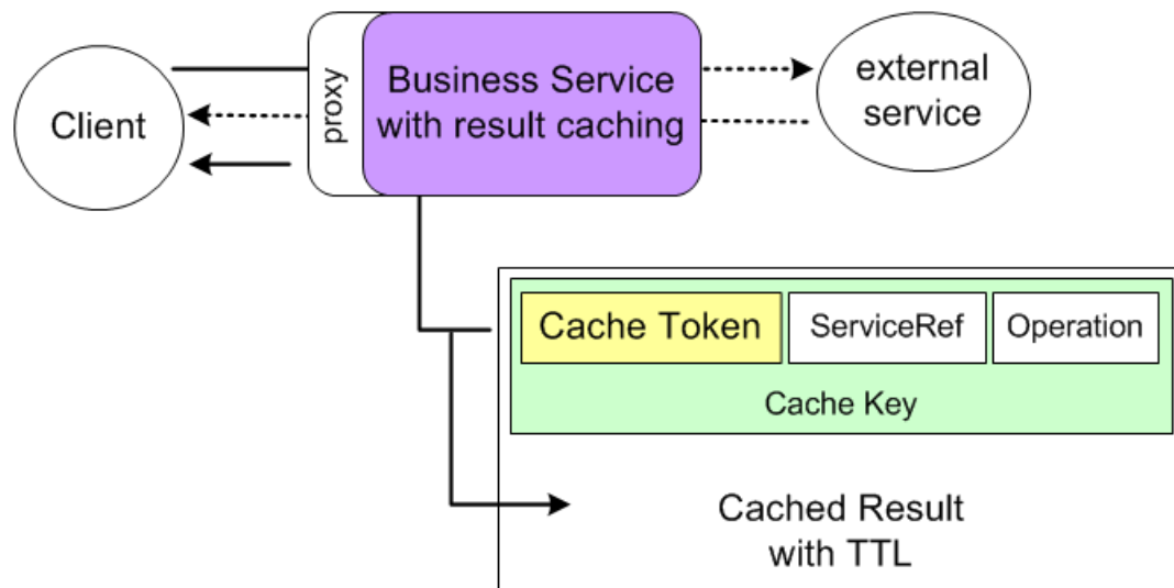
Figure 35–1 Business Service Result Caching
