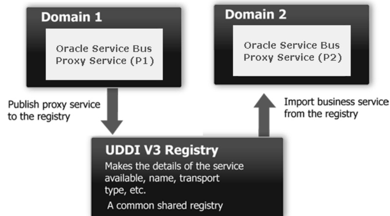
Figure 40–4 Sample Business Case of Cross-Domain Deployment
