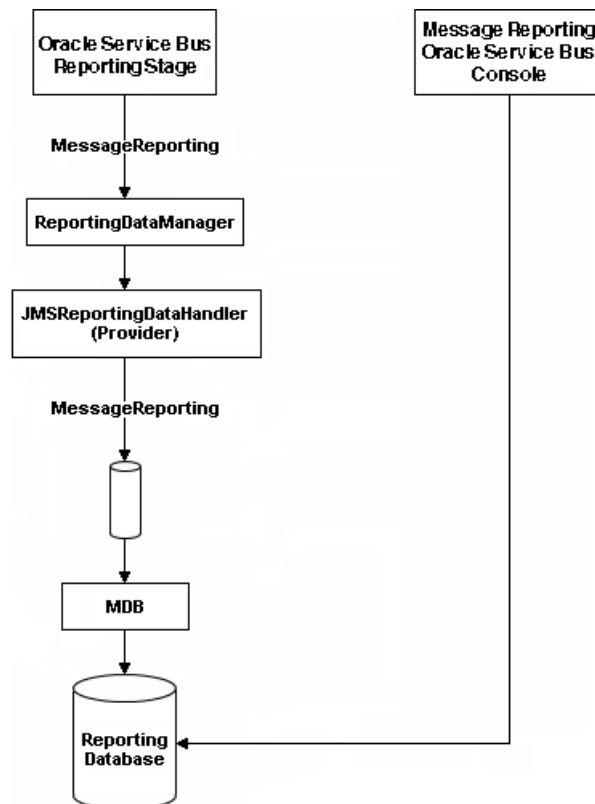
Figure 46-2 JMS Reporting Provider
