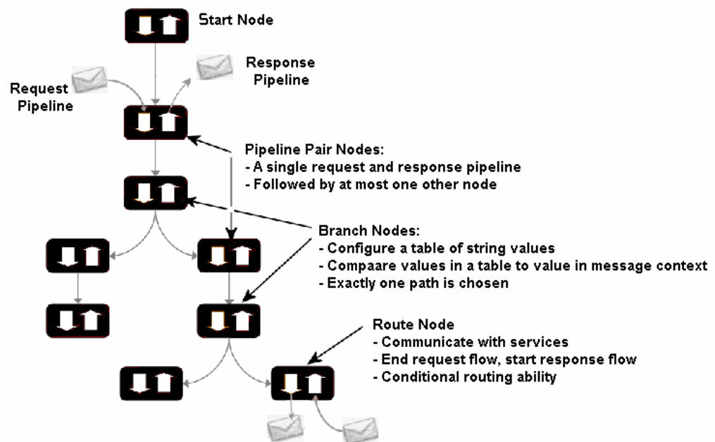
Figure 36–1 Components of Message Flow
