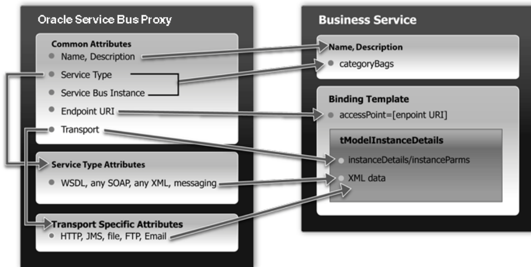
Figure 40–7 Oracle Service Bus to UDDI Mapping
