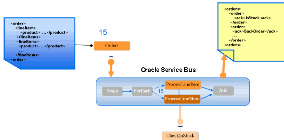
Figure 37-2 Dynamic Split-Join – Unknown number of service requests
