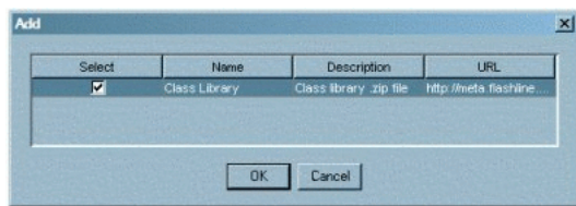
Figure 13–9 Add Dialog
