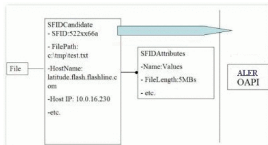
Figure 13–11 Object Model
