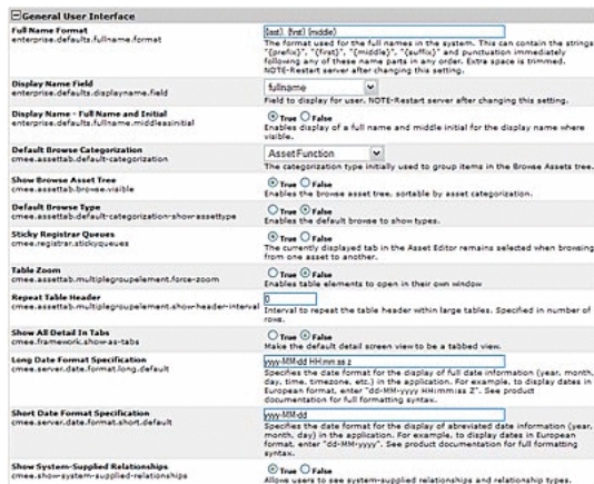
Figure 16–4 General User Interface
