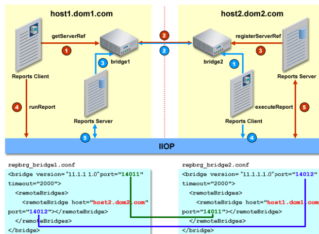
Figure 8–1 Oracle Reports Bridge Configuration (Two-Way)
