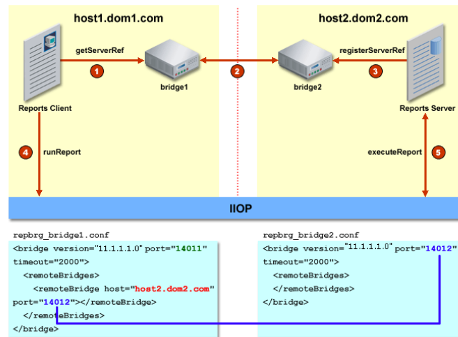
Figure 8–2 Oracle Reports Bridge Configuration (One-Way)
