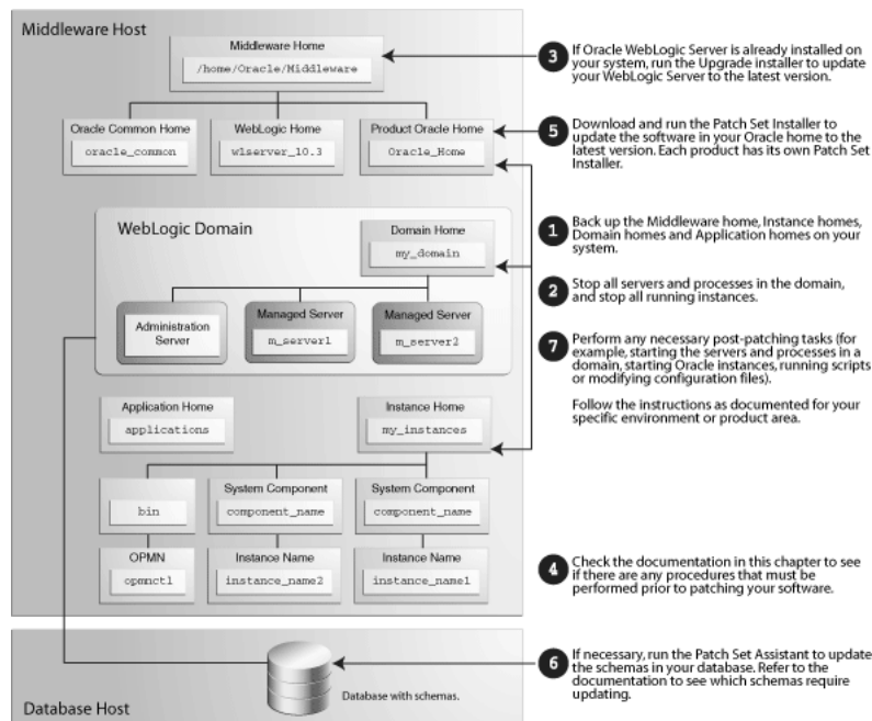
Figure 3–1 Patch Set Installer Procedural Overview and Roadmap
