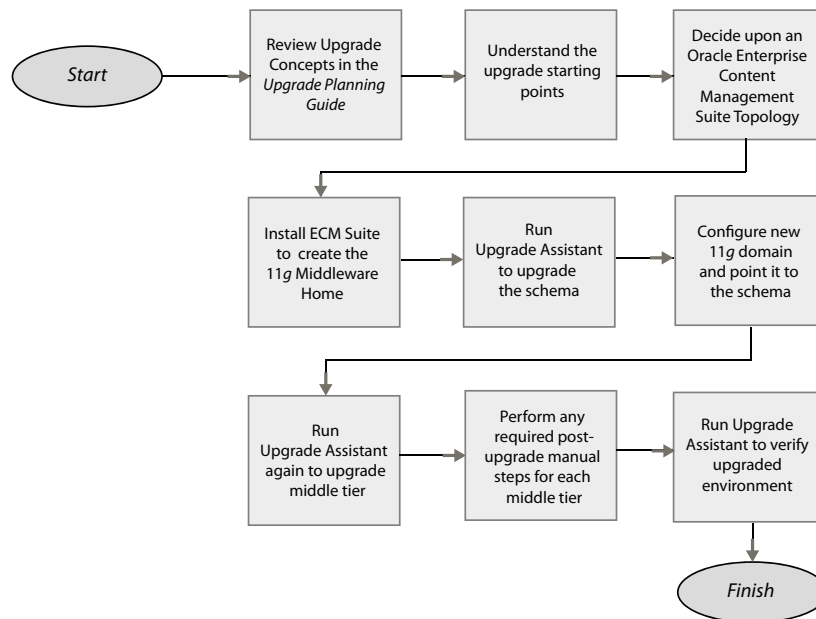
Figure 1–1 Flow Chart of the Oracle Enterprise Content Management Suite Upgrade Process
