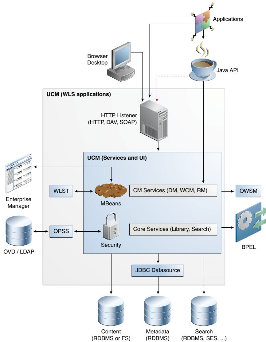
Figure 3–3 The Oracle UCM Architecture for Oracle Fusion Middleware 11g
