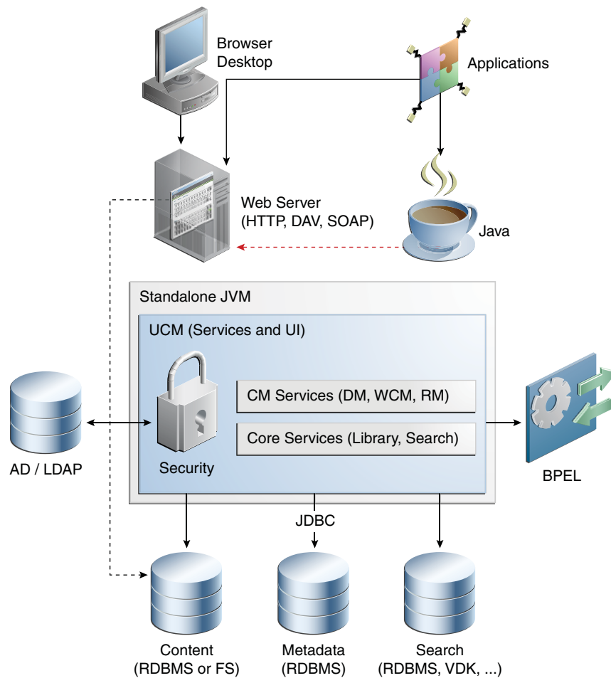
Figure 3–2 Comparing the Oracle Enterprise Content Management Suite Topology in 10g Release 2 (10.1.2) and Oracle Fusion Middleware 11g
