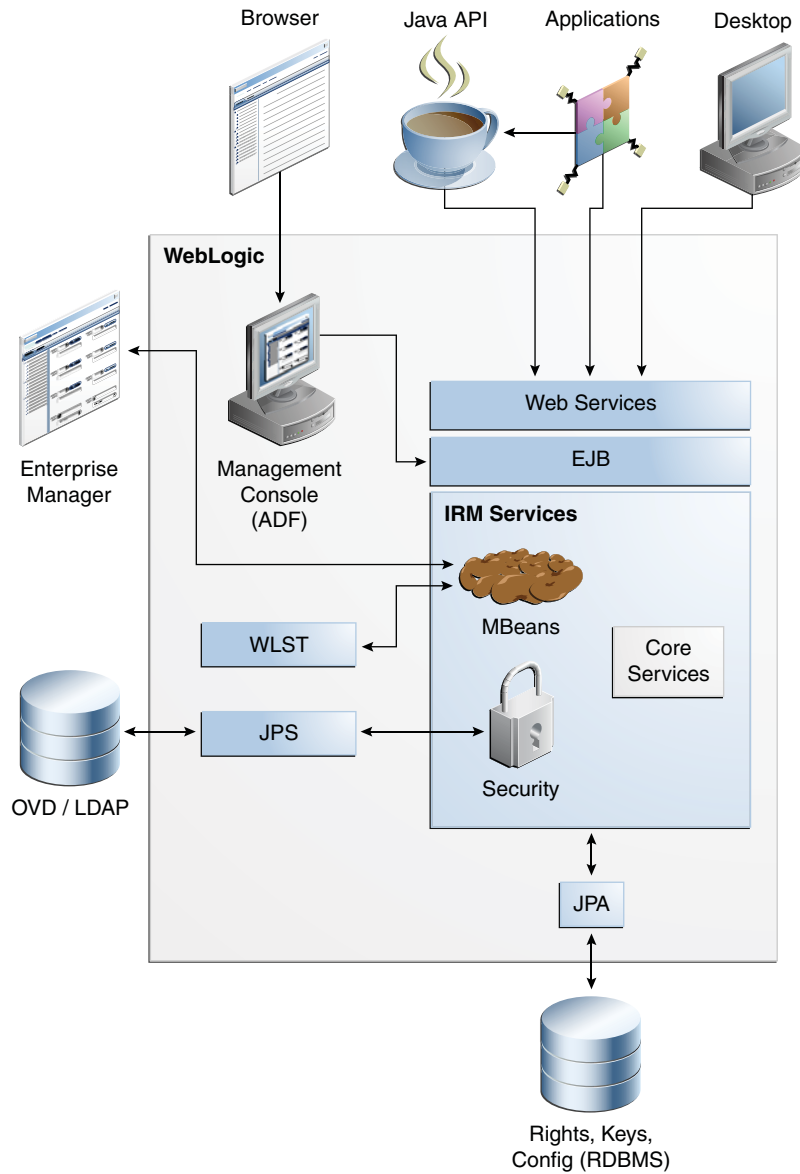
Figure 3–6 Oracle IRM Server 11g Running on Oracle WebLogic Server
