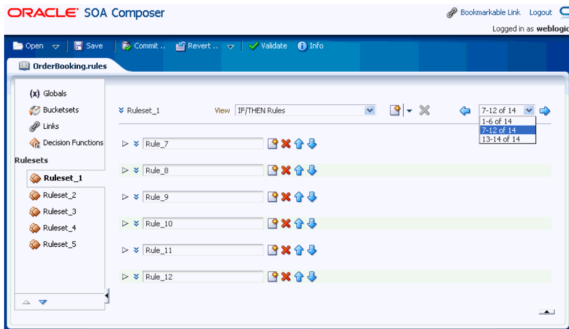
Figure 12–43 Rules Paging
