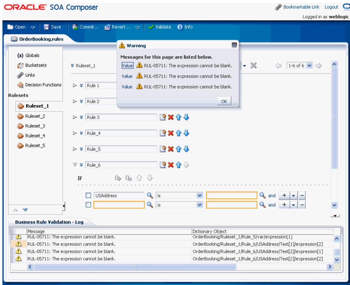
Figure 12–81 Rules Validation
