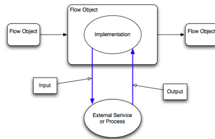
Figure 7-3 Relationship between a Flow Object, Implementation and an External Service or Process
