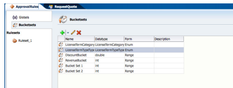
Figure 9–2 The Bucketsets Tab of the Oracle Business Rules Editor
