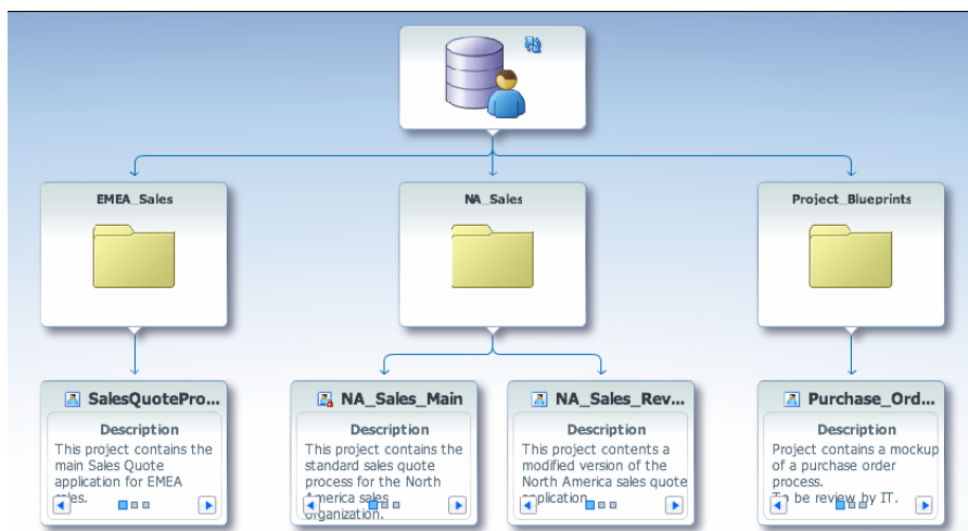
Figure 4–2 The Oracle BPM Metadata Service (MDS) Browser
