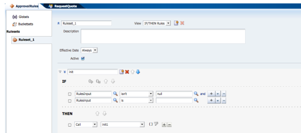
Figure 9–3 The Rulesets Tab of the Oracle Business Rules Editor
