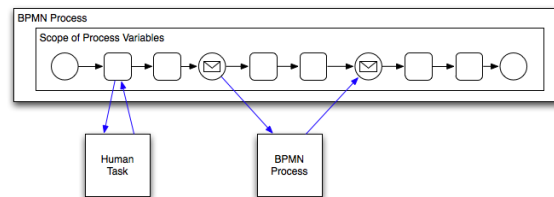
Figure 7-4 Data Associations between a process
