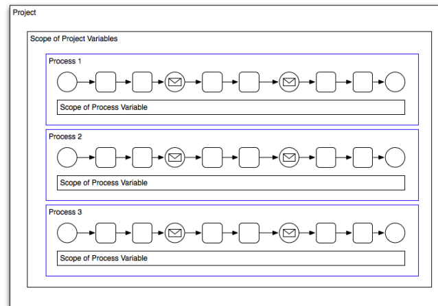
Figure 7–2 Scope of Process and Project Data Objects
