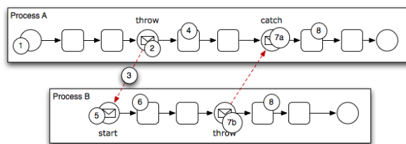
Figure 6–26 Using Message Throw and Catch Events Between Processes
