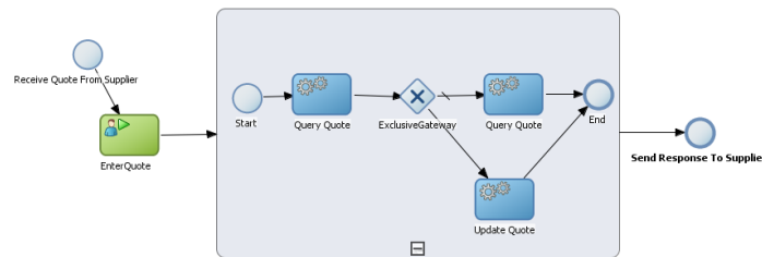
Figure 6–45 Example of a Subprocess
