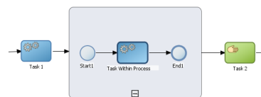
Figure 6-44 Example of an Expanded Subprocess
