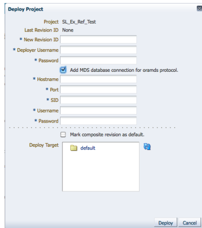
Figure 4–8 The Deploy Project Dialog
