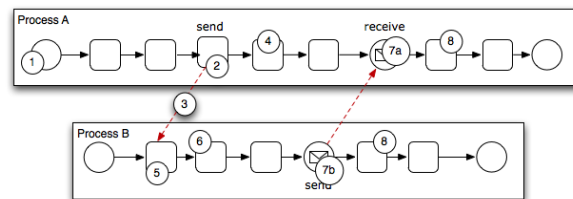
Figure 6–23 Using the Send and Receive Tasks to Communicate Between Processes
