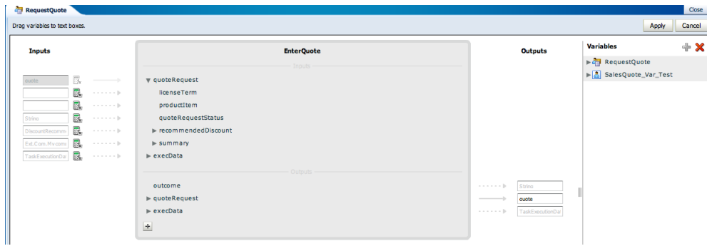
Figure 7-5 The Data Association Editor
