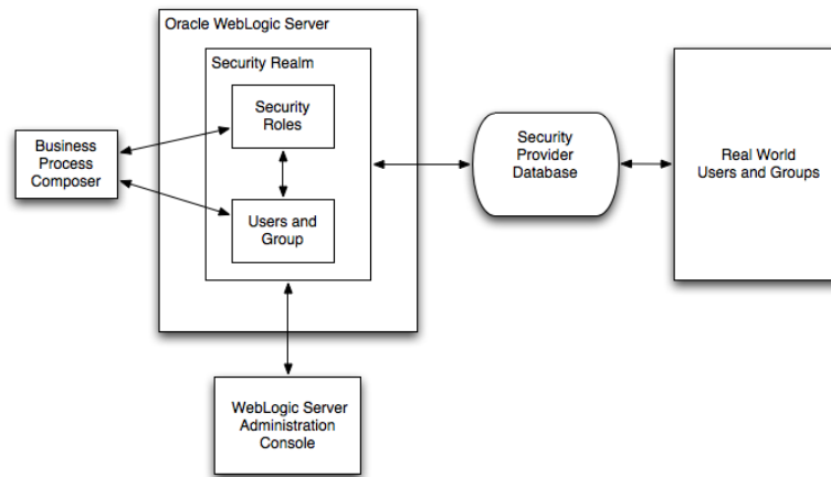
Figure 10–1 Oracle Business Process Composer Administration
