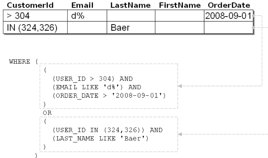
Figure 5–43 View Object Automatically Translates View Criteria Rows into Additional Runtime WHERE Filter
