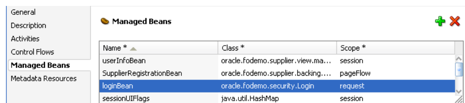
Figure 30–18 Login Bean Registered in adfc-config.xml File
