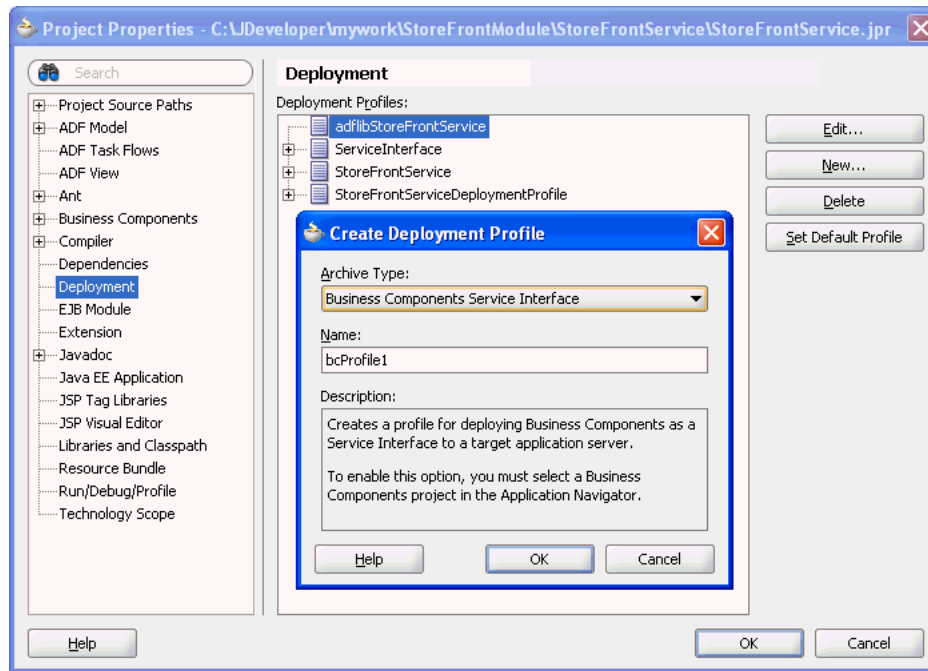
Figure 11–11 Dialog for Creating a Business Components Service Deployment Profile
