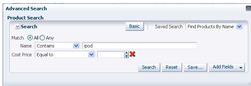
Figure 27–5 User-Added Search Criteria with Delete Icon
