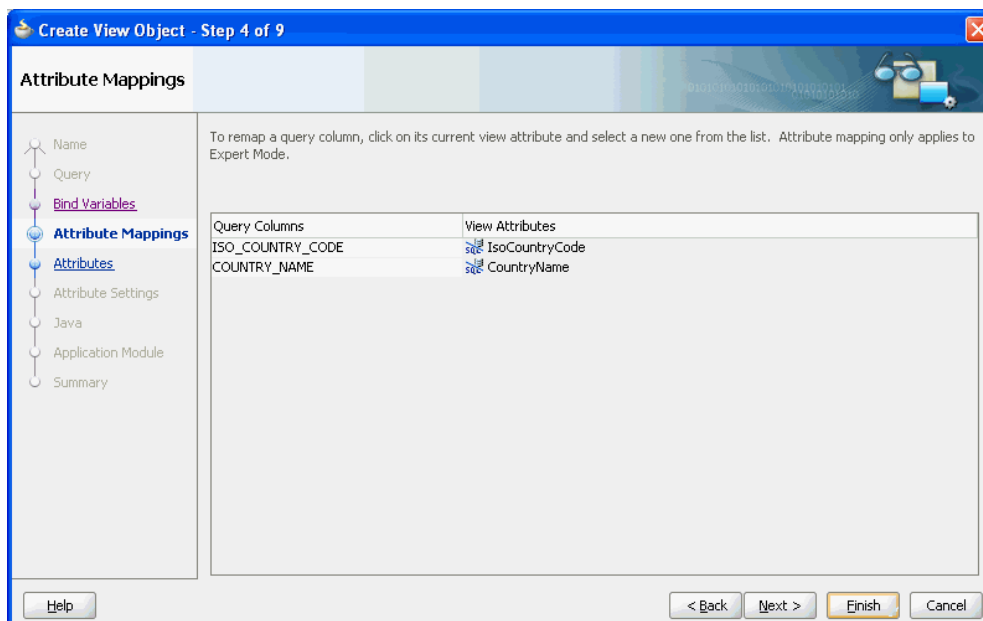
Figure 5–9 Create View Object Wizard, Attribute Mappings Page
