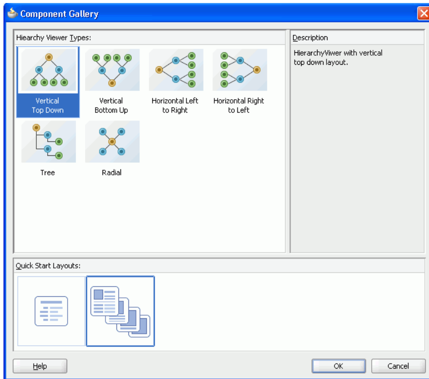
Figure 26–49 Component Gallery for Hierarchy Viewer Types
