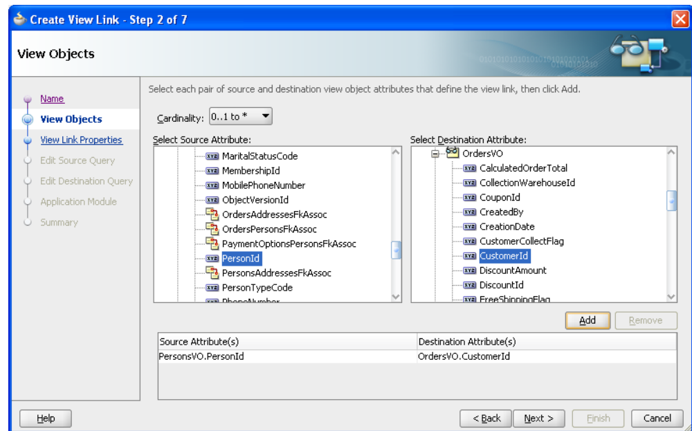
Figure 5–23 Defining Source/Target Attribute Pairs While Creating a View Link
