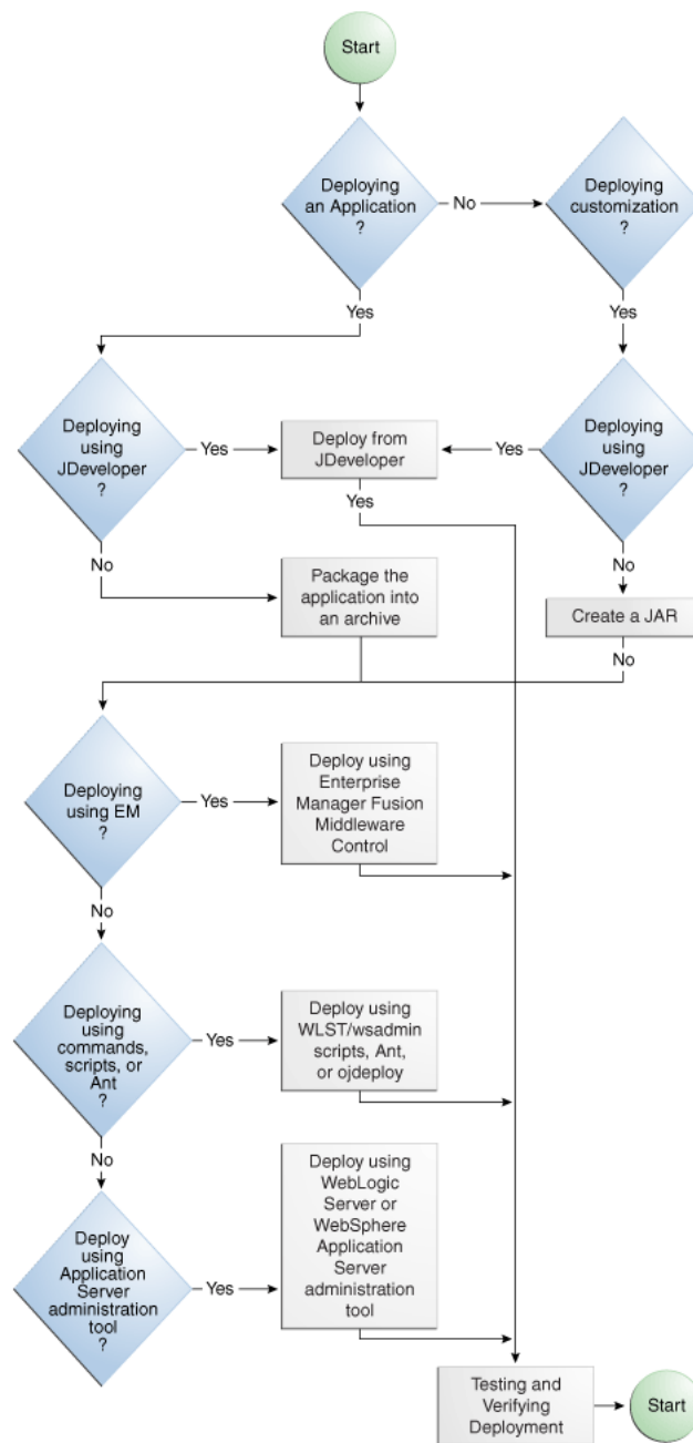
Figure 36–5 Application Deployment Flow Diagram
