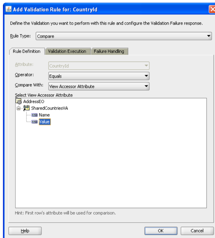
Figure 10–5 List Validator Using a View Accessor
