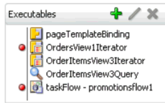
Figure 31–21 ADF Declarative Breakpoints Enabled in the Page Definition Executables
