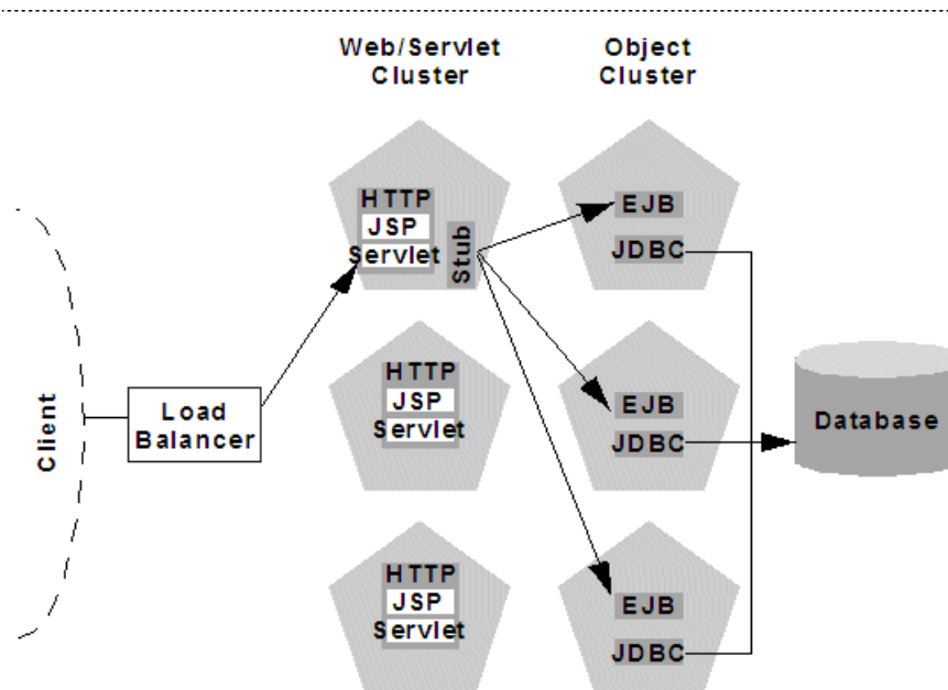
Figure 9-3 Load Balancing Objects in a Multi-Tier Architecture
