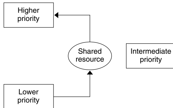
FIGURE 12-1 Unbounded Priority Inversion
