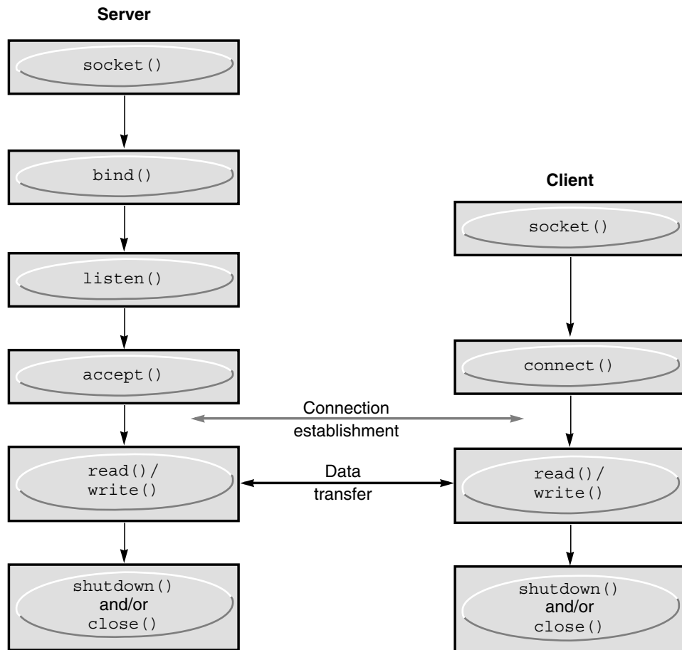
FIGURE 8-1 Connection-Oriented Communication Using Stream Sockets
