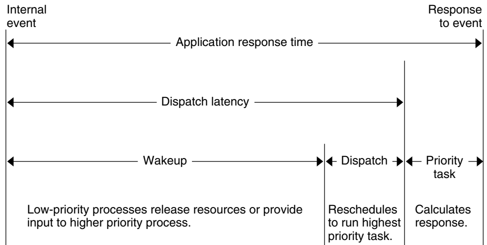
FIGURE 12-3 Internal Dispatch Latency
