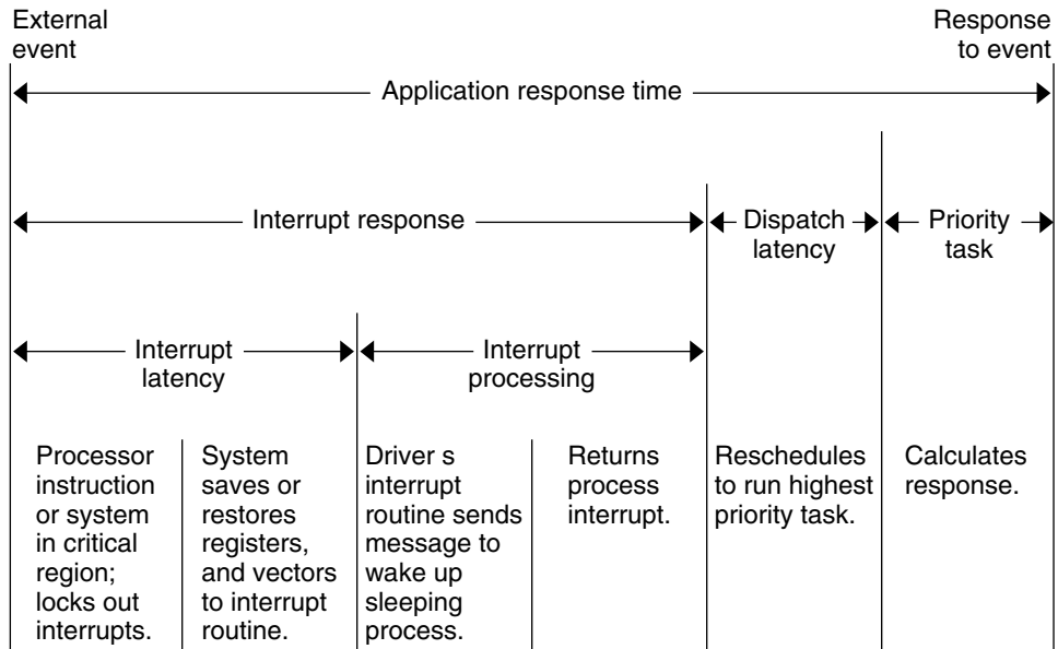
FIGURE 12-2 Application Response Time
