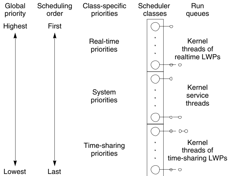
FIGURE 4-1 Process Priorities (Programmer's View)
