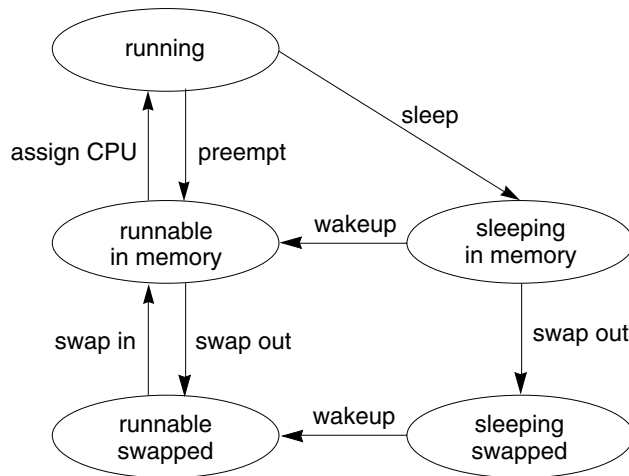
FIGURE 4-2 Process State Transition Diagram
