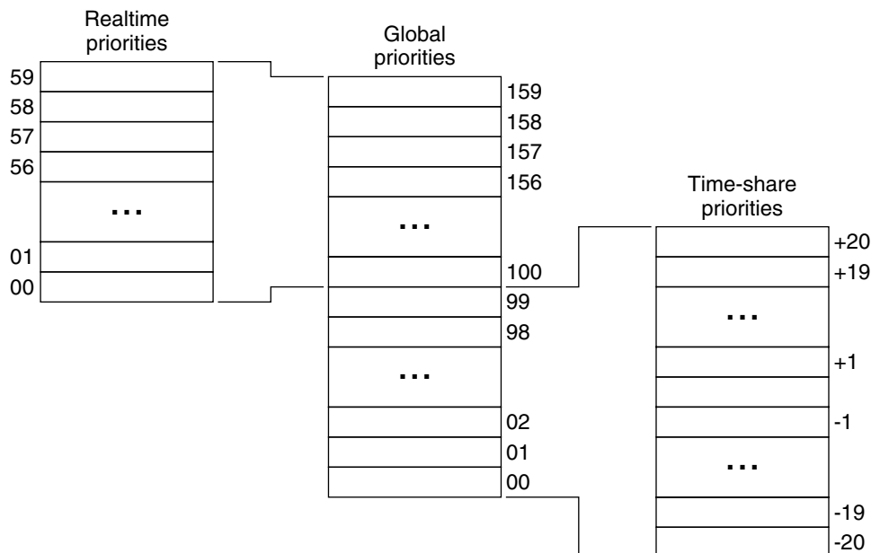
FIGURE 12-5 Kernel Dispatch Queue
