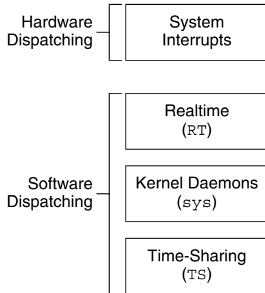
FIGURE 12-4 Dispatch Priorities for Scheduling Classes
