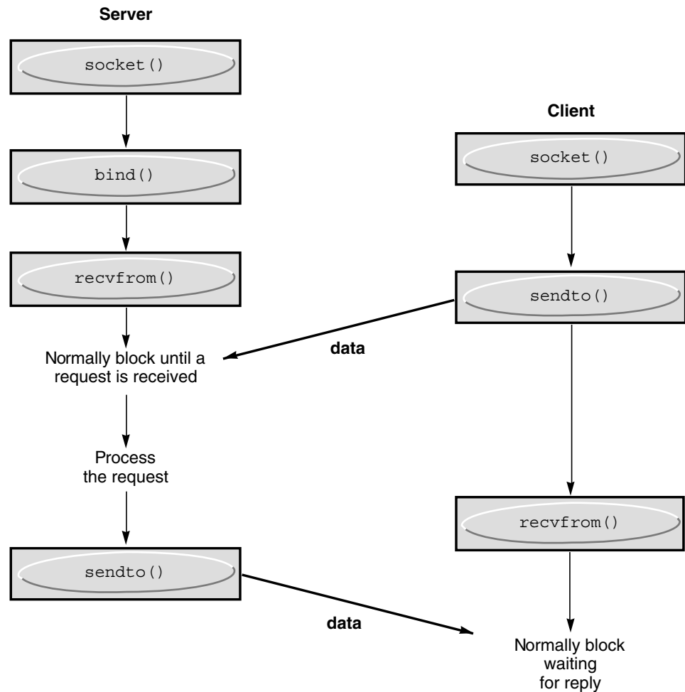
FIGURE 8-2 Connectionless Communication Using Datagram Sockets
