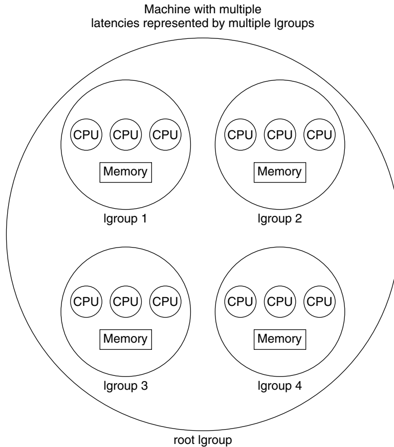
FIGURE 5-2 Multiple Locality Groups Schematic
