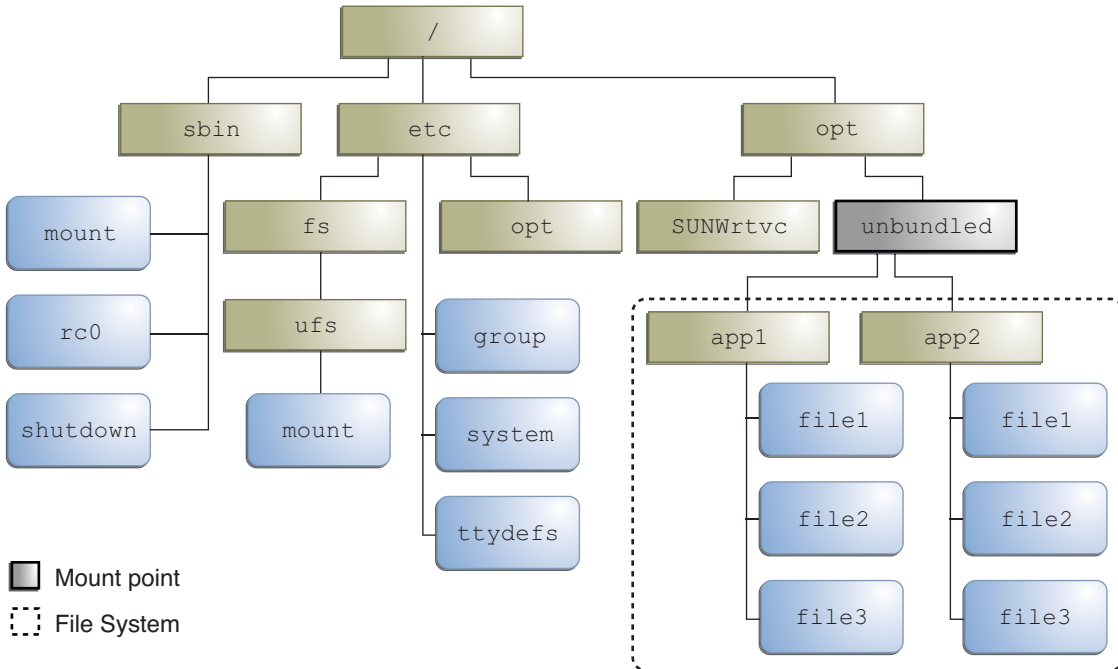
FIGURE 16-2 Mounting a UFS File System
