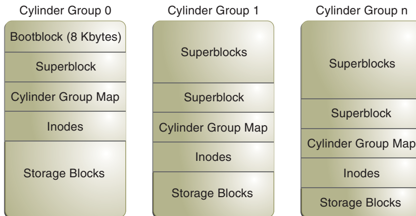
FIGURE 21-2 A Typical UFS File System
