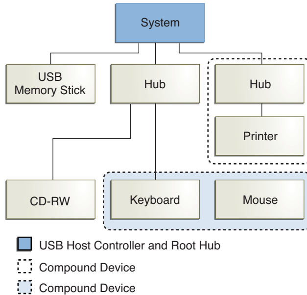
FIGURE 7-1 USB Physical Device Hierarchy
