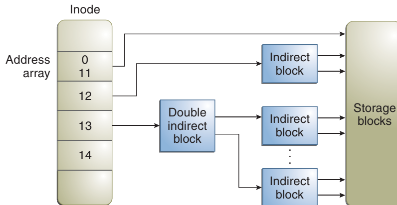
FIGURE 21-1 Address Chain for a UFS File System
