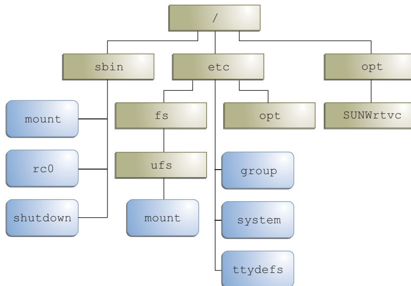
FIGURE 16-1 Sample UFS root (/) File System
