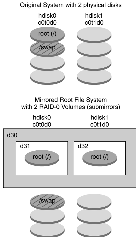
FIGURE 9-1 Creating RAID-1 Volumes on the Root (/) File System on Two Disks
