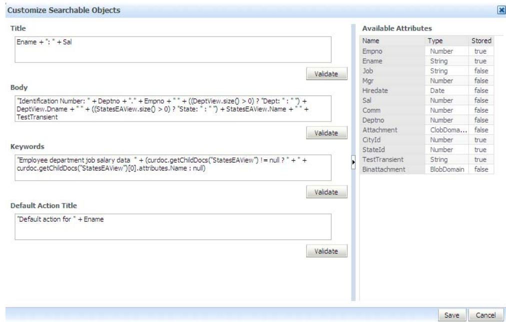
Figure 7–12 Customize Searchable Objects Dialog
