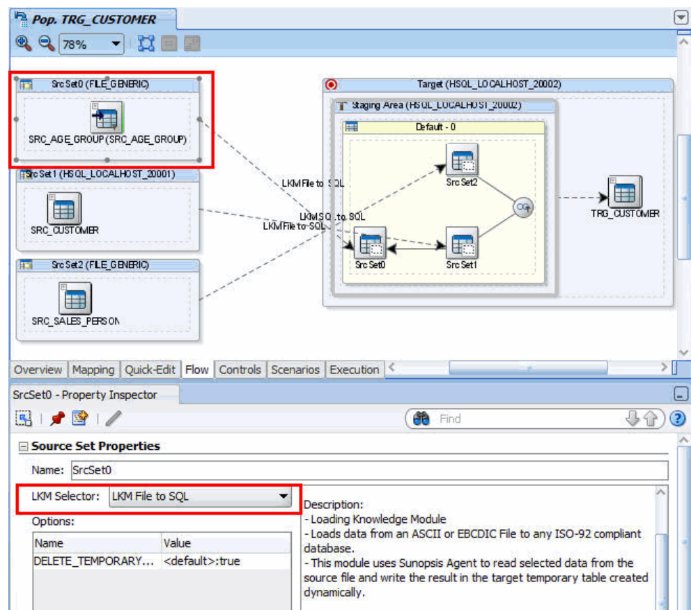
Figure 6–19 Flow tab of the Pop. TRG_CUSTOMER Interface Editor
