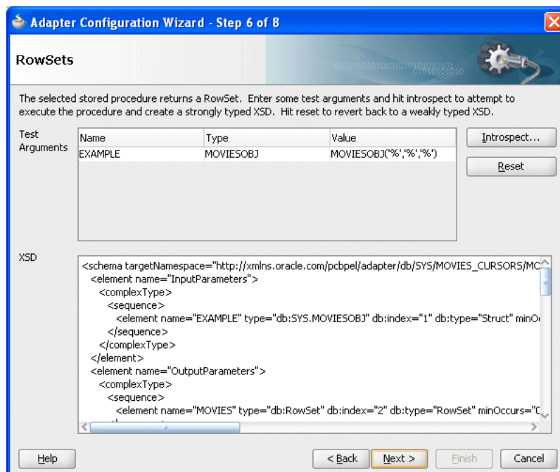
Figure 9–50 RowSets Page
