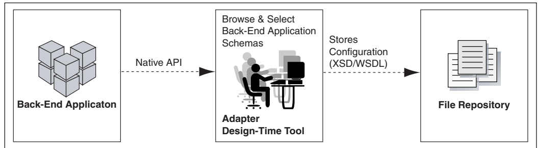
Figure 1–18 Metadata Service
