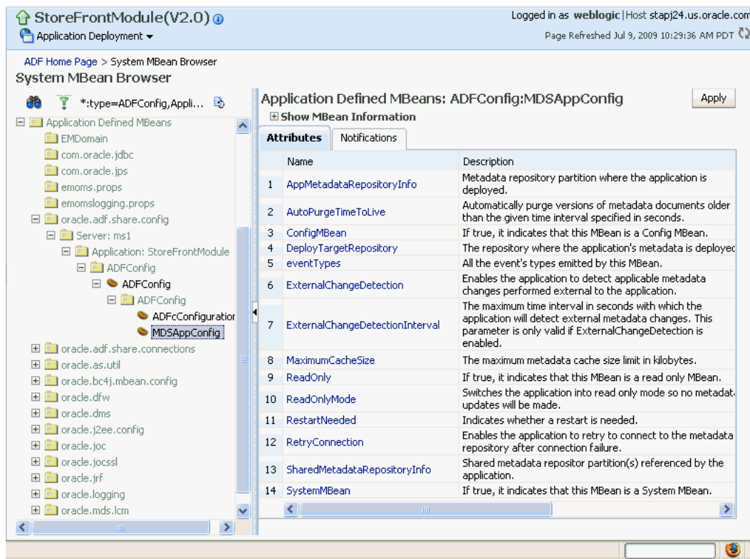
Figure 3–3 MDS MBean
