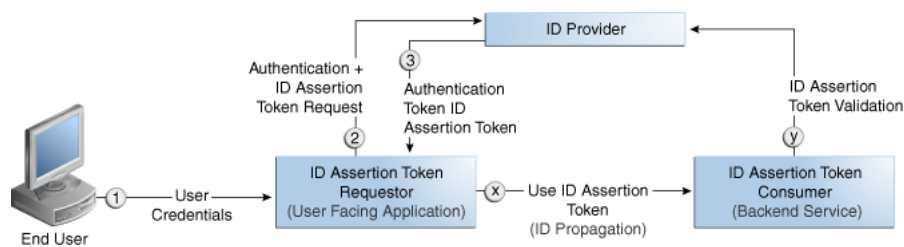
Figure 16–3 Process Flow During Identity Propagation
