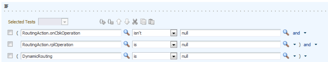
Figure 26–8 Nested Rules Support
