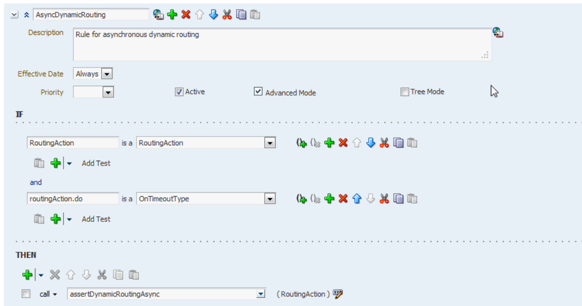
Figure 26–11 Advanced Mode Features
