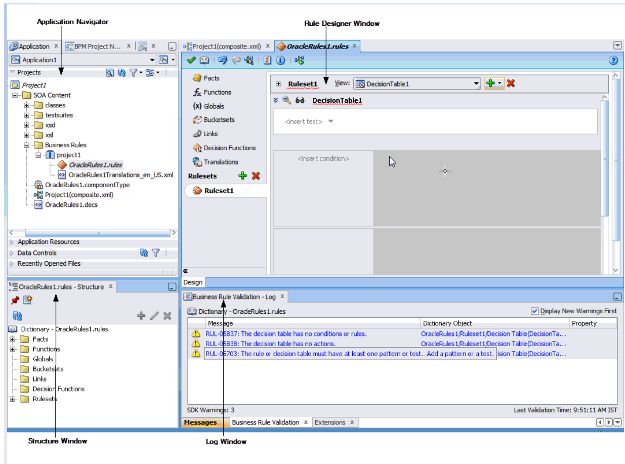
Figure 25–1 Rules Designer in Oracle JDeveloper
