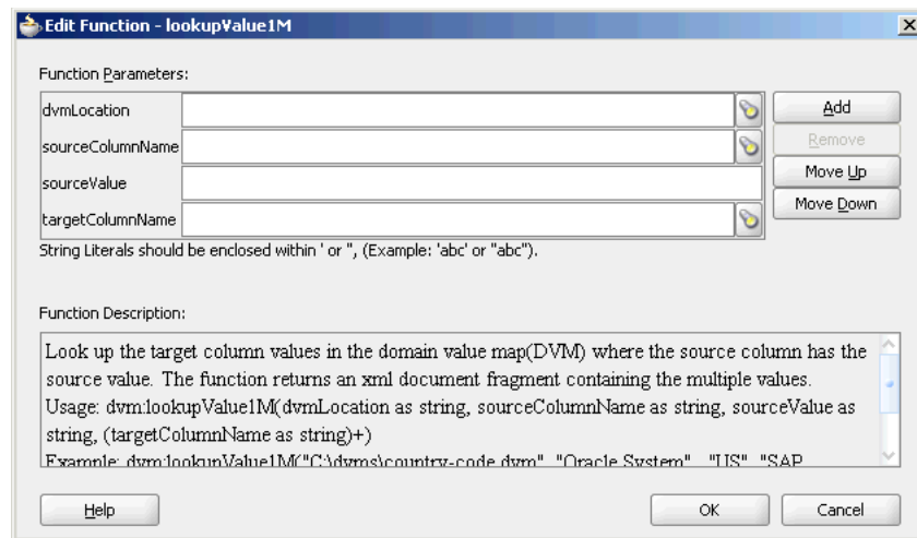
Figure 47–8 Edit Function – lookupValue1M Dialog
