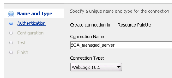
Figure 64–17 New Application Server Connection
