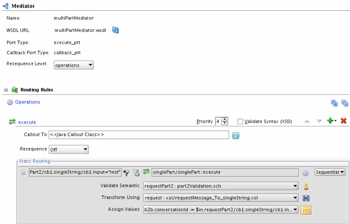
Figure 21–1 Mediator Editor for a Multipart Source
