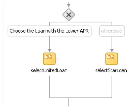
Figure A–40 Switch Activity
