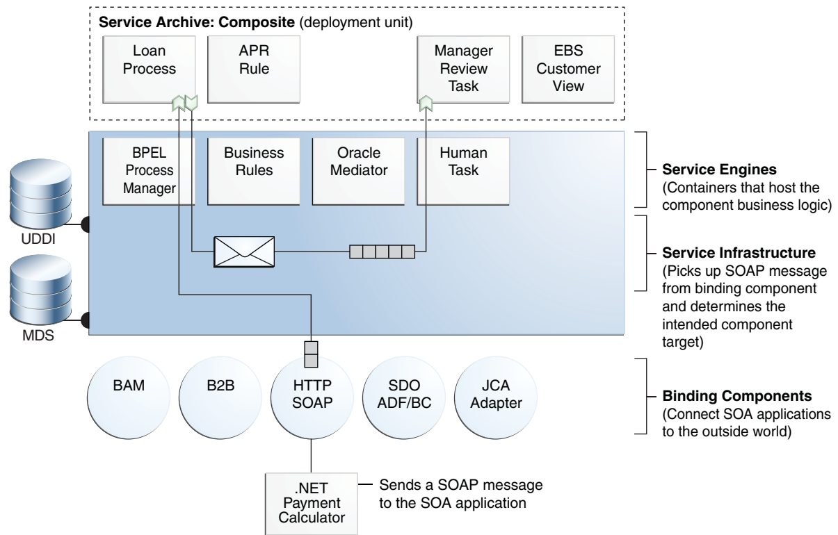
Figure 1–2 Runtime Behavior of SOA Composite Application
