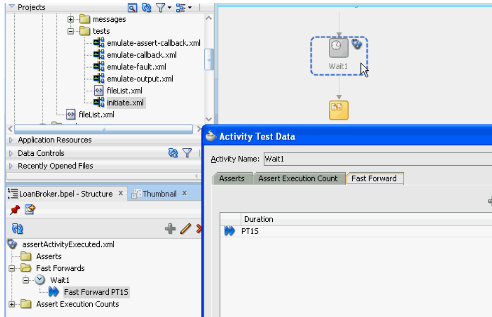
Figure 44–25 Fast Forwards Folder in Structure Window
