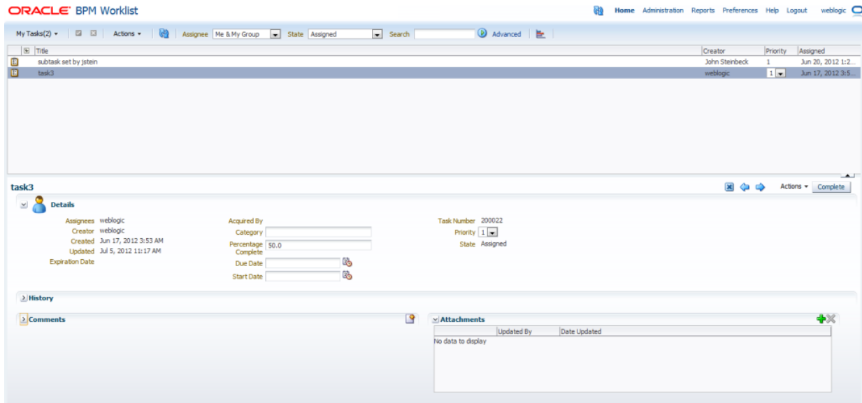
Figure 32–2 Oracle BPM Worklist—The Home (Task List) Page
