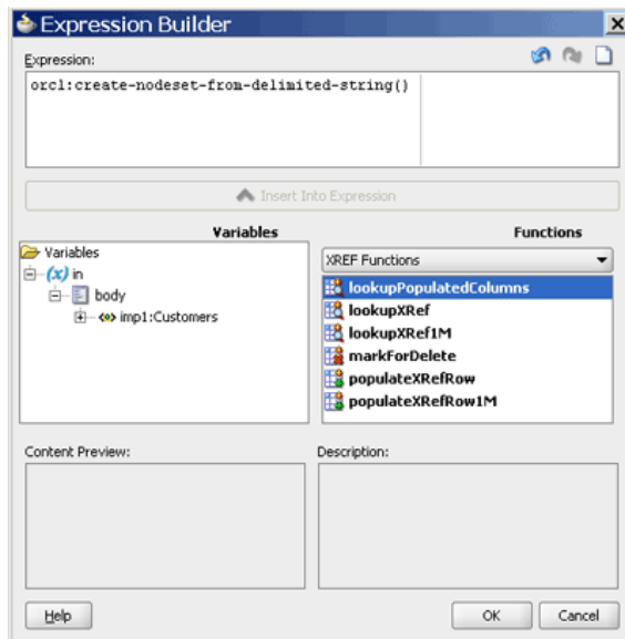
Figure 49-6 Expression Builder Dialog with Cross Reference Functions
