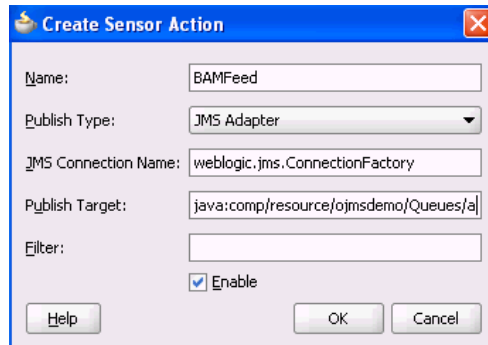
Figure 18–11 Using the JMS Adapter Publish Type
