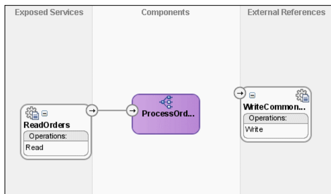
Figure 47-14 WriteCommonOrder Reference in the SOA Composite Editor
