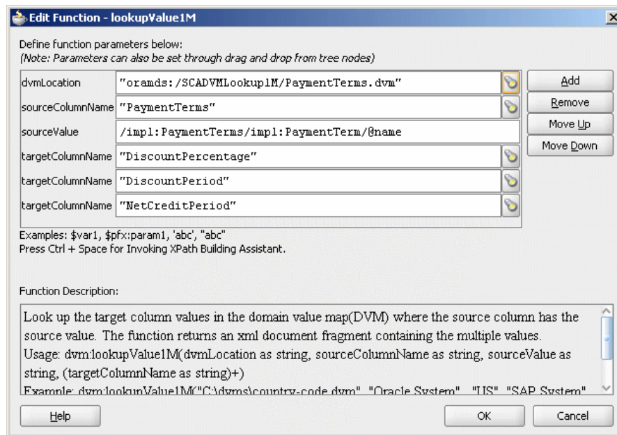
Figure 47–9 Populated Edit Function – lookupValue1M Dialog
