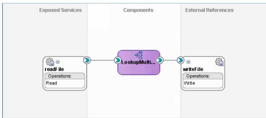
Figure 47–24 LookupMultipleValuesMediator Mediator Connected to the writeFile Reference
