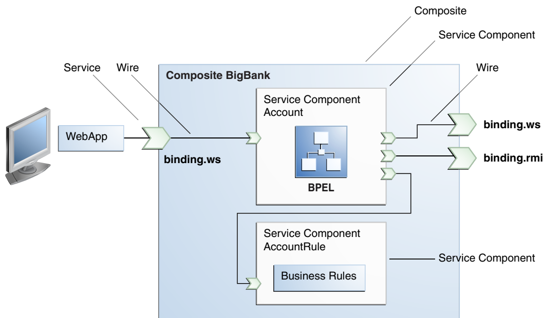
Figure 1-1 Simple SOA Composite Architecture
