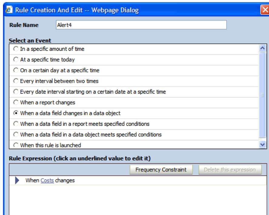
Figure 60–7 Rule Creation and Edit Dialog
