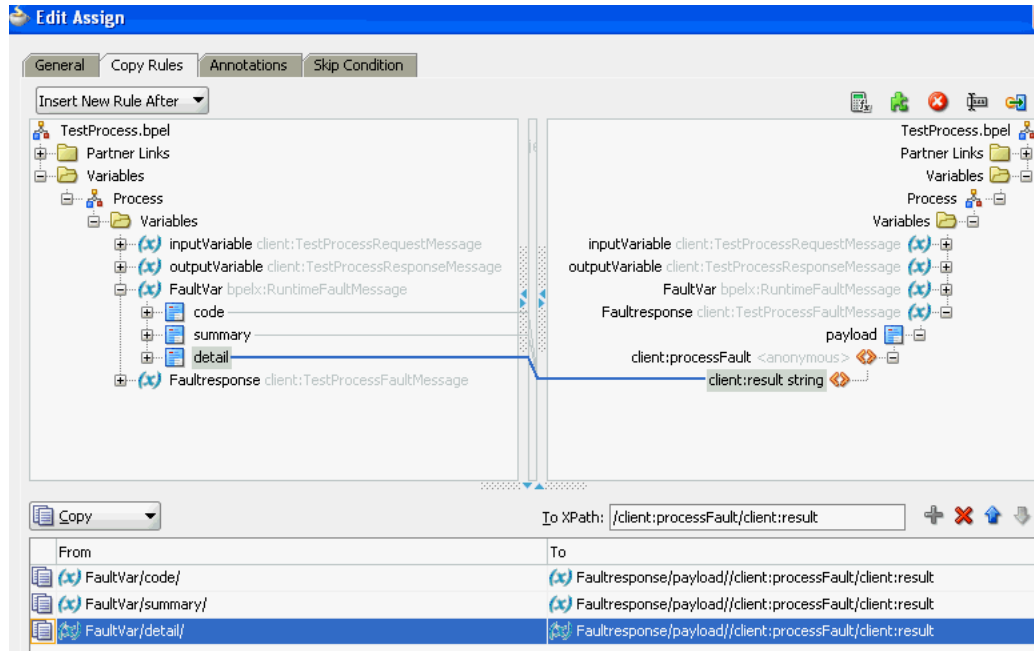
Figure 12–7 Edit Assign Dialog
