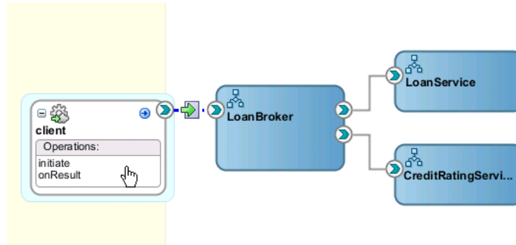
Figure 44-7 Service Binding Component Access
