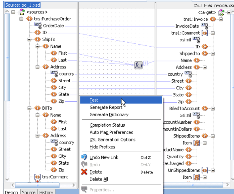
Figure 40–48 Invoking the Test Dialog
