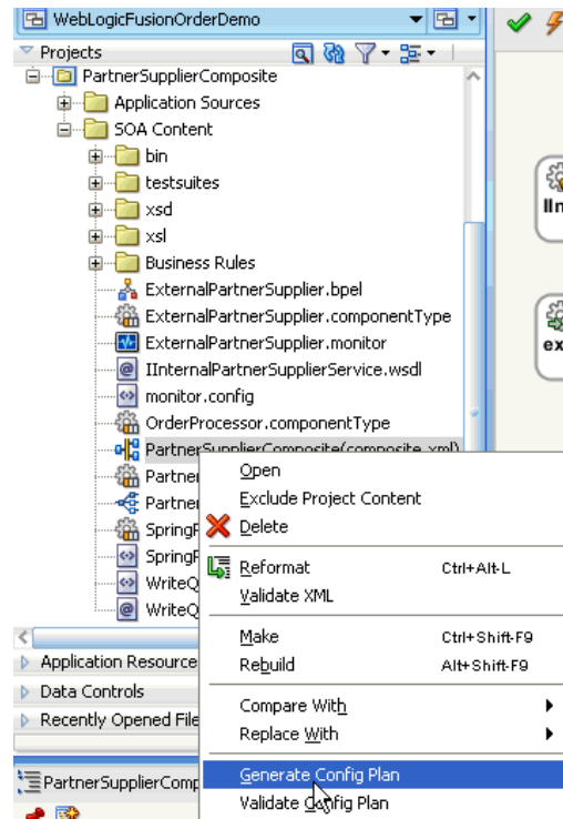
Figure 43–1 Generate a Configuration Plan
