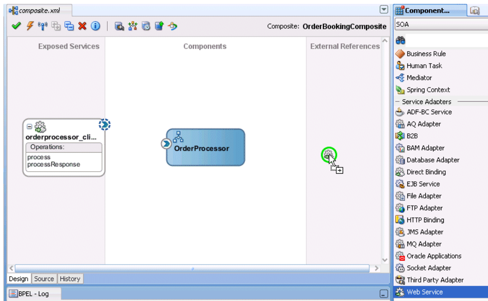
Figure 2–14 Adding Web Service to Composite
