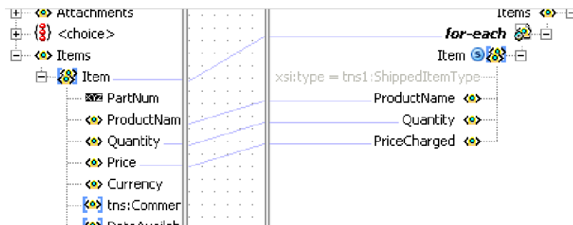
Figure 40–53 Item Elements in XSLT Mapper
