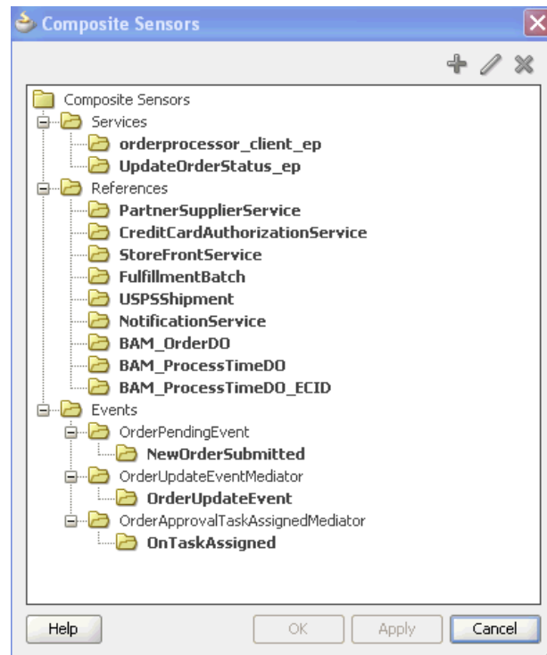
Figure 50–4 Composite Sensors Dialog
