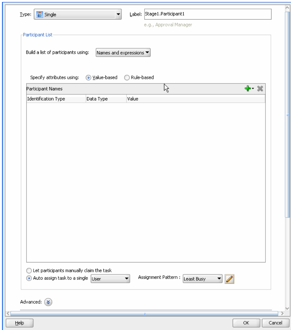
Figure 29–22 Edit Participant Type — Single Type
