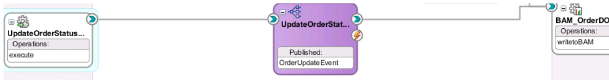
Figure 37–1 Service and Reference Binding Components
