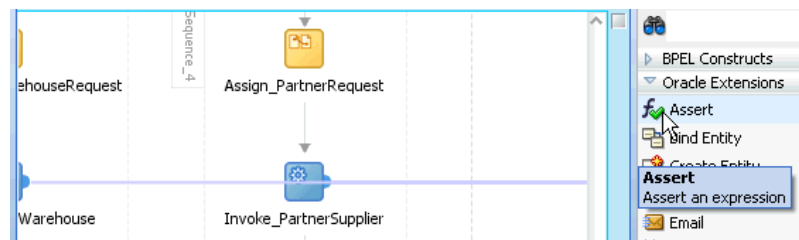
Figure 12–34 Assert Activity in Component Palette
