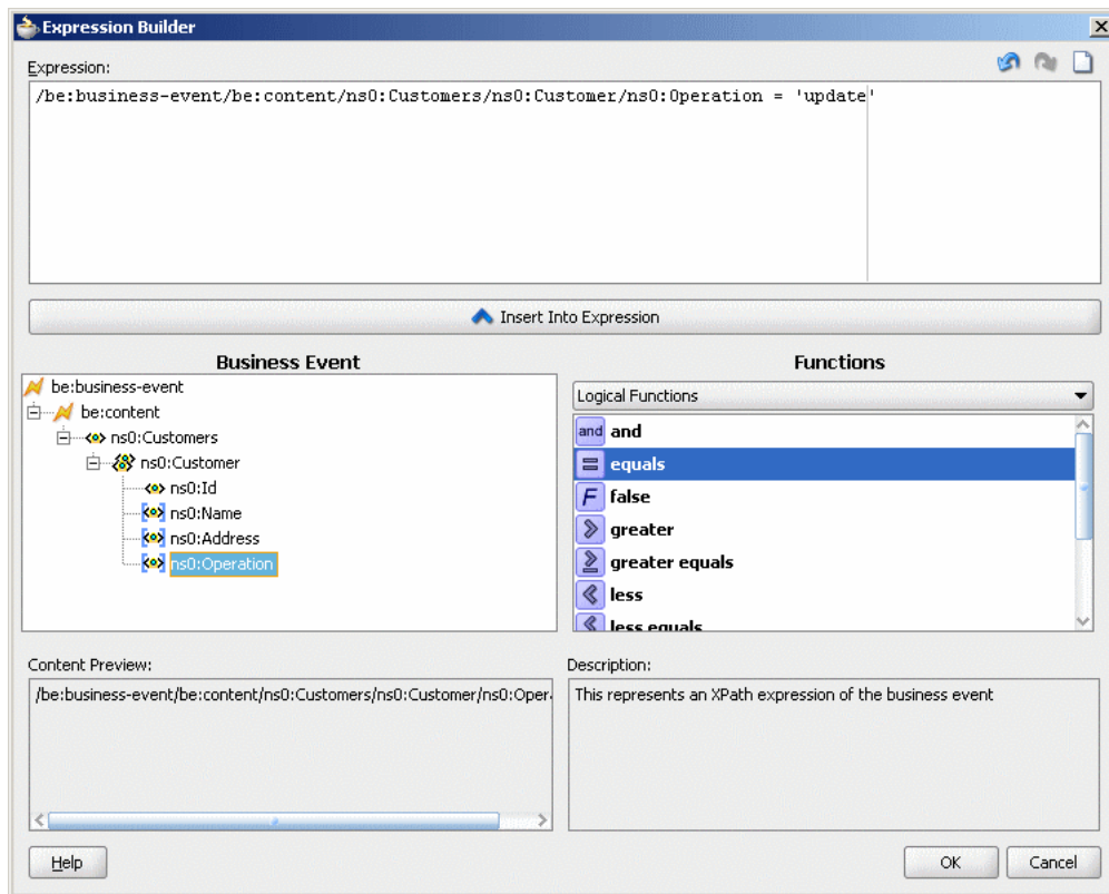
Figure 19–11 Business Event Filter
