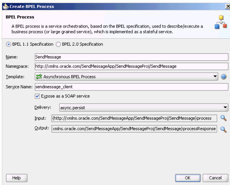
Figure J-4 Creating the BPEL Process
