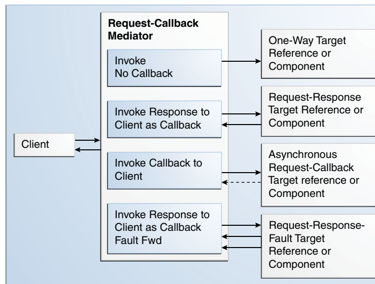
Figure 24–4 Request-Callback Message Exchange Pattern
