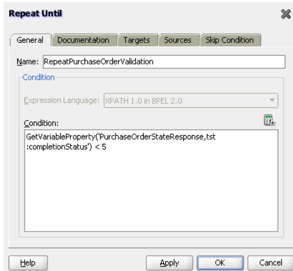
Figure A-30 Repeat Until Dialog
