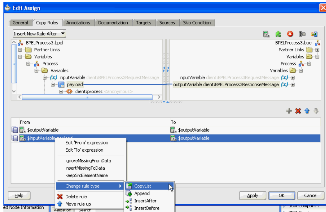
Figure A-5 Copy Rule Converted to bpelx Extension in BPEL 2.0
