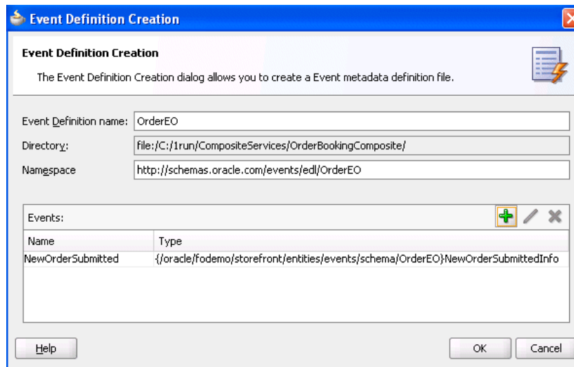
Figure 41–4 Event Definition Creation Dialog
