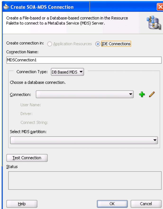
Figure 43–23 Create SOA-MDS Connection Dialog
