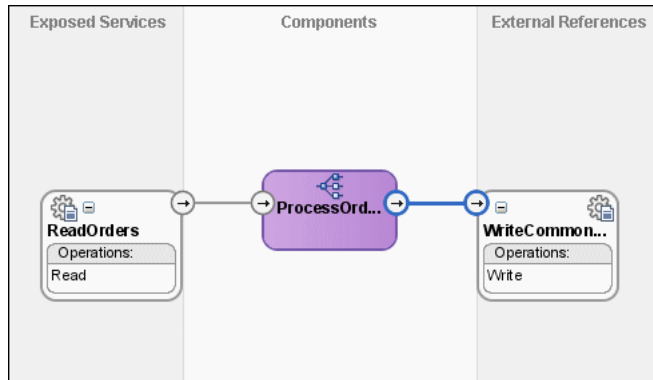
Figure 47-15 ProcessOrders Mediator Connected to the WriteCommonOrder Reference
