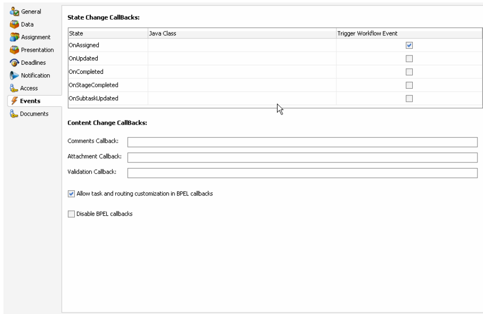
Figure 29–66 Callback Details Dialog with Java Selected
