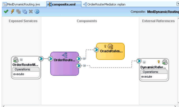
Figure 20–33 SOA Composite Editor with Wire Links Between the Business Rule and Mediator Service Components
