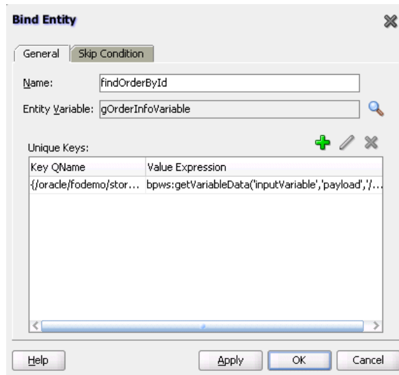
Figure A-7 Bind Entity Dialog
