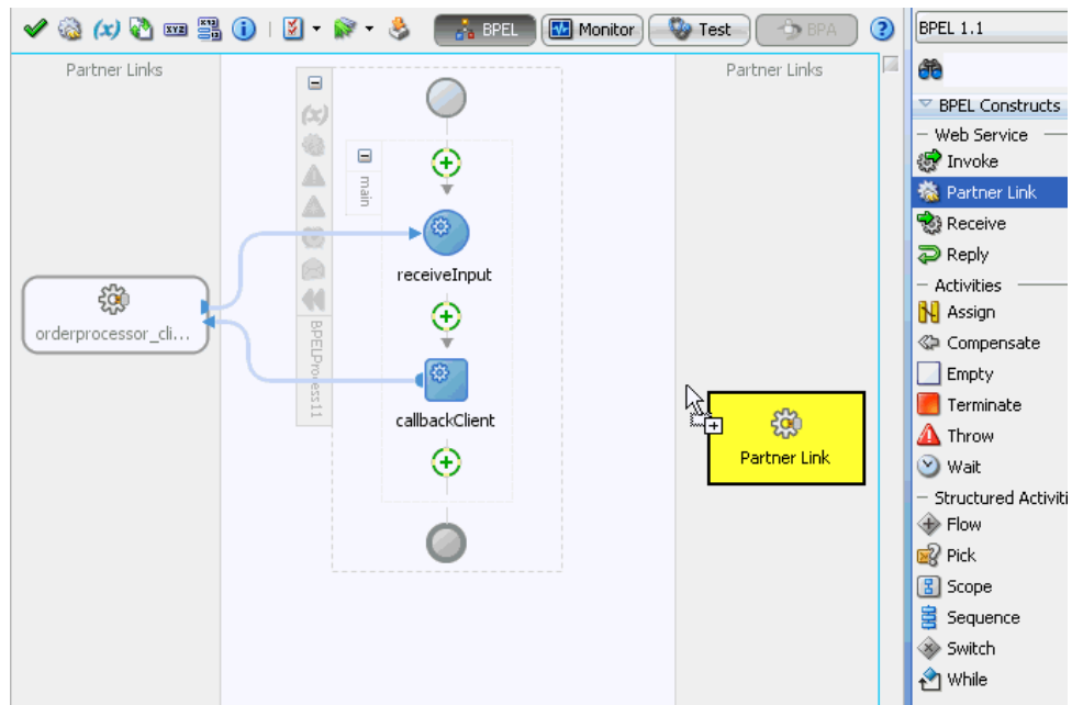
Figure 4–10 Partner Link Creation in Oracle BPEL Designer
