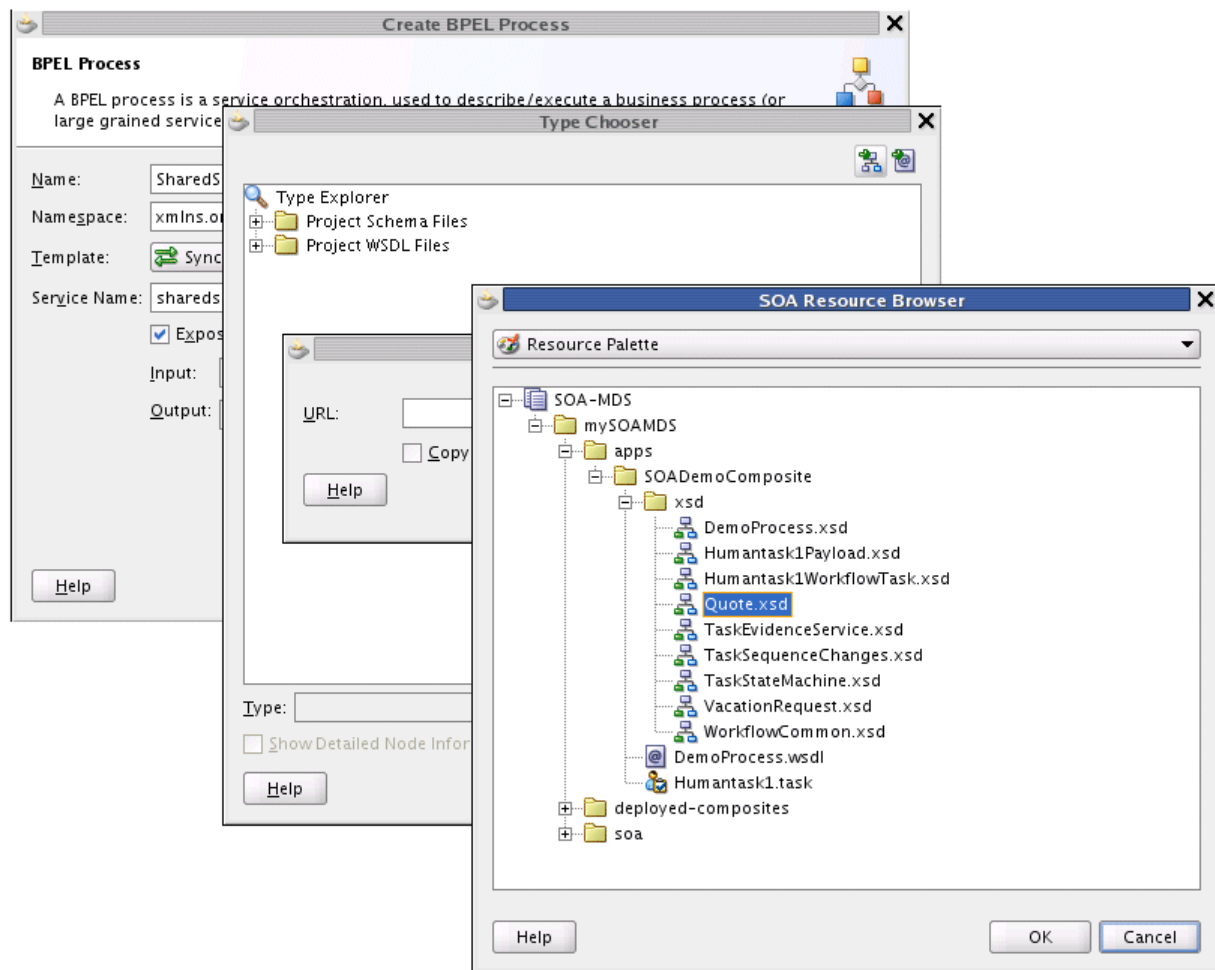
Figure 43–24 Shared Data in the SOA Resource Browser
