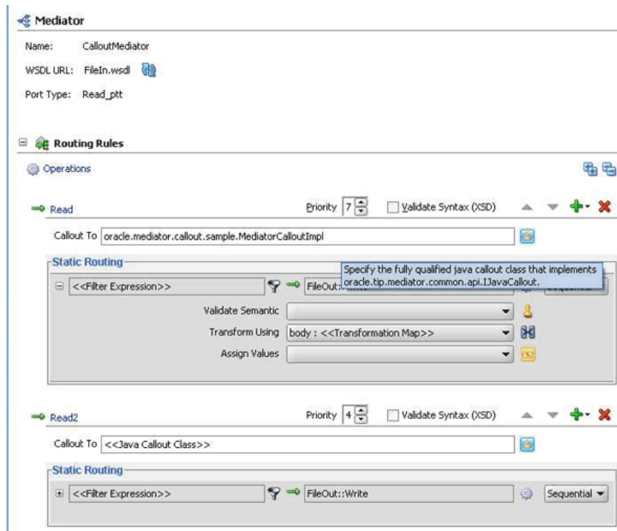
Figure 20–27 Sample Mediator Supporting Java Callout
