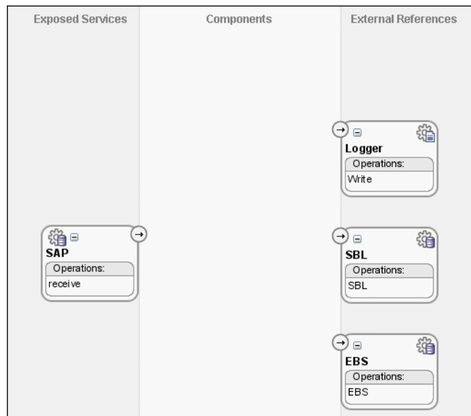
Figure 49–22 Logger Reference in SOA Composite Editor
