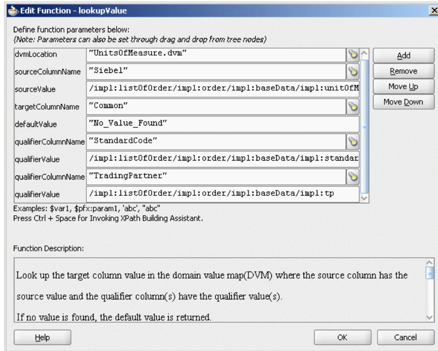
Figure 47-18 Edit Function-lookupValue Function Dialog: Hierarchical Lookup Use Case
