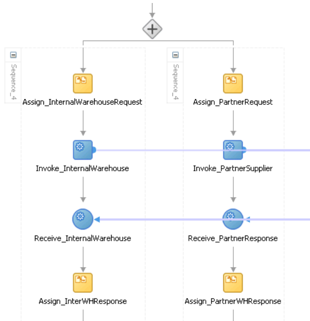
Figure A-16 Flow Dialog (After Design Completion)
