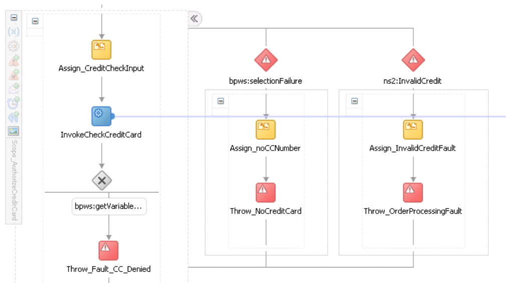
Figure 12–16 Scope Activity After Design Completion
