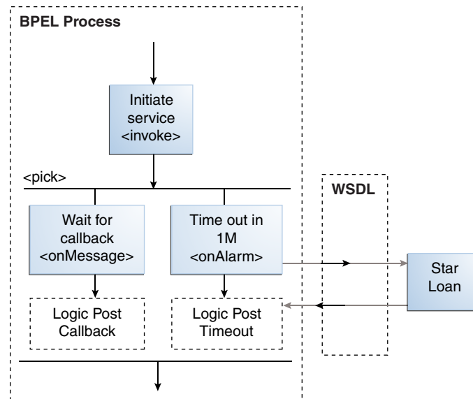
Figure 15–1 Overview of the Pick Activity
