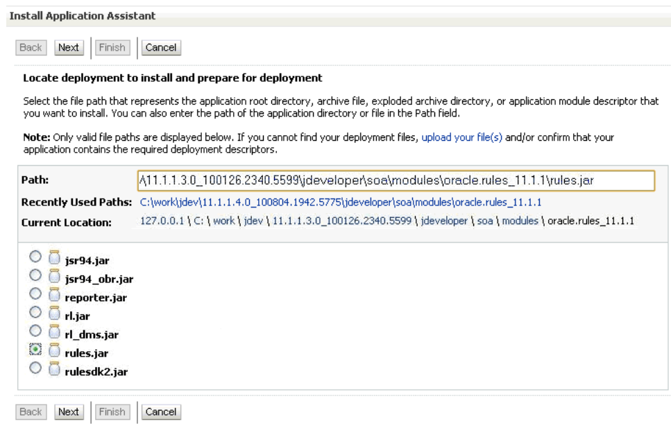
Figure 26–24 Deploying the oracle.rules Shared Library
