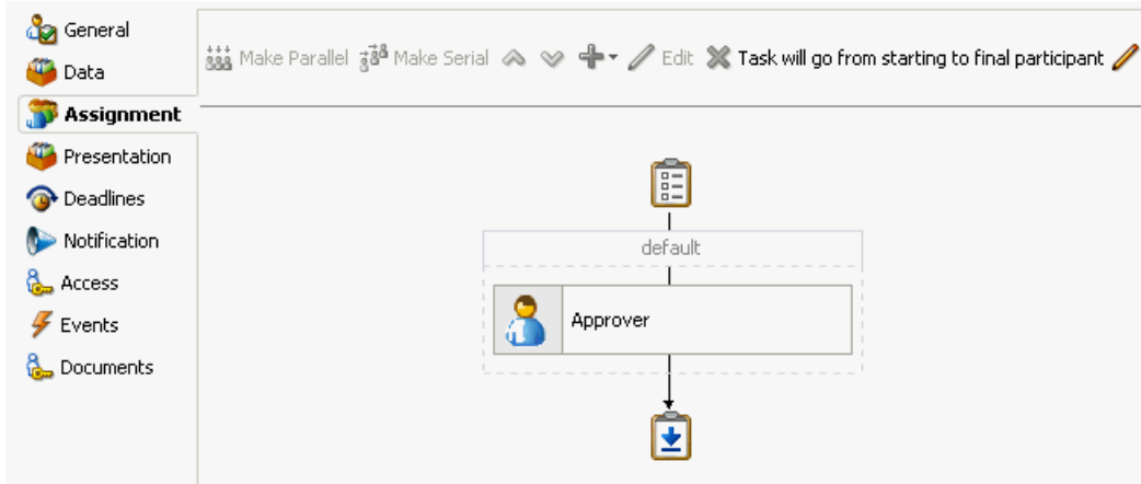
Figure 29–40 Human Task Editor — Assignment Section
