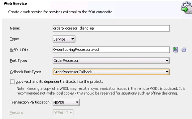
Figure 2–6 Create Web Service Dialog
