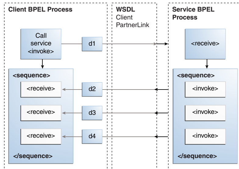
Figure 5–6 One Request, Multiple Responses
