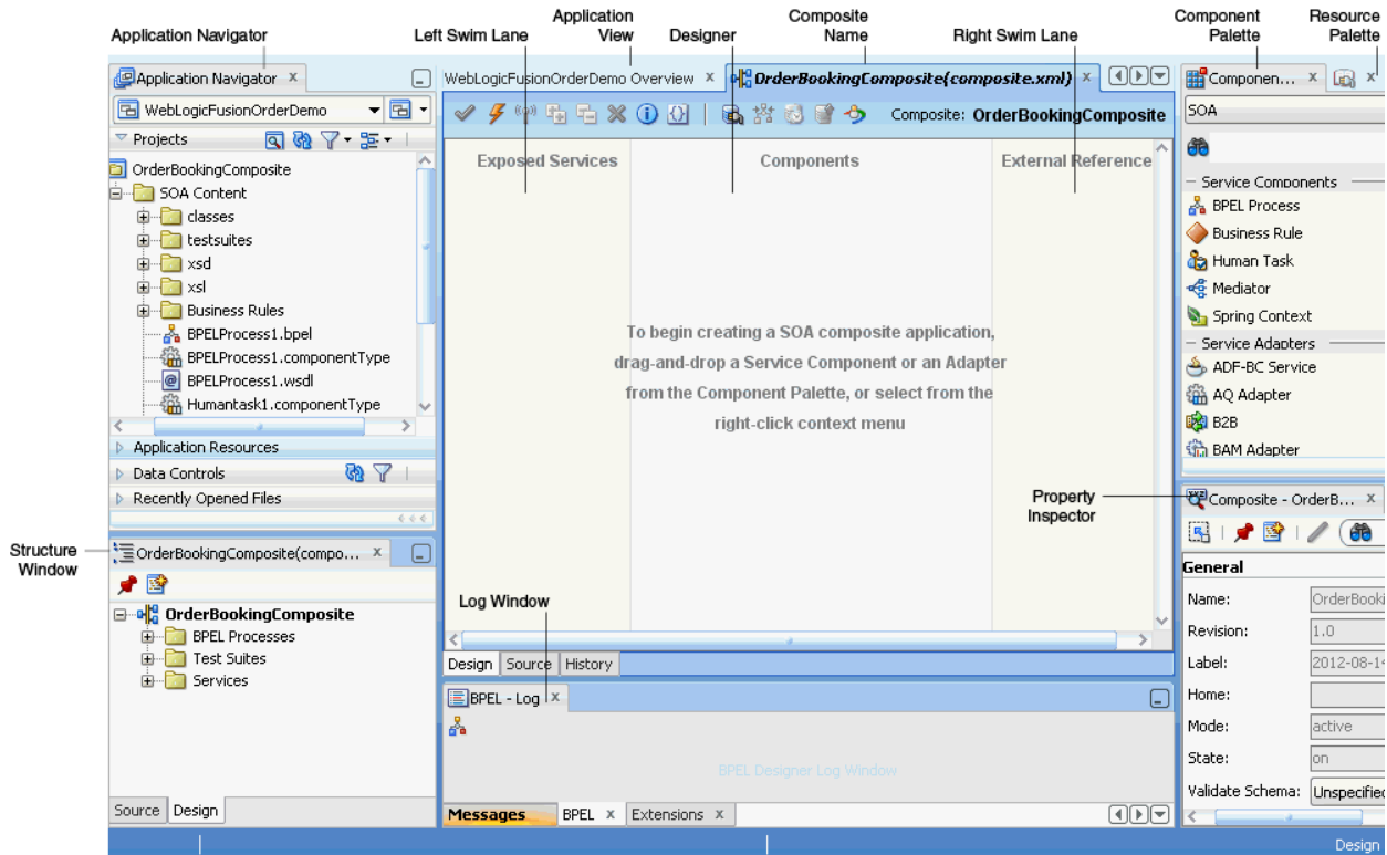
Figure 2–1 New Workspace for a SOA Composite Application
