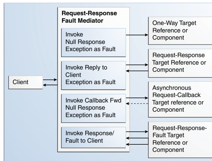
Figure 24-3 Request-Reply-Fault Message Exchange Pattern
