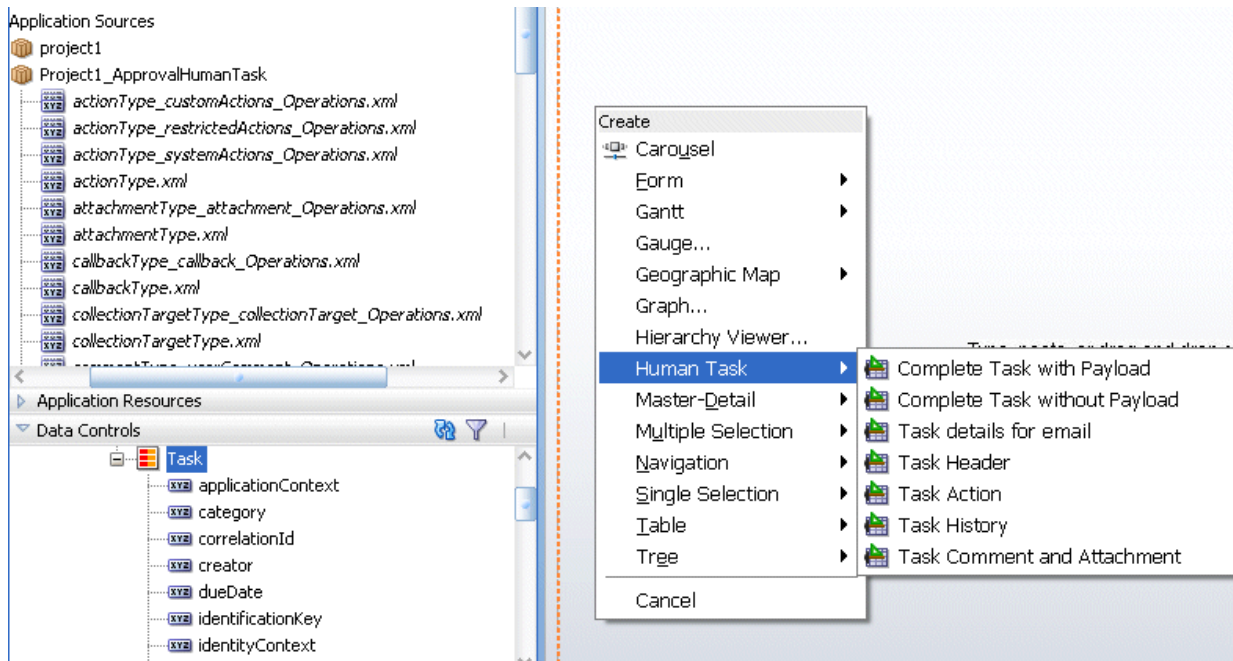
Figure 30–17 Human Task Drop Handlers for Creating the Task Form
