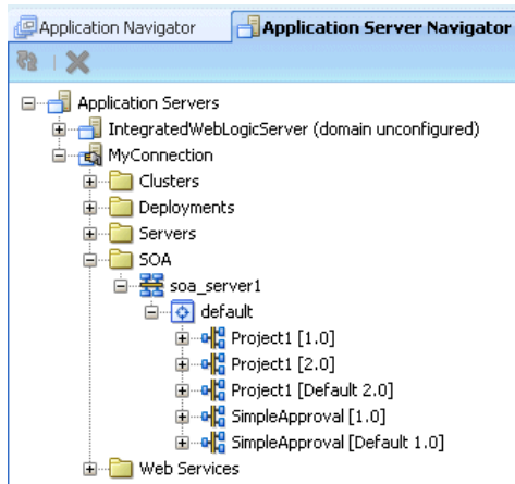
Figure 2–24 Deployed SOA Composite Applications
