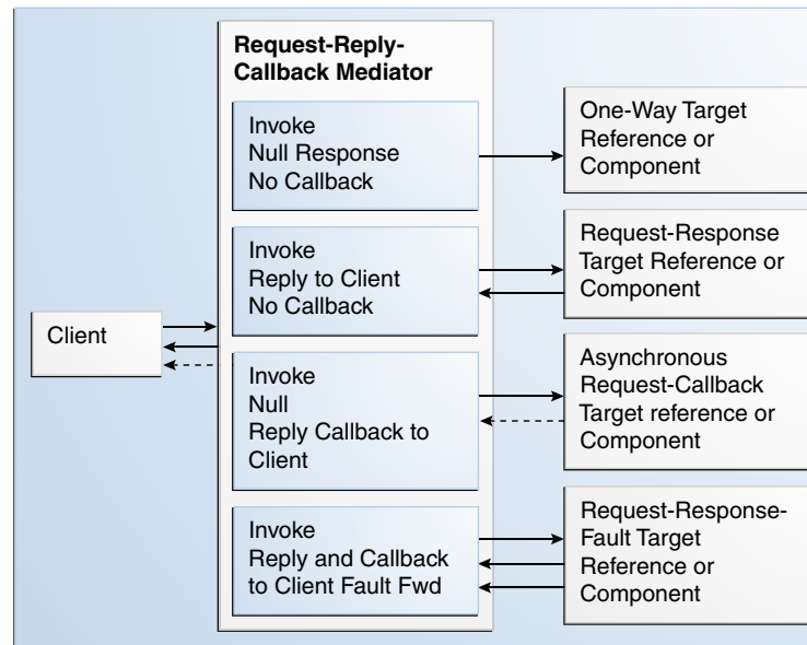
Figure 24–5 Request-Reply-Callback Message Exchange Pattern
