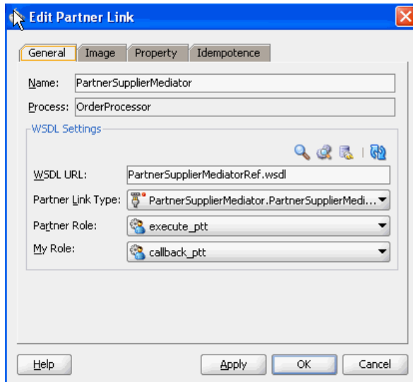
Figure A–23 Partner Link Activity
