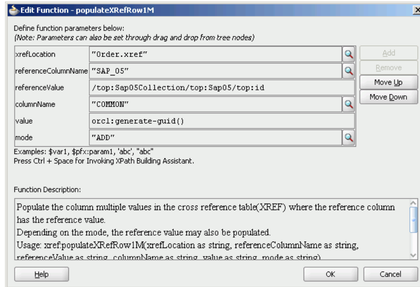
Figure 49–55 Edit Function – populateXRefRow1M Dialog: XrefOrderApp Use Case
