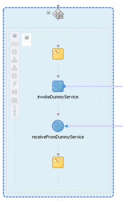
Figure 10–16 forEach Activity with Contained and Expanded Scope Activity
