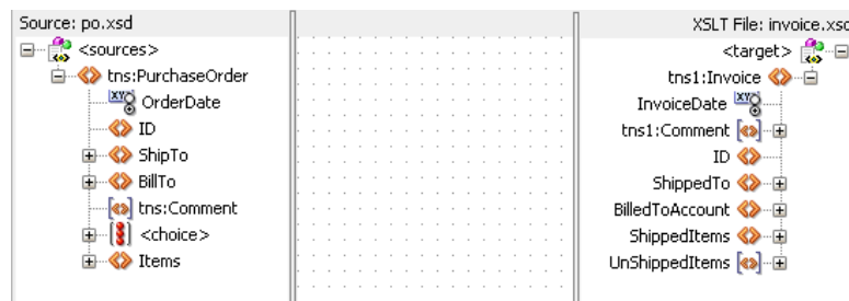
Figure 40–7 New XSL Map
