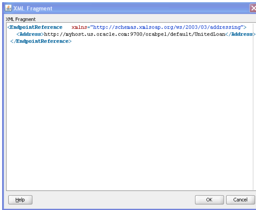
Figure 8–6 XML Fragment Dialog in BPEL 1.1
