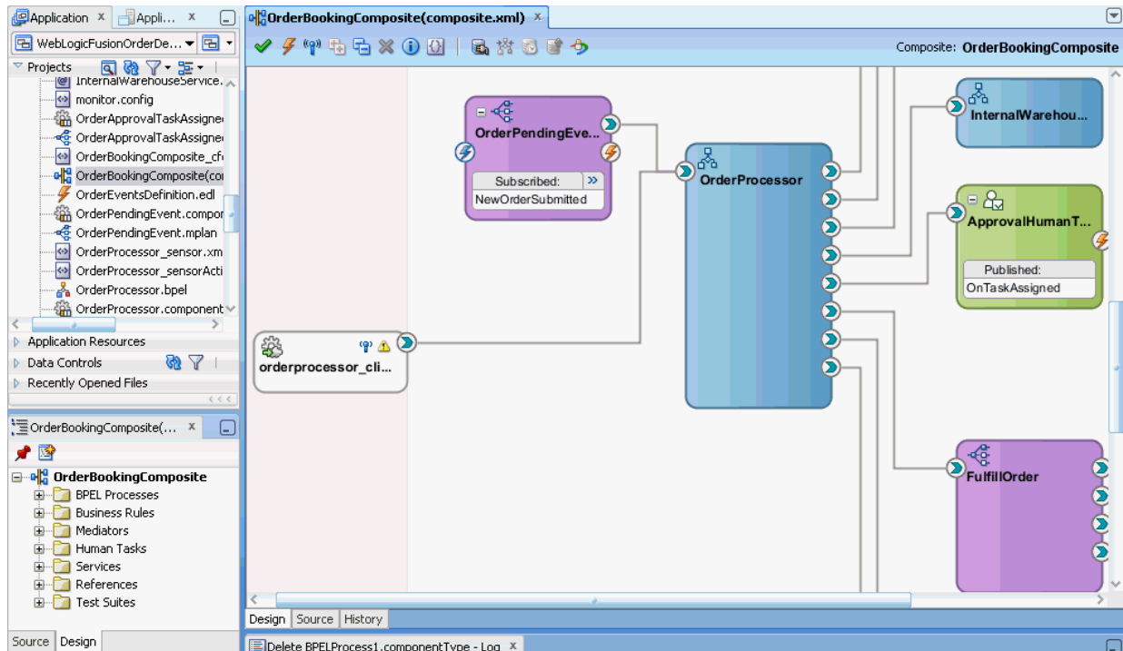
Figure 3-3 SOA Composite Editor
