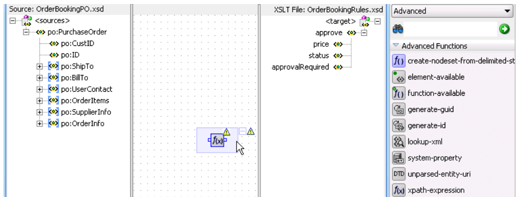
Figure 40–21 Editing XPath Expressions
