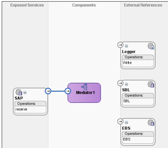
Figure 49-23 SAP Service Connected to Mediator1
