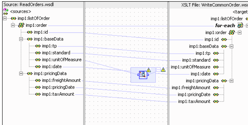
Figure 47-17 Adding lookupValue Function to imp1:listOfOrder To imp1:listOfOrder.xsl
