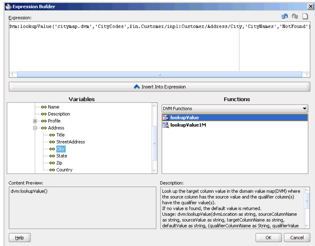
Figure 47–10 Domain Value Map Functions in the Expression Builder Dialog
