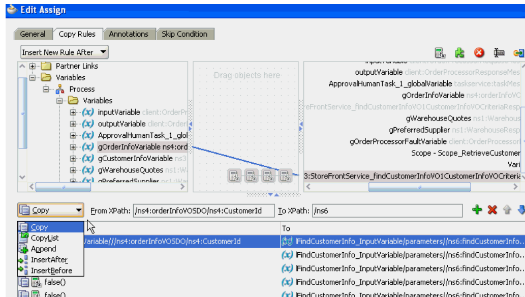
Figure 6-6 Copy Rule Converted to bpelx Extension in BPEL 1.1
