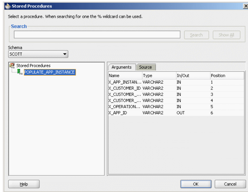
Figure 49–18 Stored Procedure Dialog
