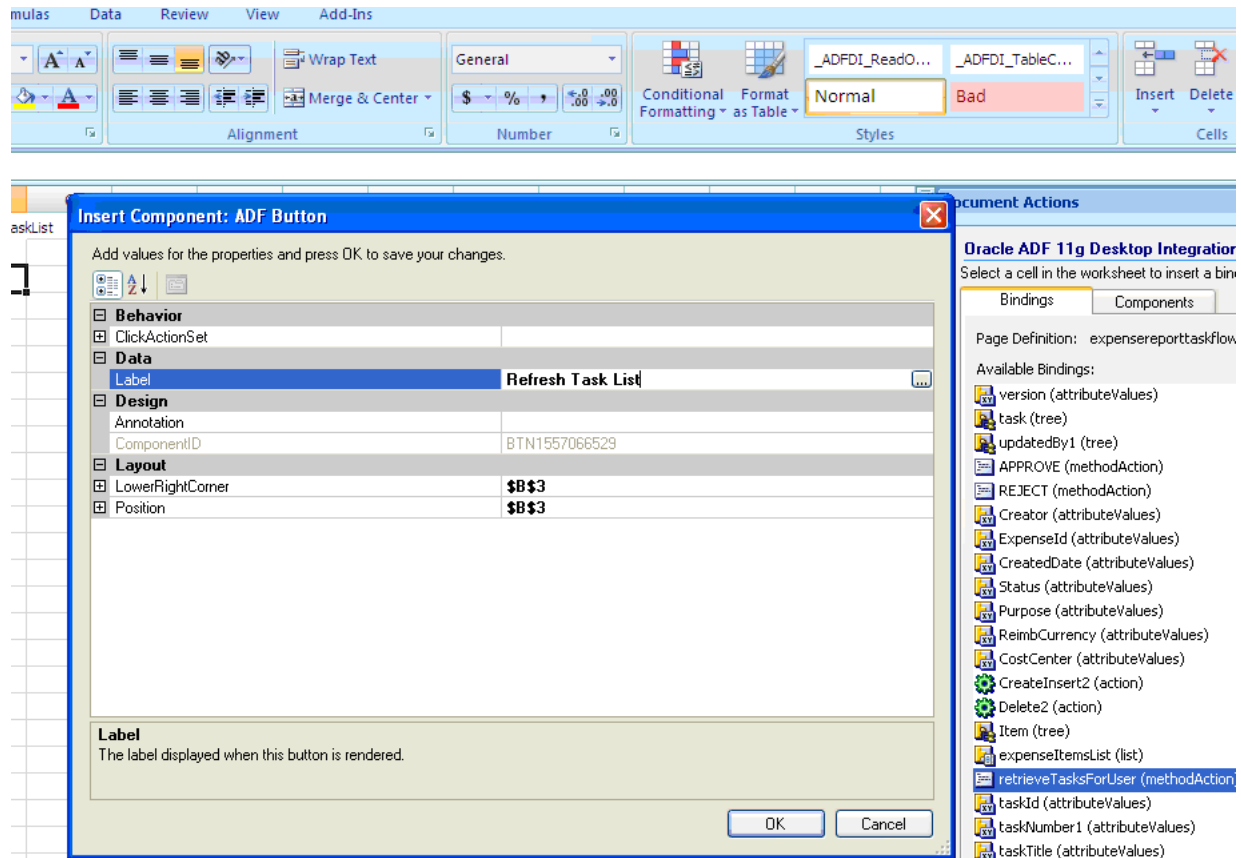
Figure 35–14 Excel: Inserting a methodAction Binding
