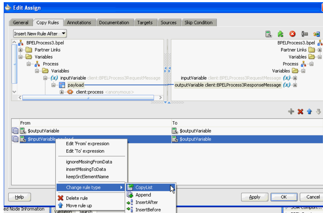
Figure 6–7 Copy Rule Converted to bpelx Extension in BPEL 2.0
