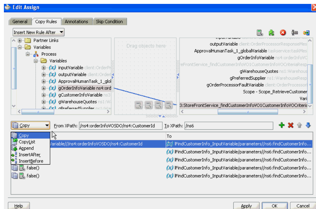
Figure A-4 Copy Rule Converted to bpelx Extension in BPEL 1.1
