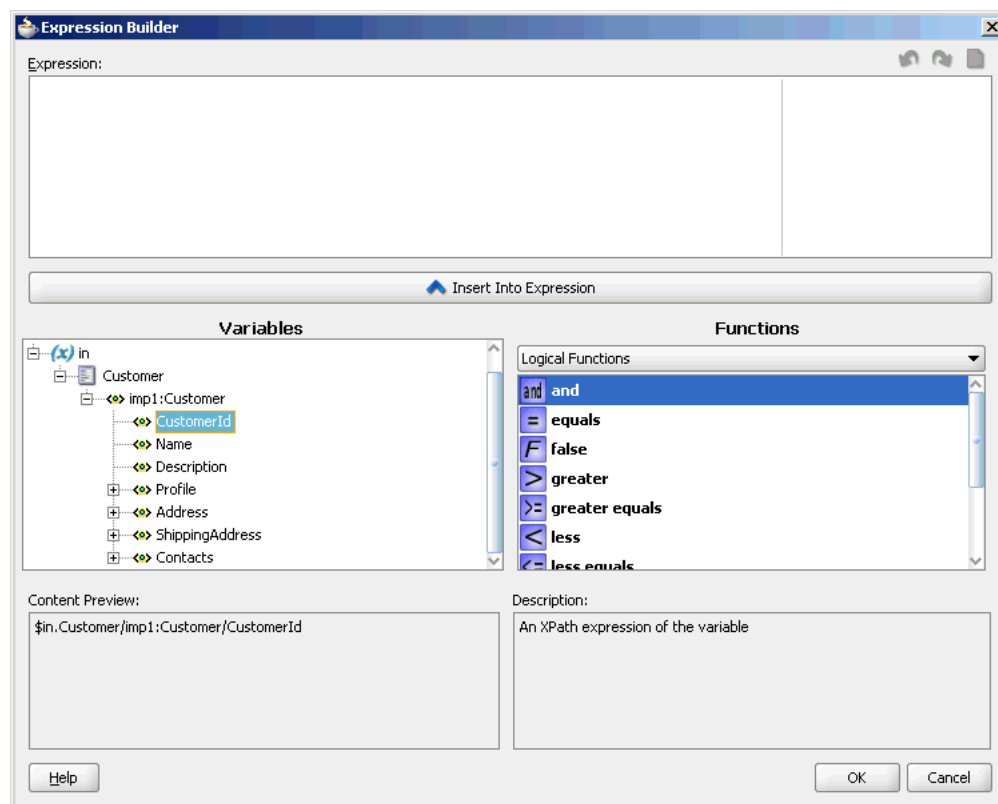
Figure 20–14 Expression Builder Dialog – Variables Element Selected
