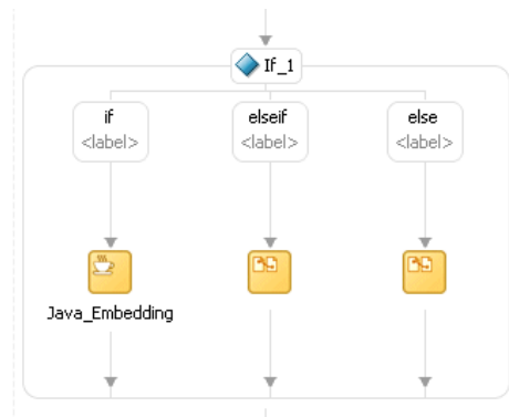
Figure 11–9 Completed If Activity
