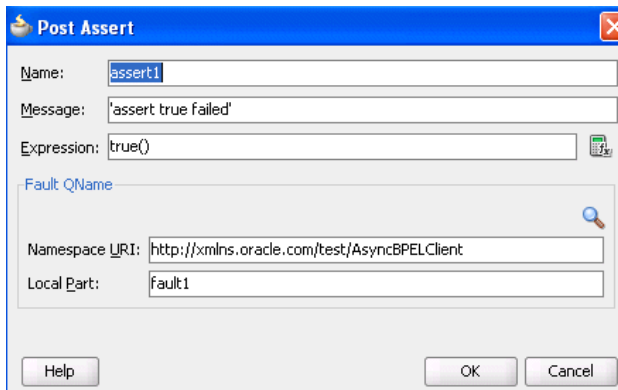
Figure 12–32 Assertion Condition Values
