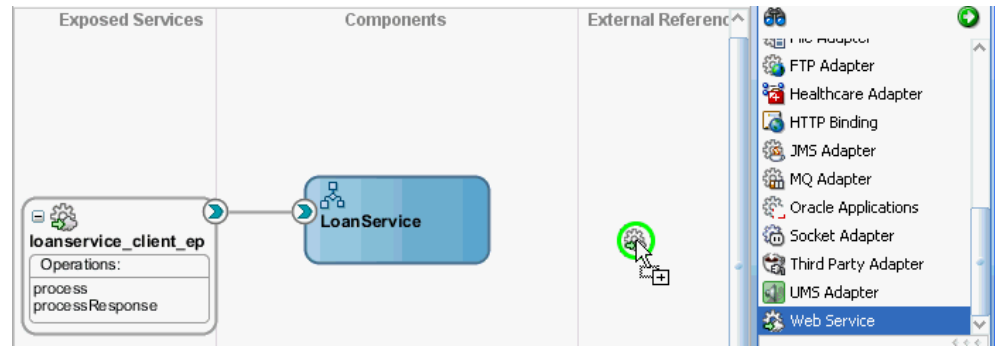
Figure 37–6 Integration of a Web Service Binding Component into a Composite
