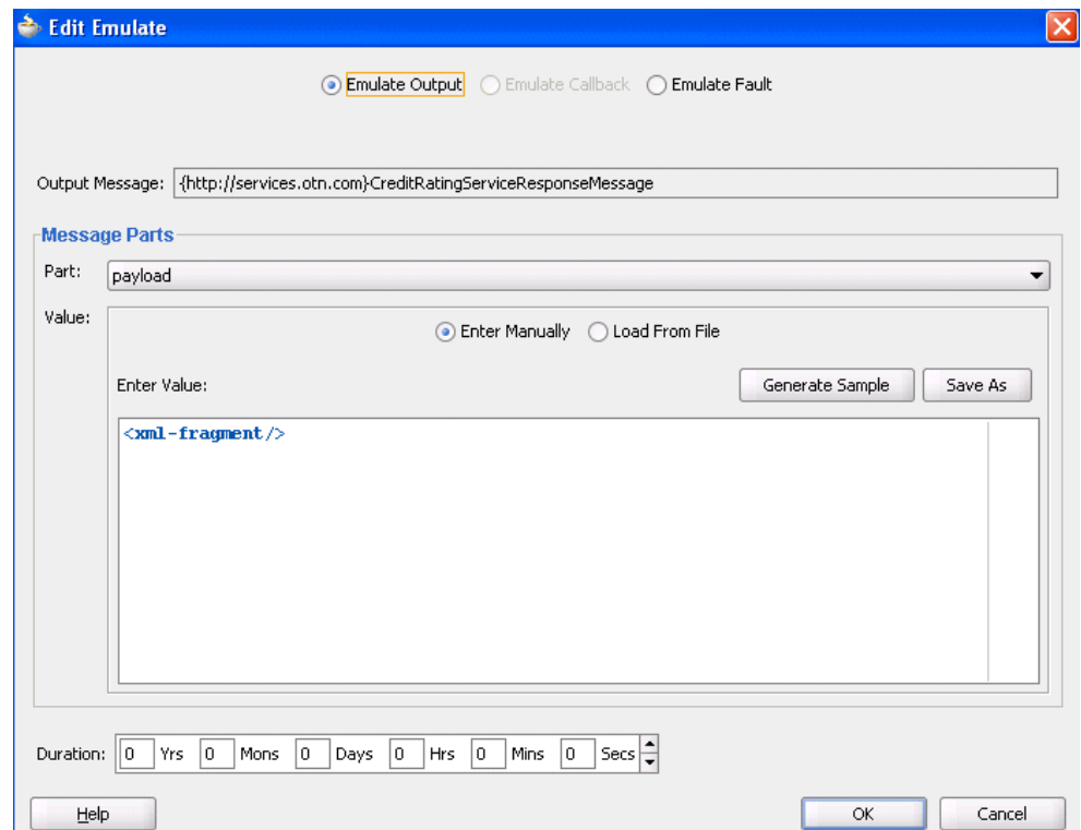
Figure 44–12 Emulate Dialog with Emulate Output Selected
