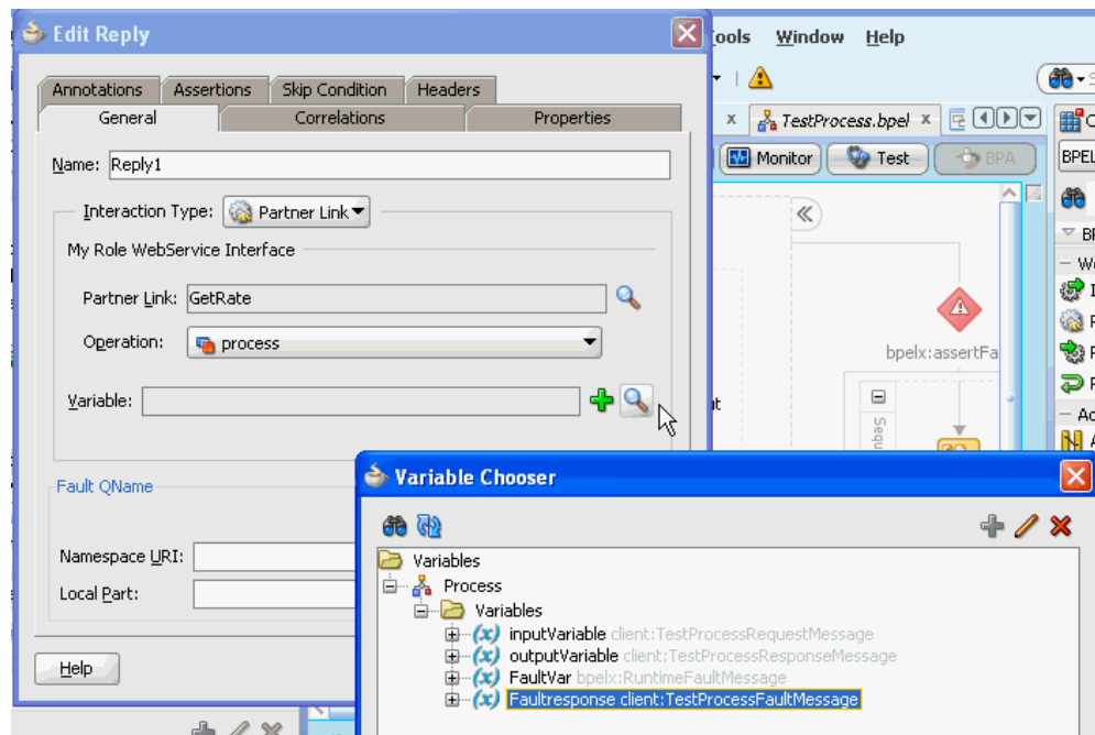
Figure 12–9 Variable Chooser Dialog
