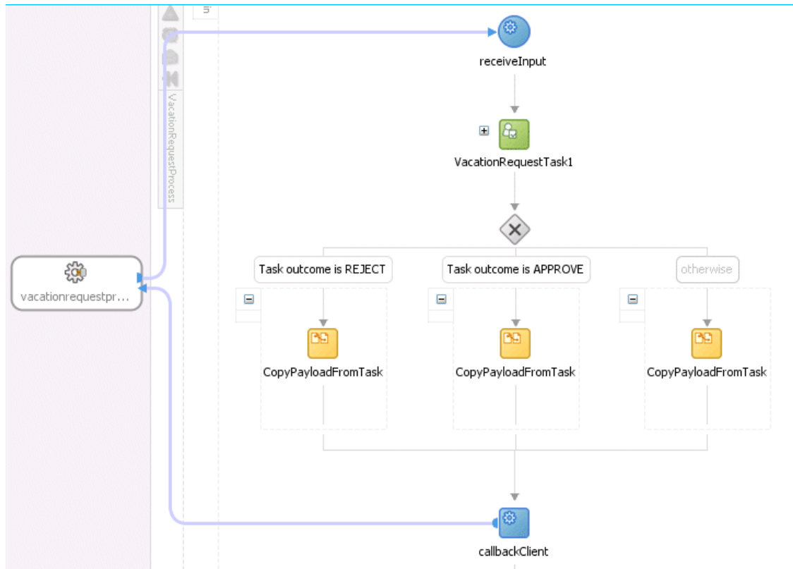
Figure 31–13 Human Task and Partner Links in Oracle BPEL Designer
