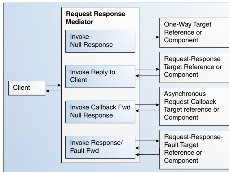
Figure 24-2 Request-Reply Message Exchange Pattern
