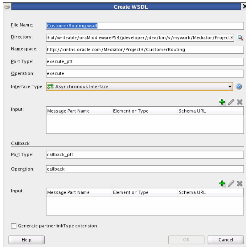
Figure 19-27 Create WSDL Dialog for an Asynchronous Interface
