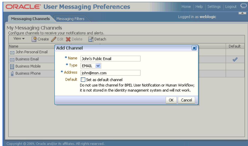
Figure 67–3 Creating a Channel
