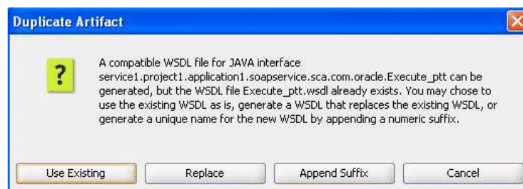
Figure 52-19 Existing WSDL File
