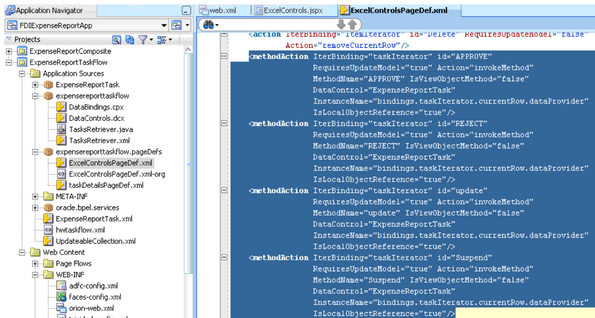
Figure 35–9 Oracle JDeveloper: Configuring the Page Definition File
