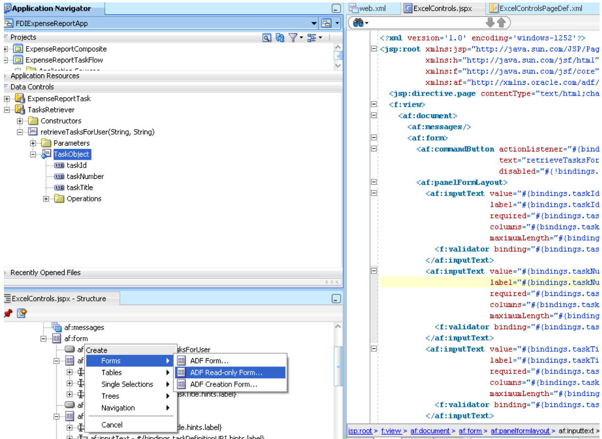
Figure 35–10 Oracle JDeveloper: Page Definition File
