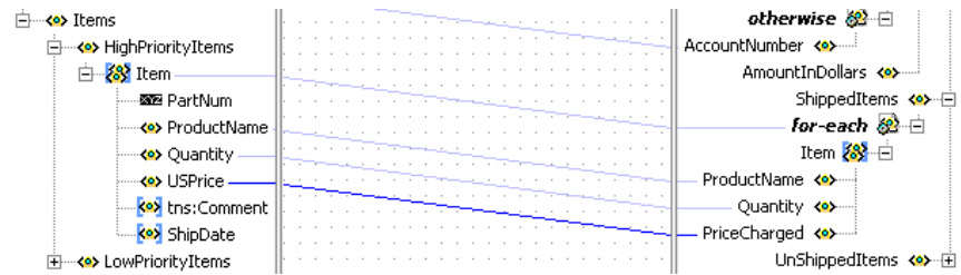
Figure 40–28 Creating Loops with xsl:for-each
