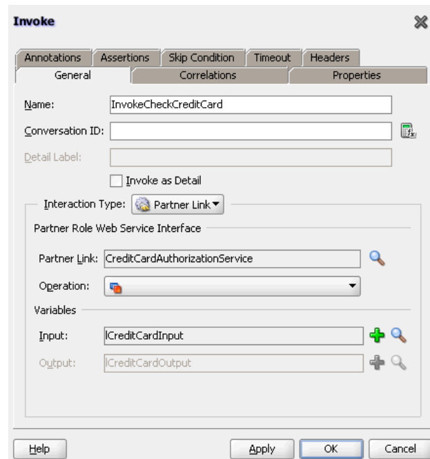
Figure 7-3 InvokeCheckCreditCard Invoke Activity
