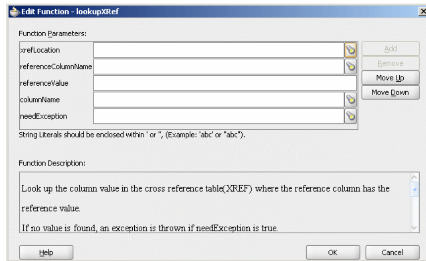
Figure 49–10 Edit Function – lookupXRef Dialog
