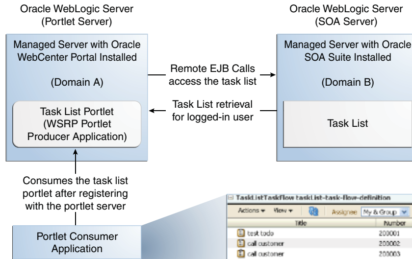
Figure 36–1 High Level Portlet Deployment and Usage
