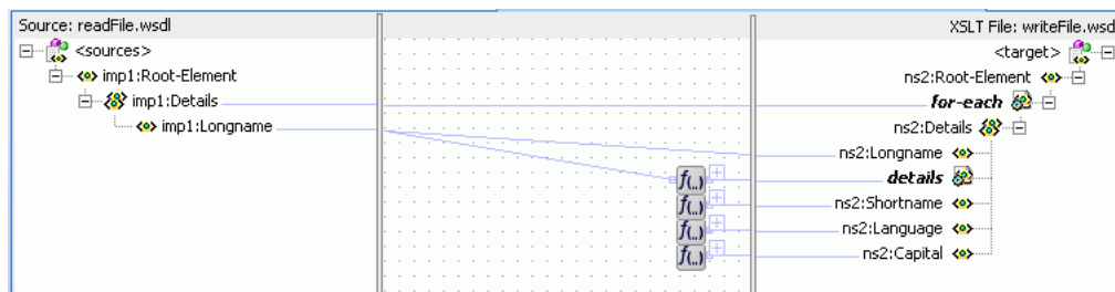
Figure 47-28 Complete imp1:Root-Element To ns2:Root-Element Transformation
