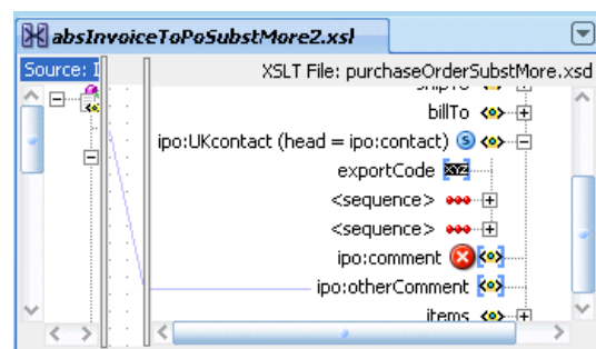
Figure 40-45 If the Element is in the Target Tree and Element Substitution is Selected
