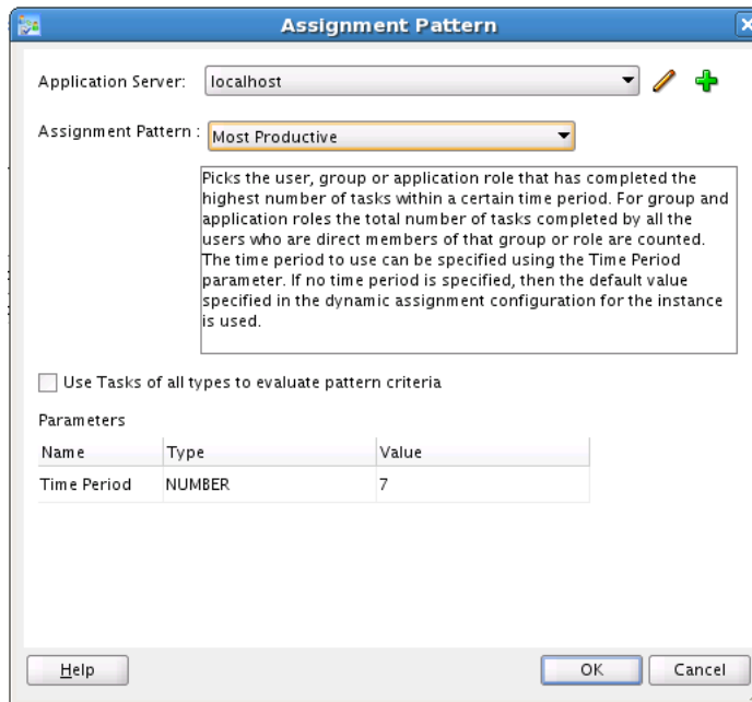
Figure 29–26 Selecting and Configuring an Assignment Pattern
