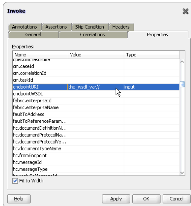
Figure 8–10 endpointWSDL Normalized Message Property of Invoke Activity
