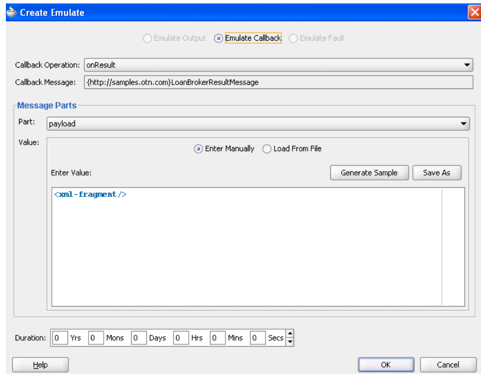
Figure 44–13 Emulate Dialog with Emulate Callback Selected
