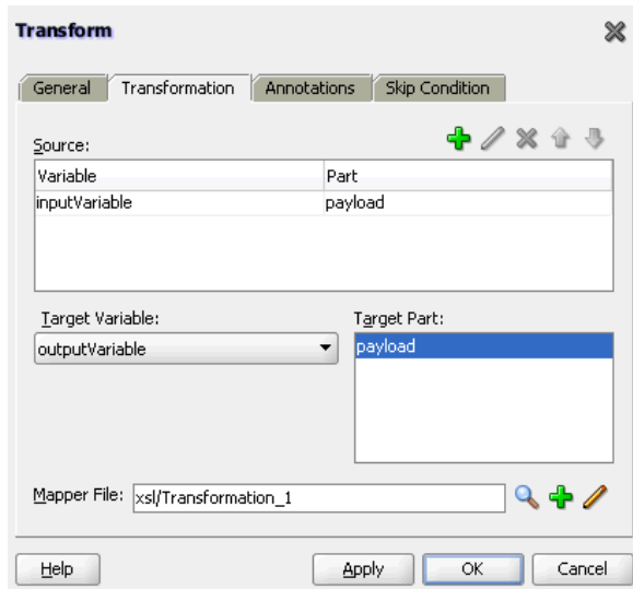
Figure A–43 Transform Dialog
