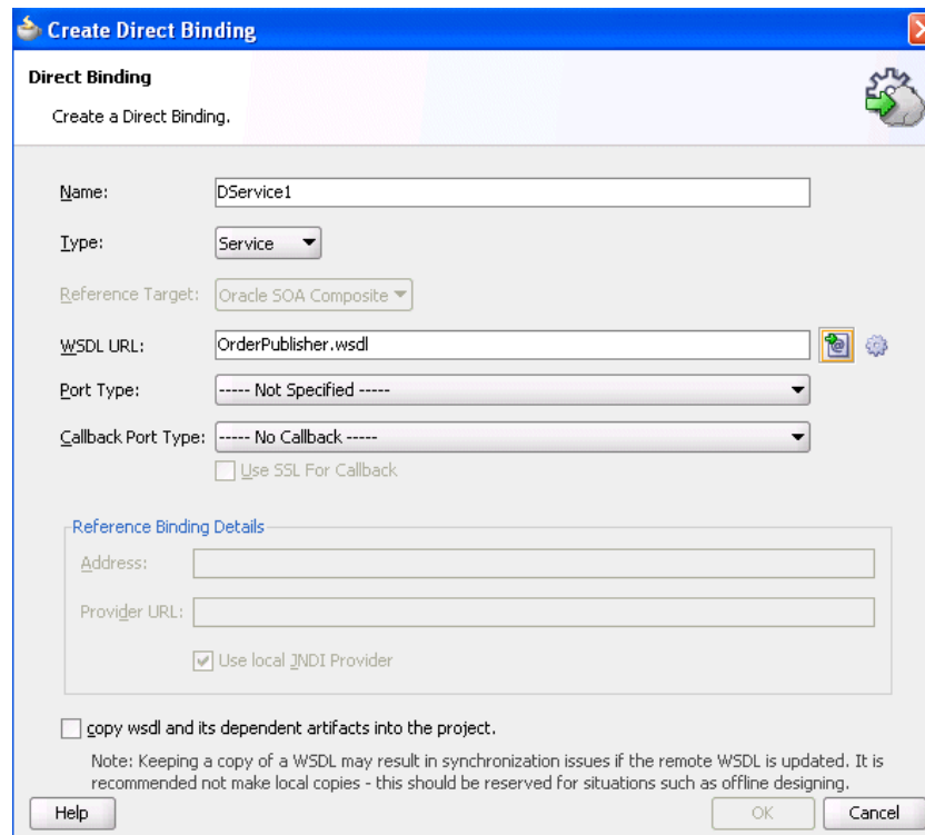
Figure 39–4 Create Direct Binding Dialog
