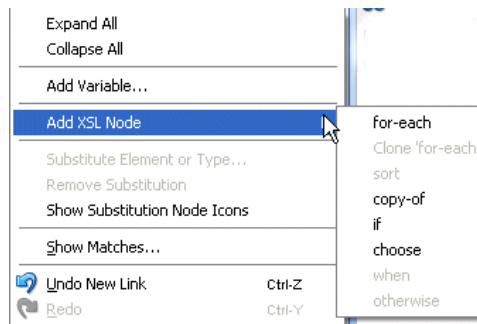
Figure 40–25 XSLT Constructs in Available Through the Context Menu
