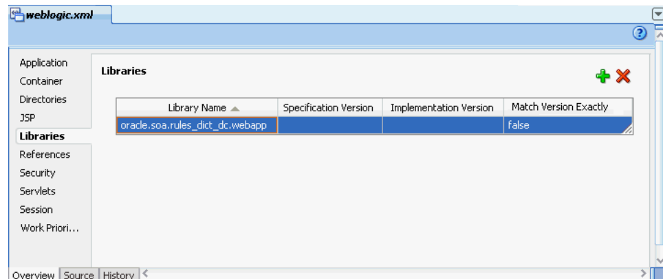
Figure 26–42 Adding the Rules Dictionary Component Library
