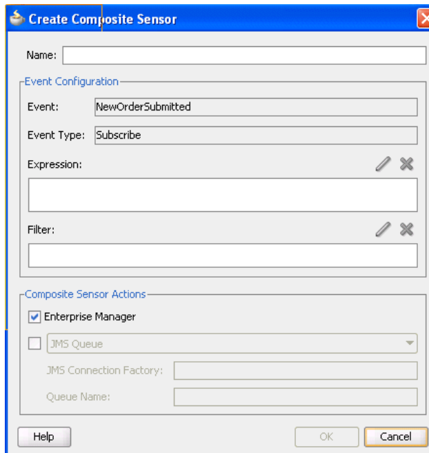
Figure 50–6 Create Composite Sensor Dialog for a Service Component
