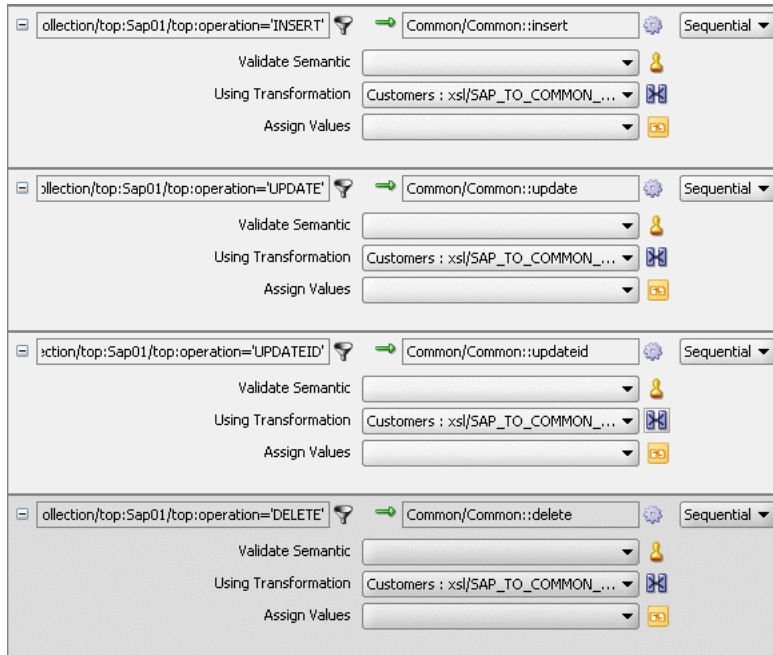
Figure 49–34 Insert, Update, UpdateID, and Delete Operations
