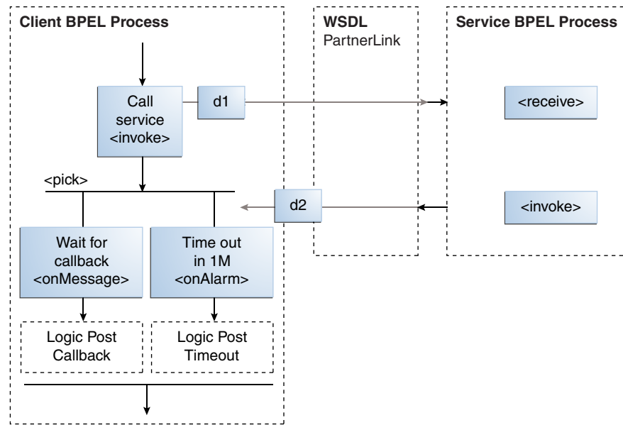
Figure 5–4 Asynchronous Interaction with Timeout
