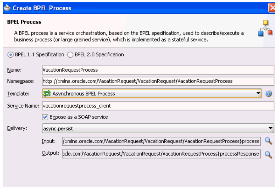
Figure 31–2 BPEL Process Dialog
