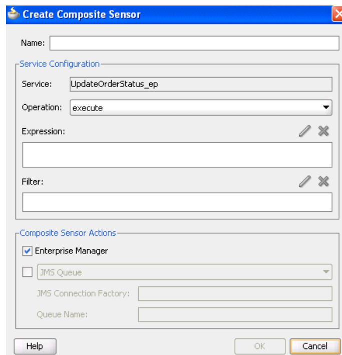
Figure 50–5 Create Composite Sensor Dialog for a Service Binding Component
