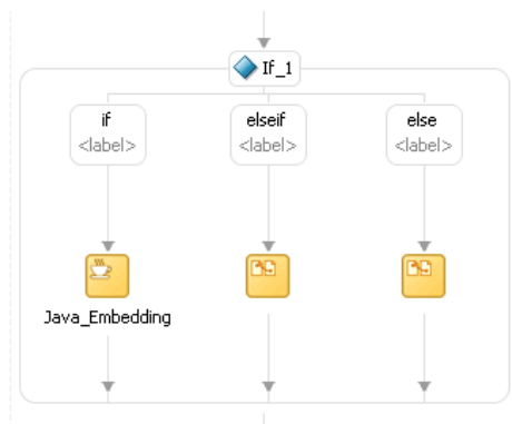
Figure A-19 If Activity
