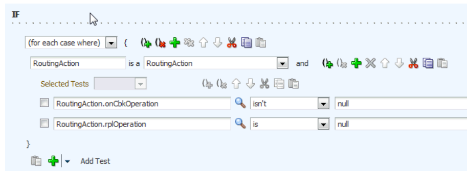
Figure 26–2 Simple Tests or Conditions in a Rule
