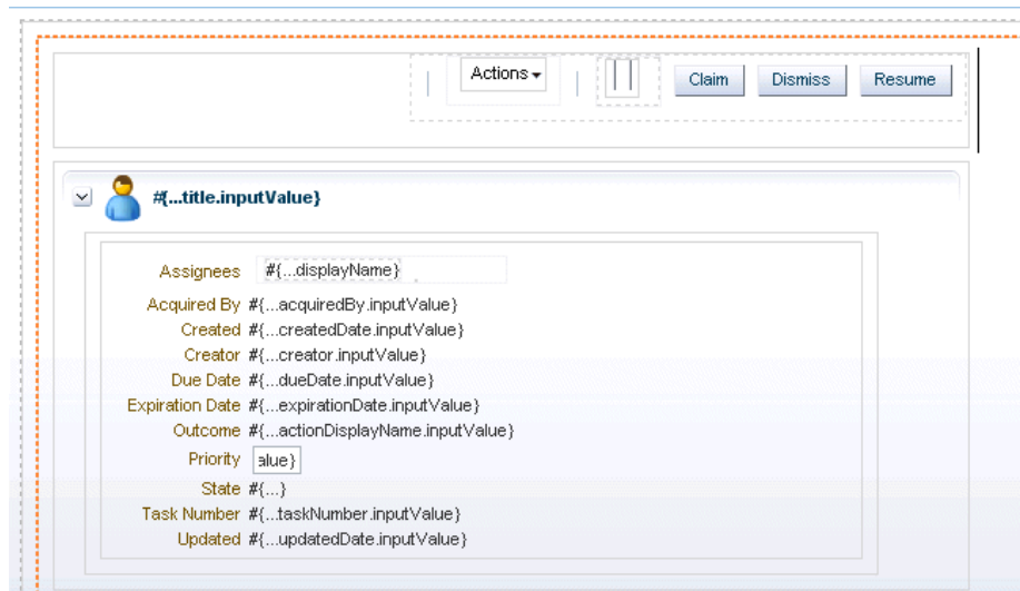
Figure 30–15 Custom Task Form (Upper Part of Tab)
