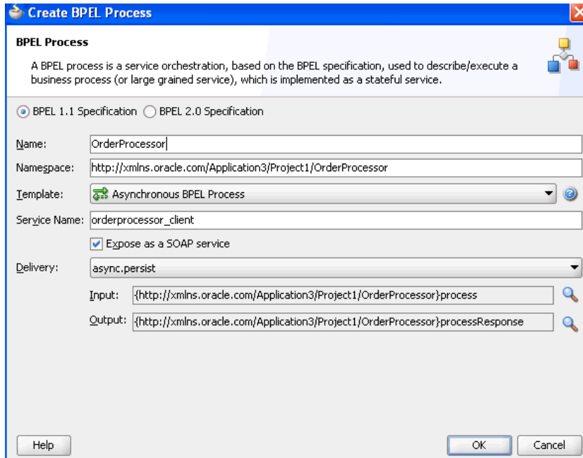
Figure 2–3 Create BPEL Process Dialog
