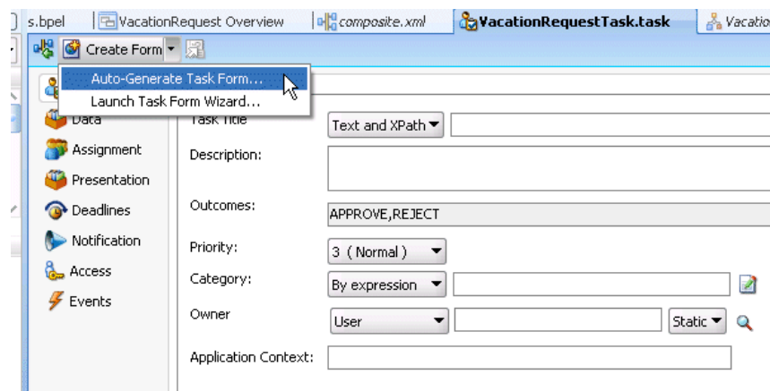
Figure 31-16 Task Form Creation
