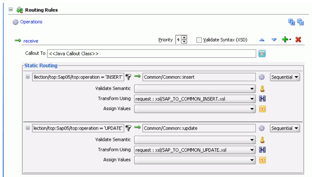
Figure 49–58 Insert Operation and Update Operation
