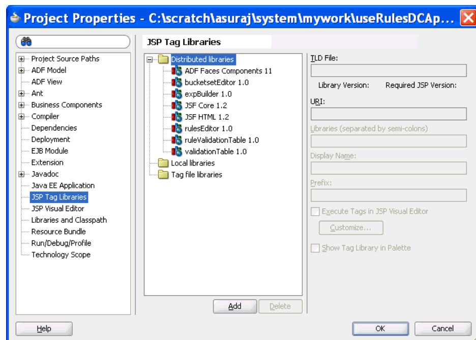
Figure 26-17 Checking the Required Tag Libraries
