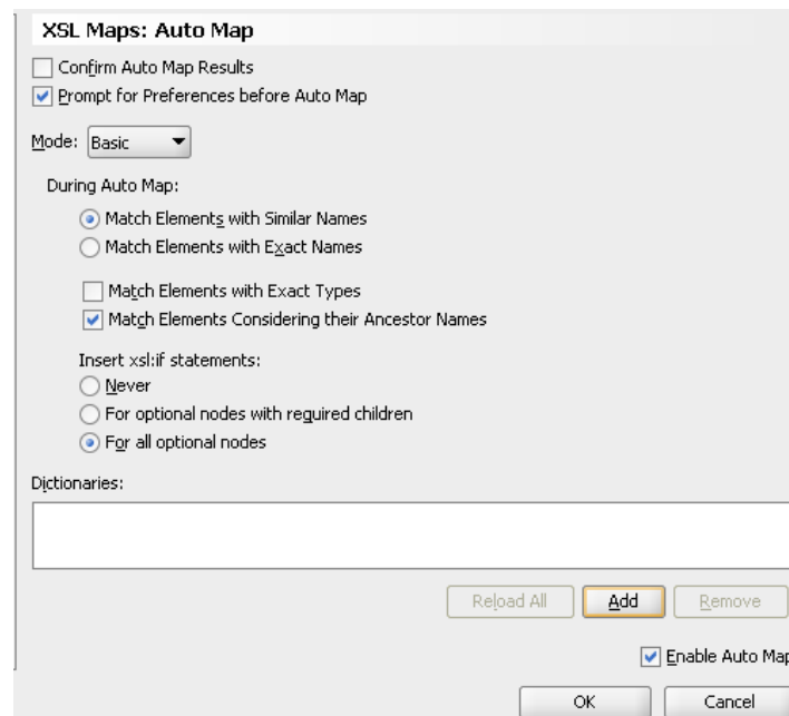
Figure 40–37 XSL Maps: Auto Map Dialog
