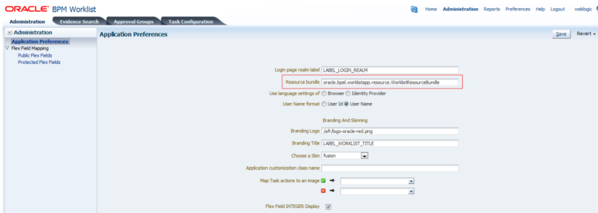
Figure 32–43 Specifying the Resource Bundle
