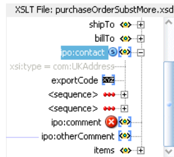
Figure 40-43 If the Element is in the Target Tree and Type Substitution is Selected
