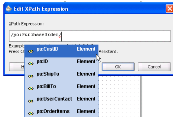
Figure 40–23 The XPath Building Assistant
