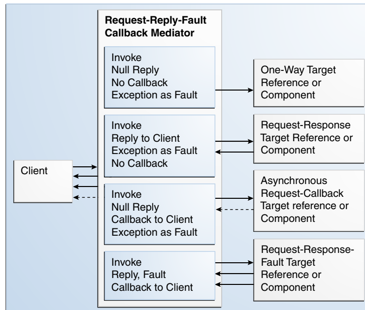
Figure 24–6 Request-Reply-Fault-Callback Message Exchange Pattern
