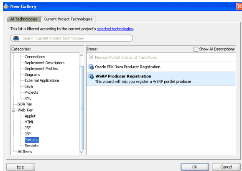
Figure 36–5 WSRP Producer Registration
