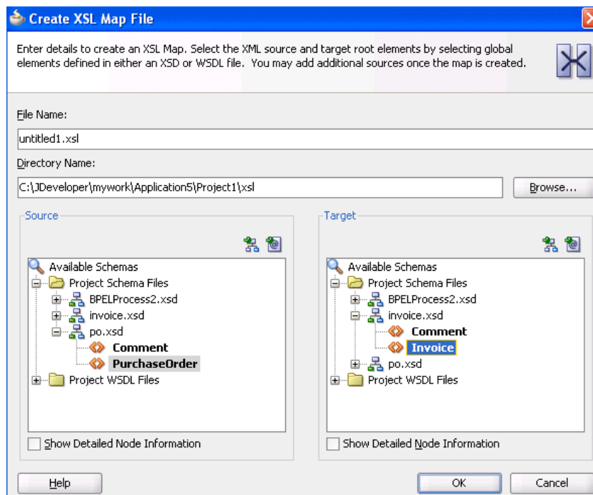
Figure 40-6 Expanded Target Section
