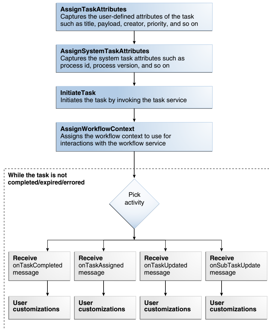
Figure 28–14 Workflow Interaction Modeling (with Callbacks)
