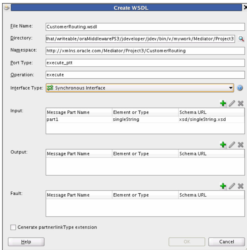
Figure 19-24 Create WSDL Dialog for a Synchronous Interface
