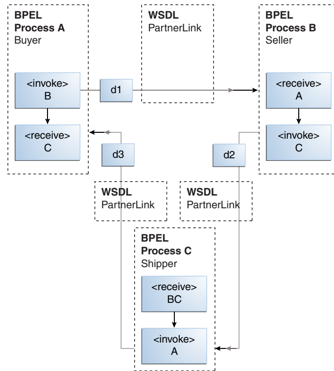
Figure 5–10 Multiple Party Interactions
