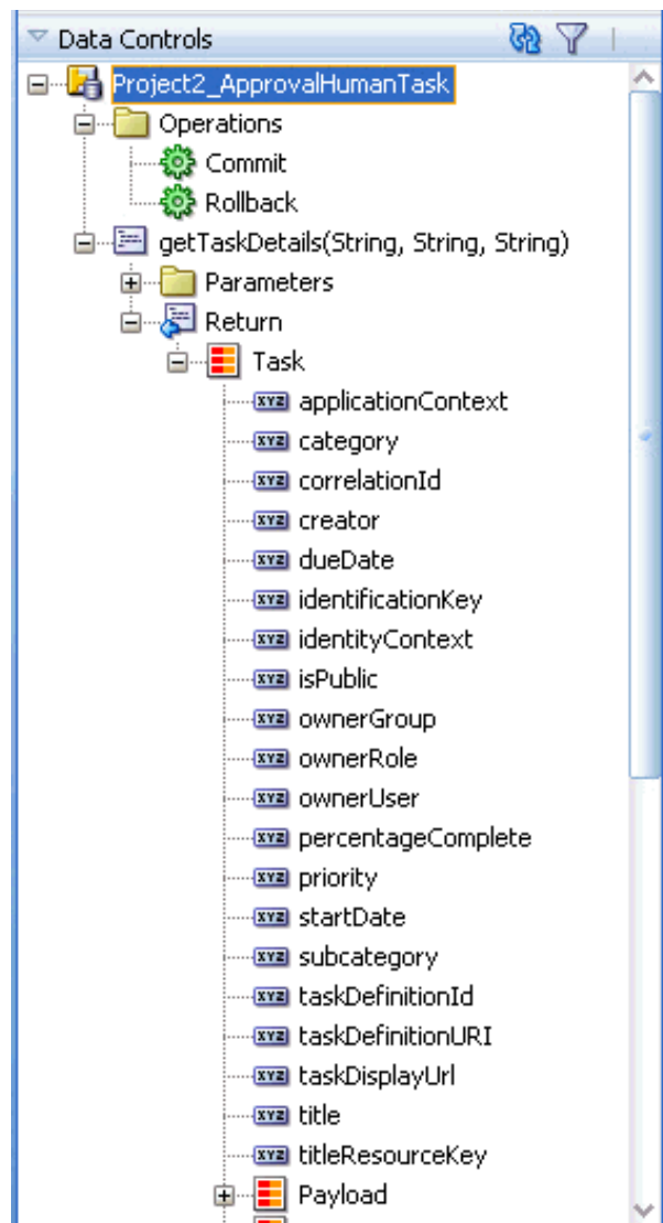
Figure 30-5 The Task Collection in the Data Controls Panel
