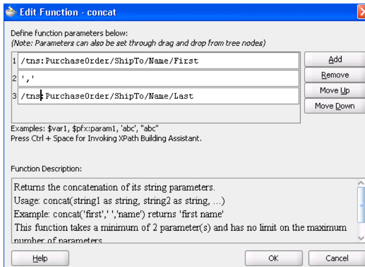
Figure 40–19 Editing Function Parameters
