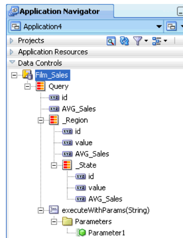
Figure 54–1 Data Controls Panel in Oracle JDeveloper
