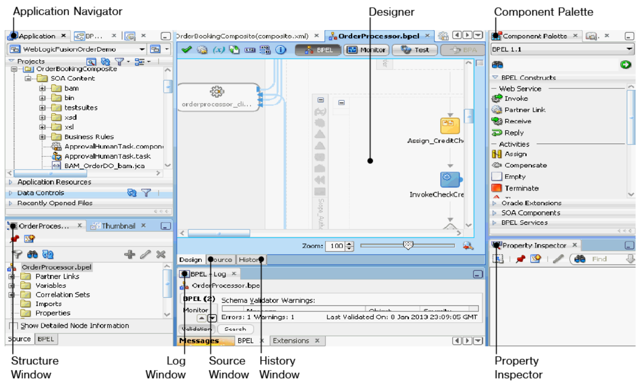
Figure 4–2 Oracle BPEL Designer Sections
