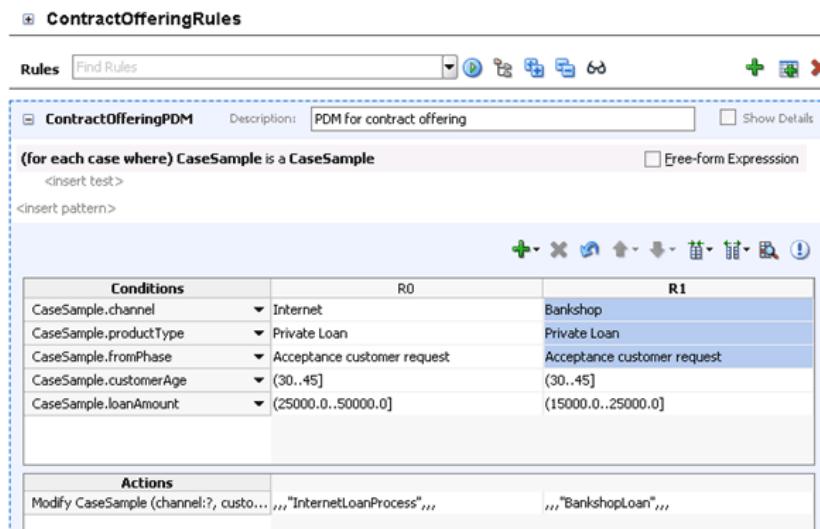
Figure 51–3 Sample Decision Table
