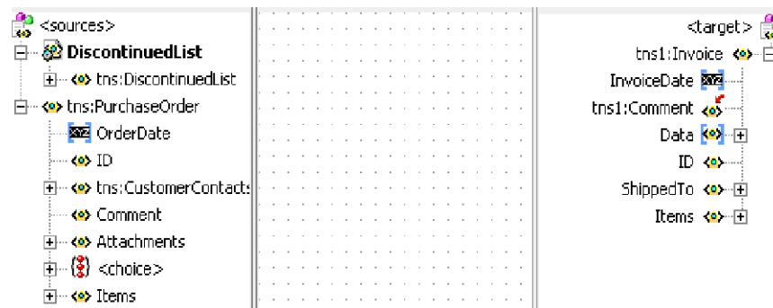
Figure 40-52 XSLT Mapper File
