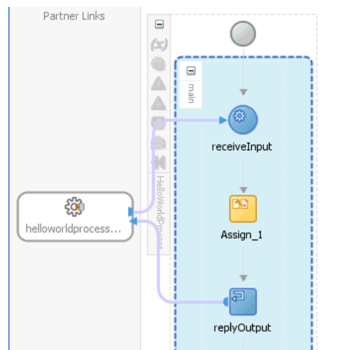
Figure A-2 Selected BPEL Process
