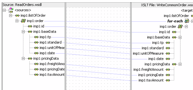
Figure 47-16 imp1:listOfOrder To imp1:listOfOrder Transformation
