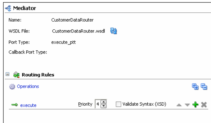
Figure 19–14 One-Way Interface Oracle Mediator in the Mediator Editor
