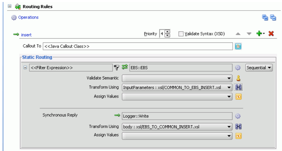
Figure 49–61 Insert Operation with EBS Target Service
