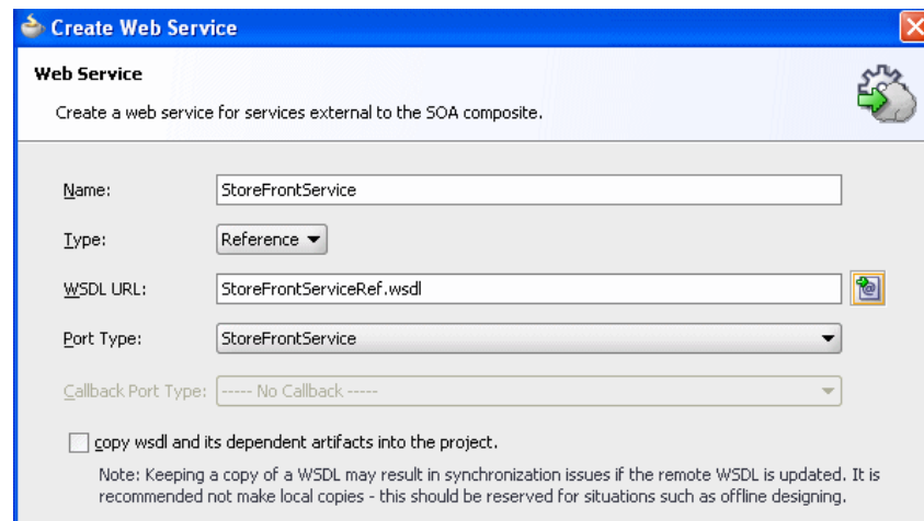
Figure 2–15 Create Web Service Dialog
