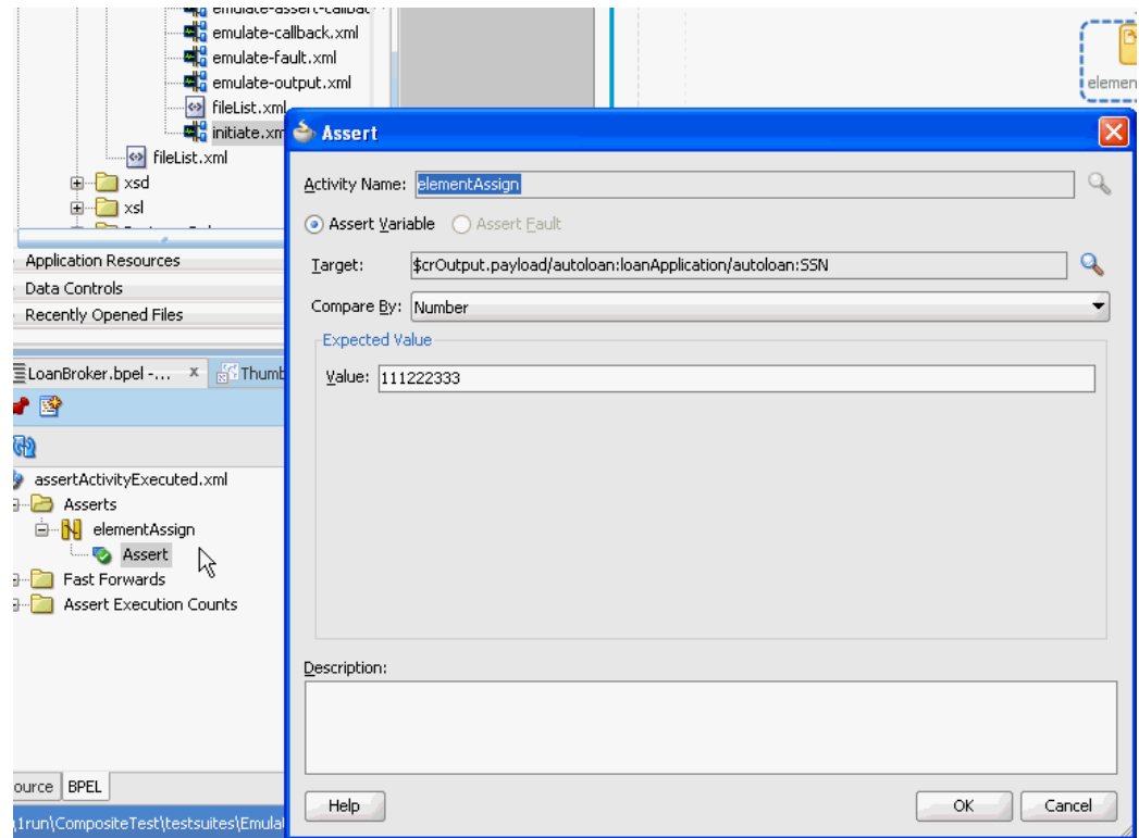
Figure 44–24 Assert Folder in Structure Window
