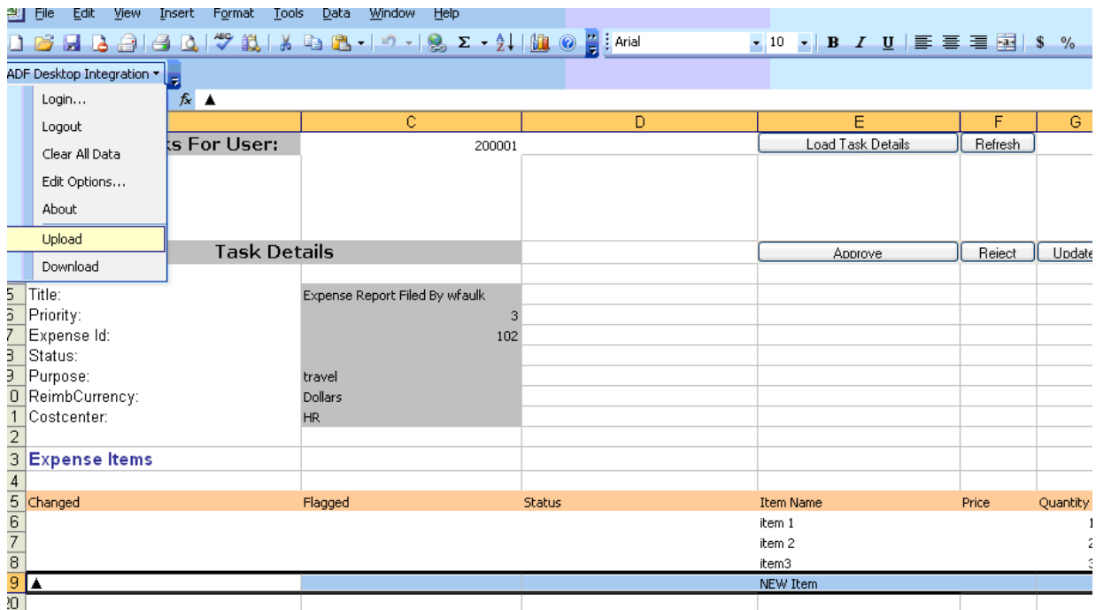
Figure 35–20 ADF Desktop-Integrated Excel Workbook Uploading New Items
