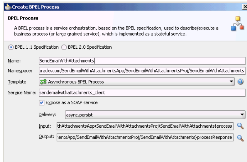
Figure J-24 Creating the BPEL Process
