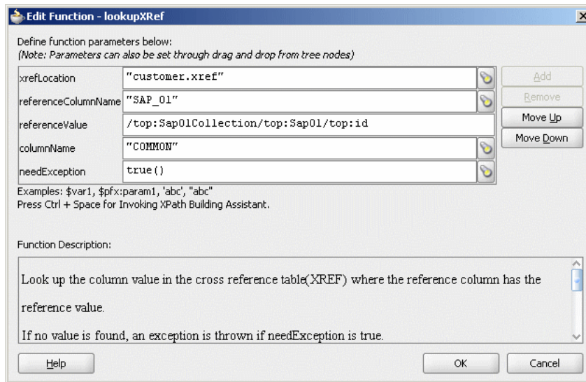
Figure 49–27 Edit Function – lookupXRef Dialog: XrefCustApp Use Case
