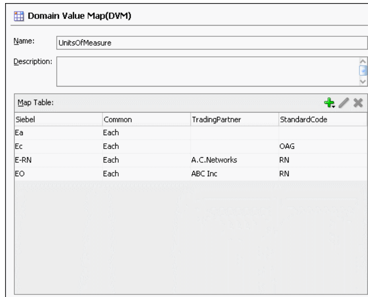
Figure 47-11 UnitsOfMeasure Domain Value Map
