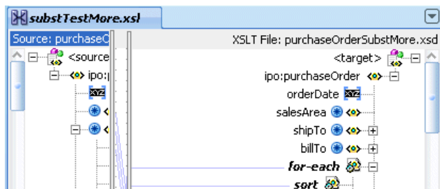
Figure 40–47 All Possible Substitutions
