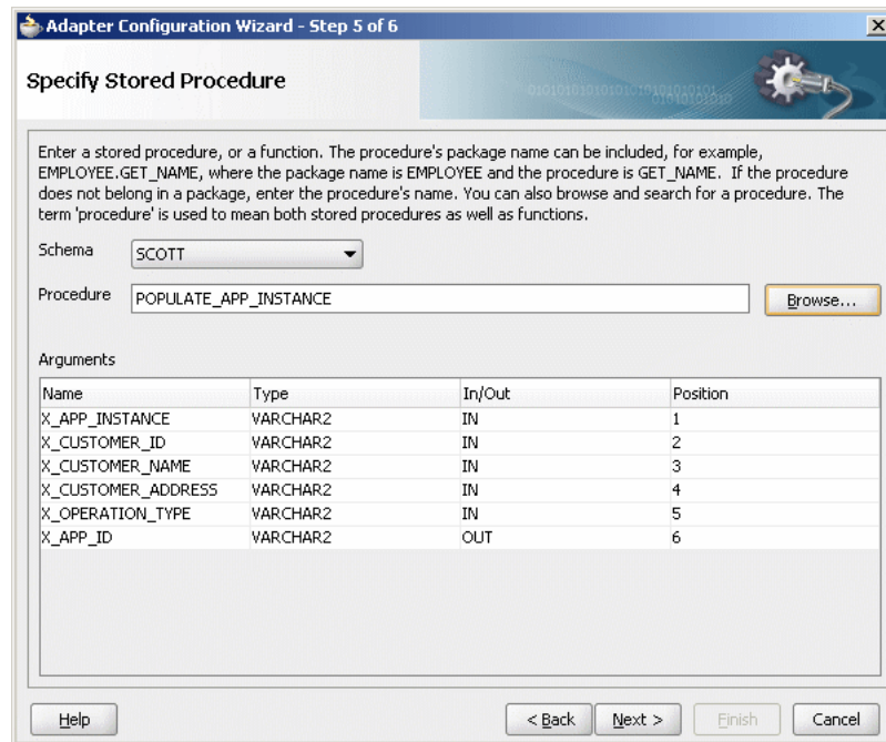
Figure 49–19 Specify Stored Procedure Page of Adapter Configuration Wizard
