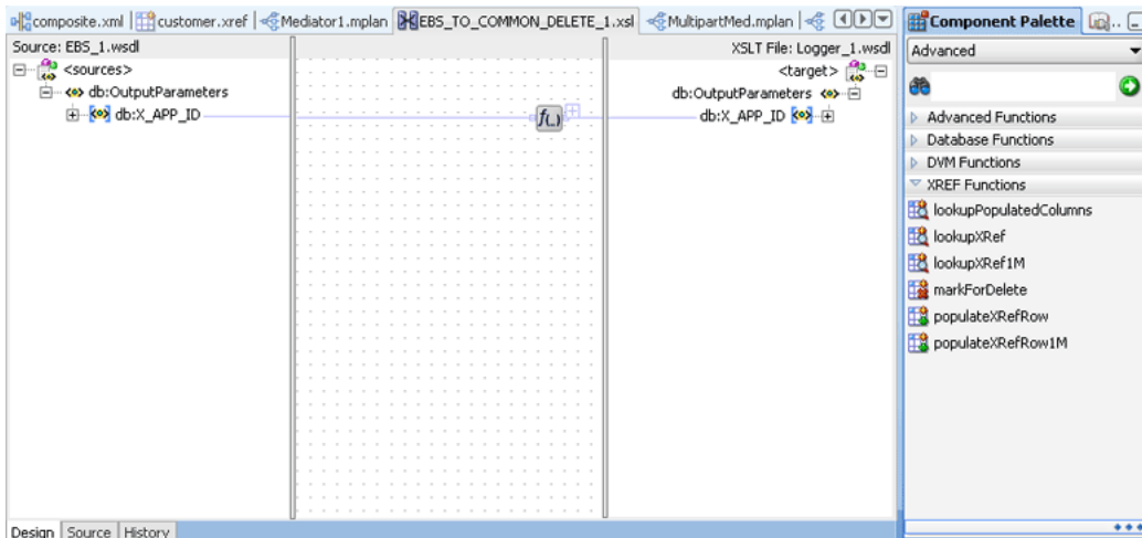
Figure 49–7 XSLT Mapper Dialog with Cross Reference Functions
