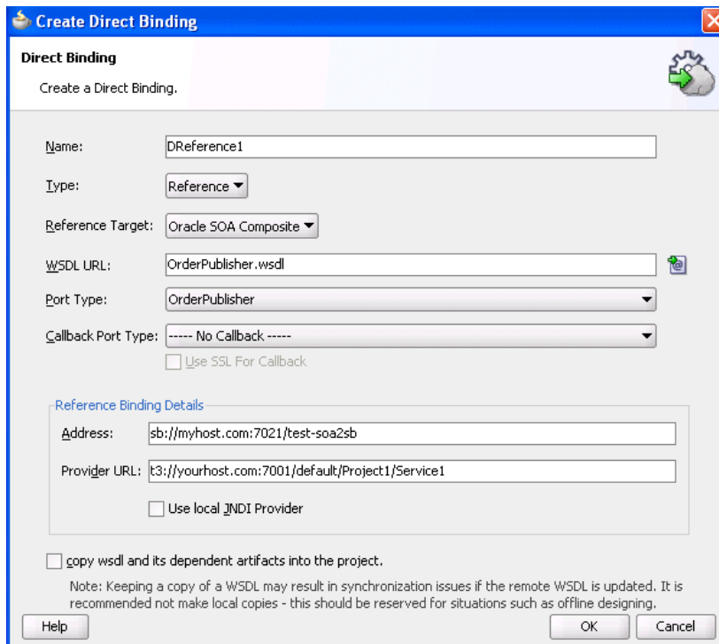
Figure 39–6 Create Direct Binding Dialog
