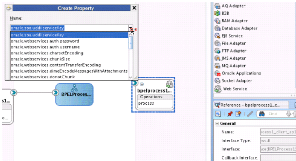
Figure A–52 serviceKey Properties
