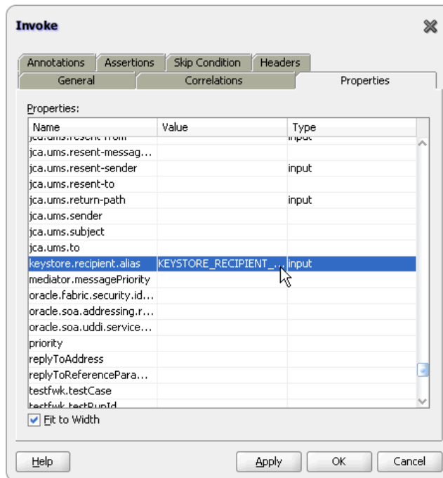
Figure 8–9 keystore.recipient.alias Normalized Message Property of Invoke Activity
