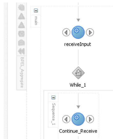
Figure 9-5 Routing a New Message to a New or Existing Instance
