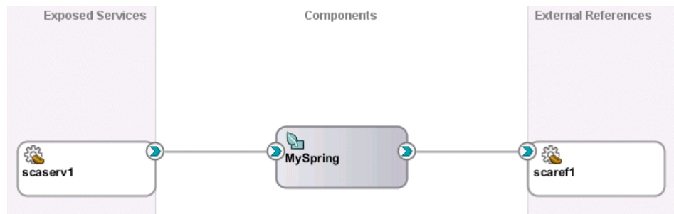
Figure 52–14 Java Interface-Based EJB Service and Reference Binding Components
