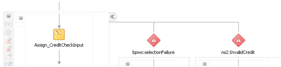
Figure 12–21 Catch Activities in the Designer
