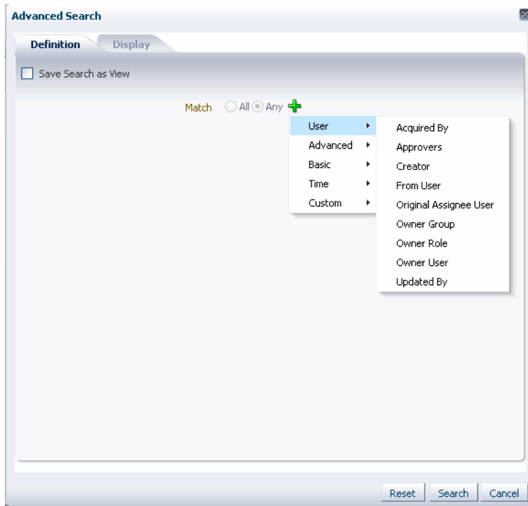
Figure 32–9 Adding Filters for an Advanced Search on Tasks
