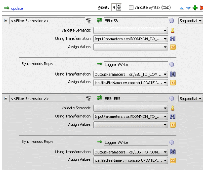
Figure 49–43 Update Operation with SBL and EBS Target Service
