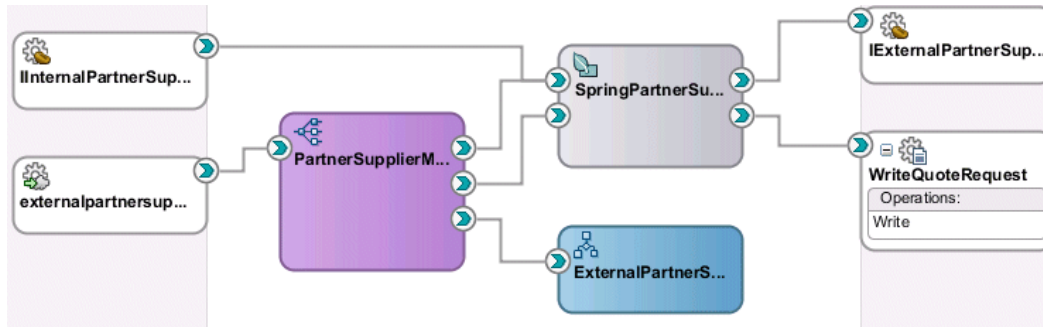
Figure 52–22 Partner Supplier Composite with Spring Service Component
