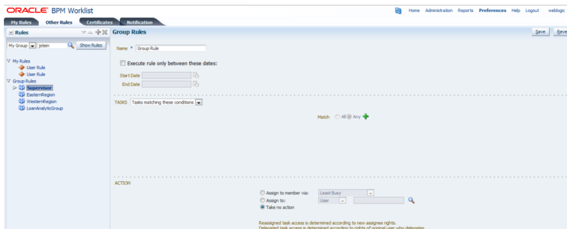
Figure 32–39 Creating a Group Rule
