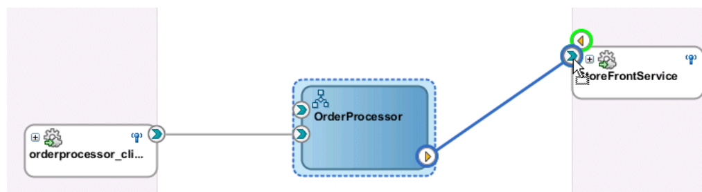
Figure 2–20 Wiring of a Service Component and Reference
