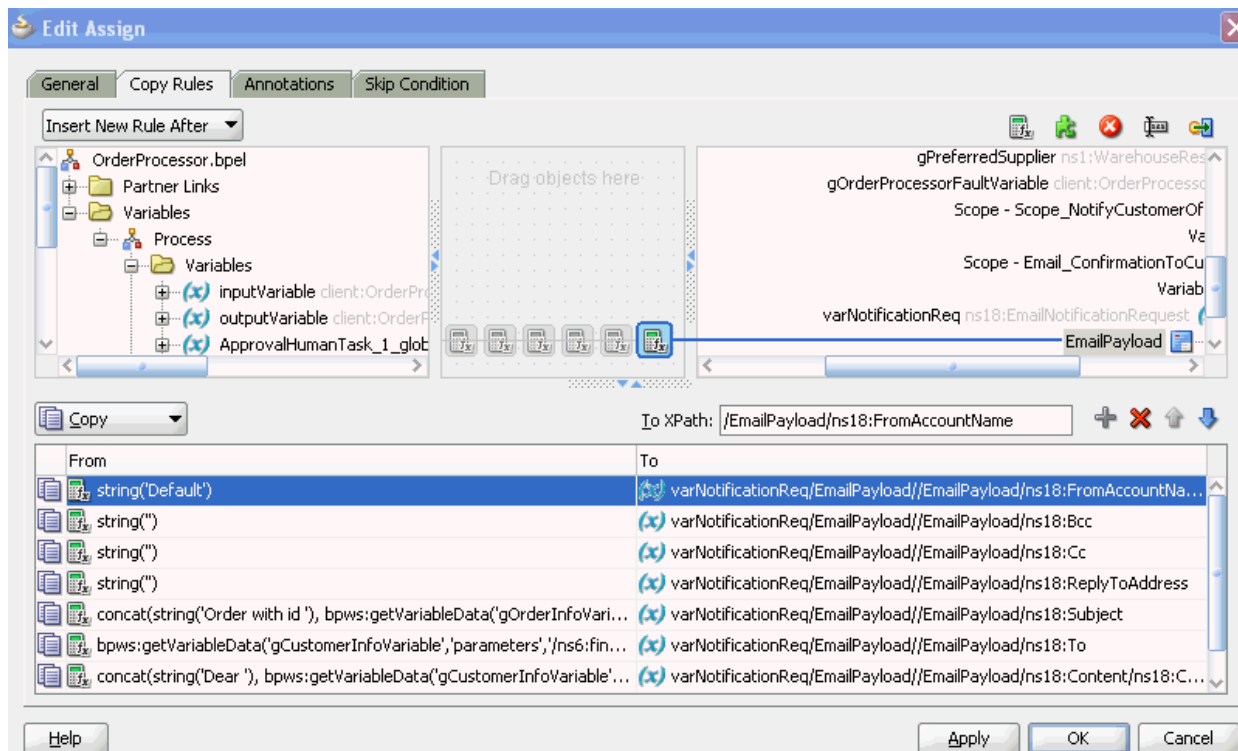
Figure 17-5 EmailParamsAssign Assign Activity
