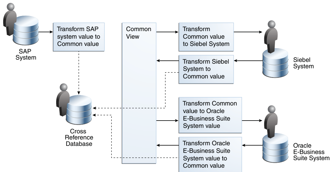
Figure 49–1 Common Value Integration Pattern Example
