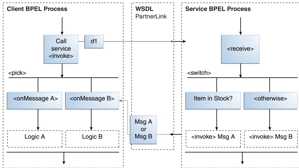
Figure 5–7 One Request, One of Two Possible Responses
