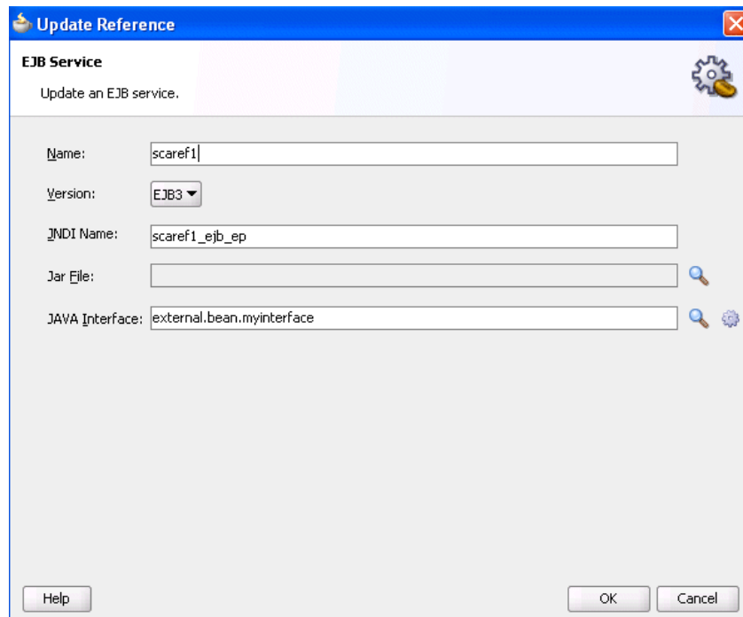
Figure 52–13 EJB Reference Dialog in External References Swimlane
