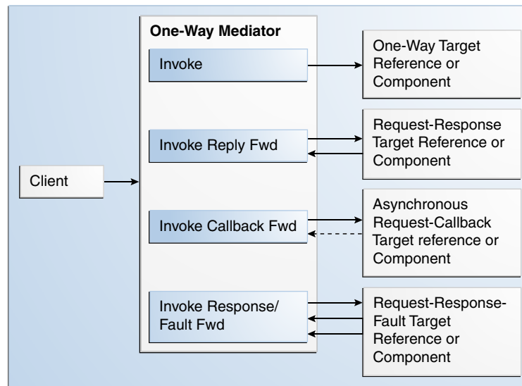
Figure 24-1 One-way Message Exchange Pattern
