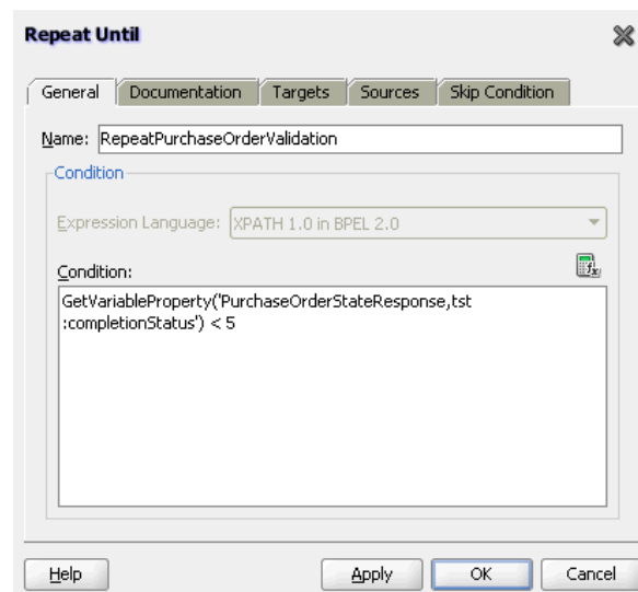
Figure 11–11 Completed Repeat Until Dialog
