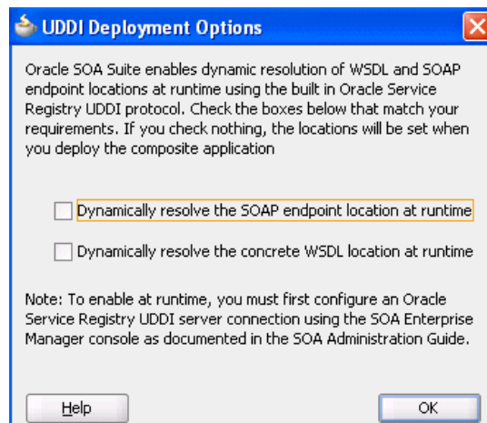
Figure A–50 UDDI Deployment Options Dialog
