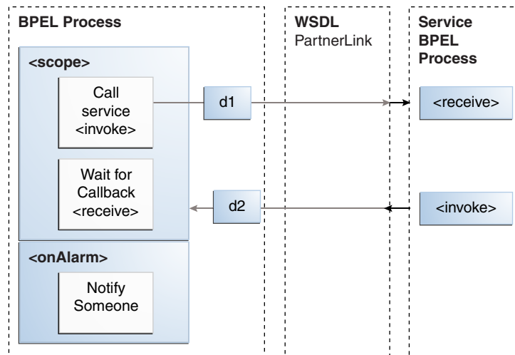
Figure 5–5 Asynchronous Interaction with a Notification Time
