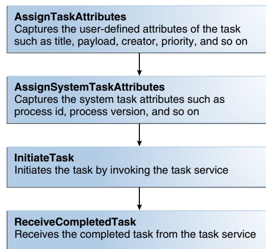
Figure 28–12 Workflow Interaction Modeling
