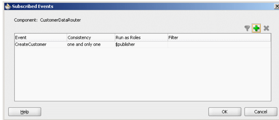
Figure 19–31 The Subscribed Events Dialog
