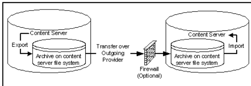
Figure 8-26 One-to-One Archiving: Over Sockets
