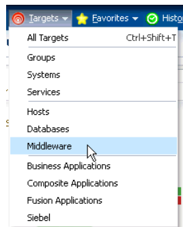
Figure 18–5 Middleware Menu
