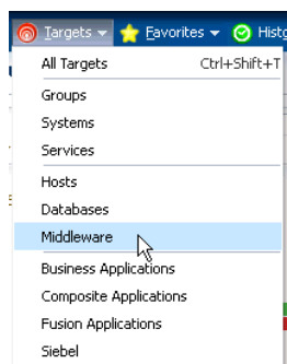
Figure 18–1 Middleware Menu
