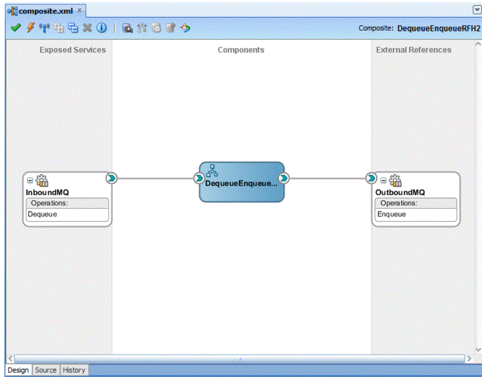
Figure 10–95 The JDeveloper - Composite.xml Page
