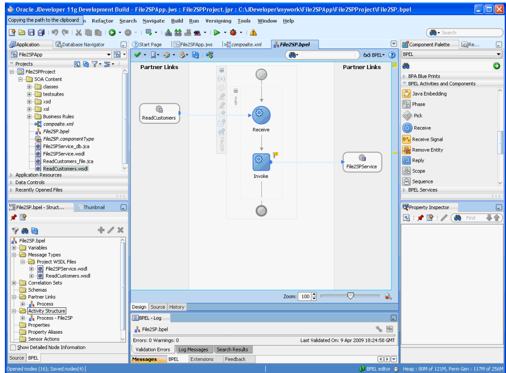
Figure 9–68 Adding a Receive Activity
