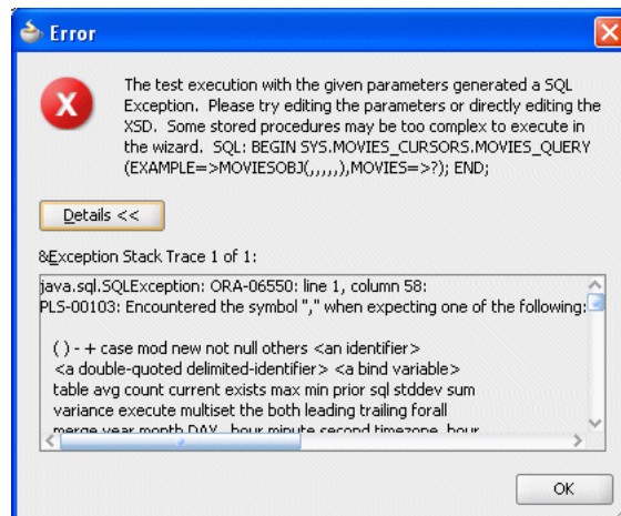
Figure 9–55 Introspection Error Dialog
