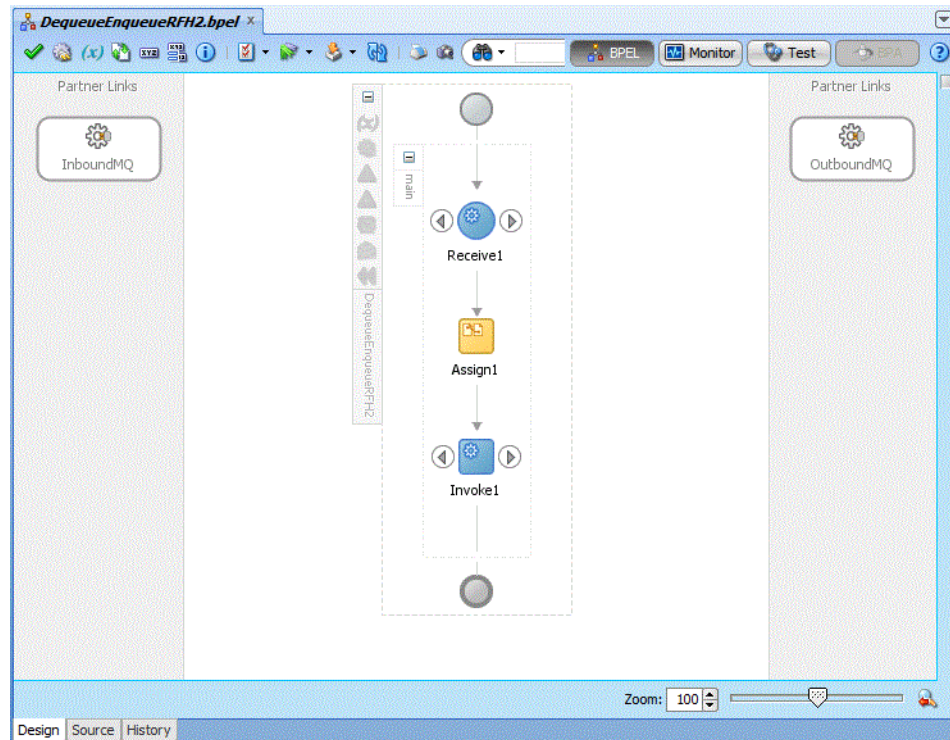
Figure 10–96 The DequeueEnqueueRFH2.bpel Page"
