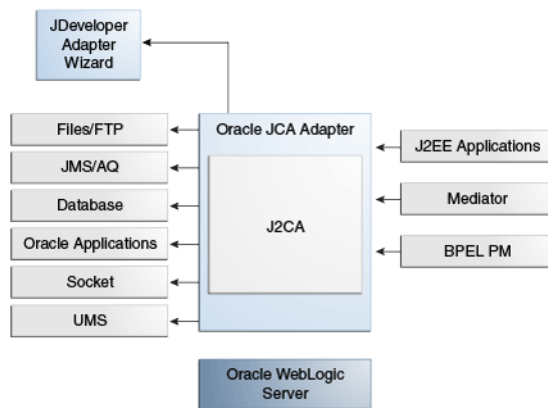
Figure 11–1 The UMS Adapter as Part of the Adapter Architecture
