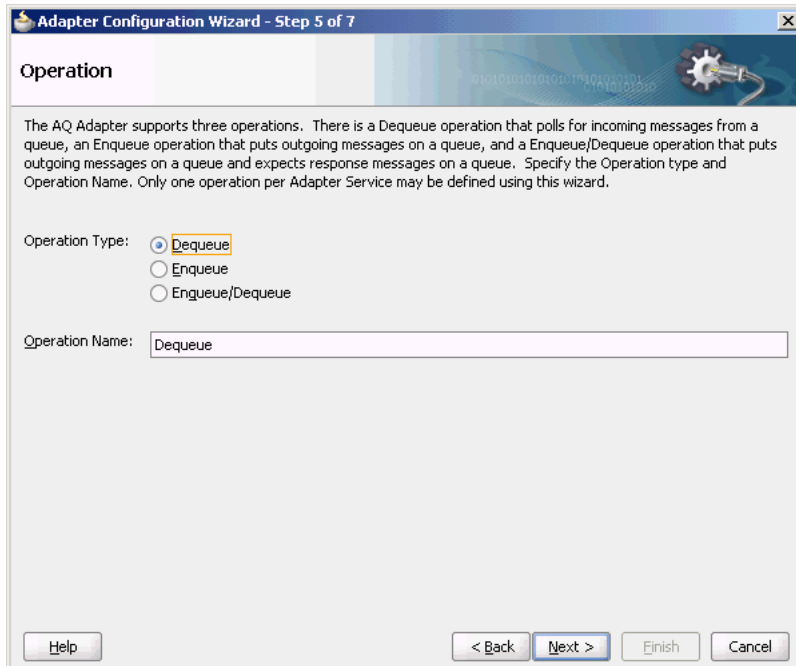
Figure 7-51 The Adapter Configuration Wizard Operation Page
