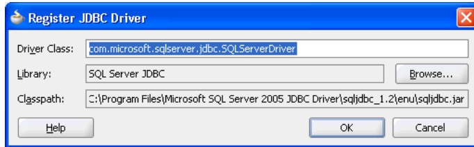
Figure 9–48 The Register JDBC Driver Dialog
