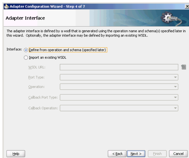
Figure 8–7 The Adapter Configuration Wizard - Adapter Interface Page
