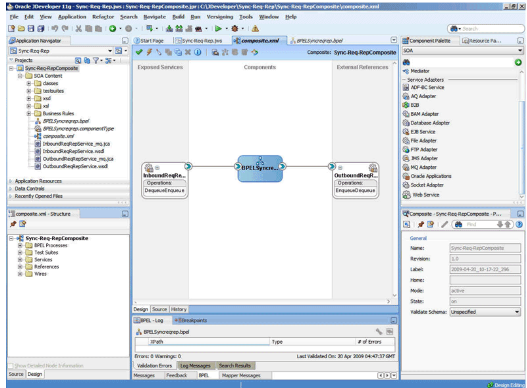
Figure 10–65 The JDeveloper - Composite.xml
