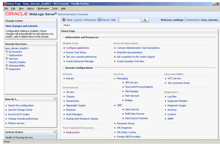
Figure 9–72 Oracle WebLogic Server Administration Console Home Page
