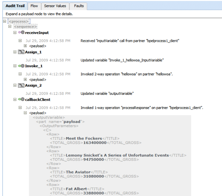
Figure 9-56 Audit Trail for Stongly Typed Payload
