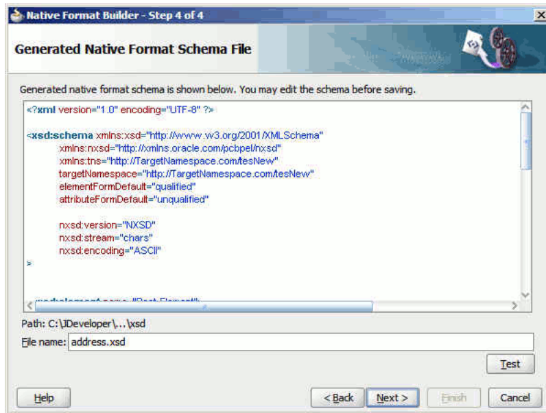
Figure 6–56 Generated Native Format Schema File Page
