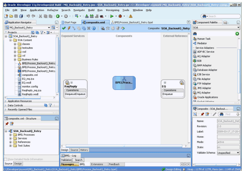
Figure 10–91 The JDeveloper Page - Composite.xml Page
