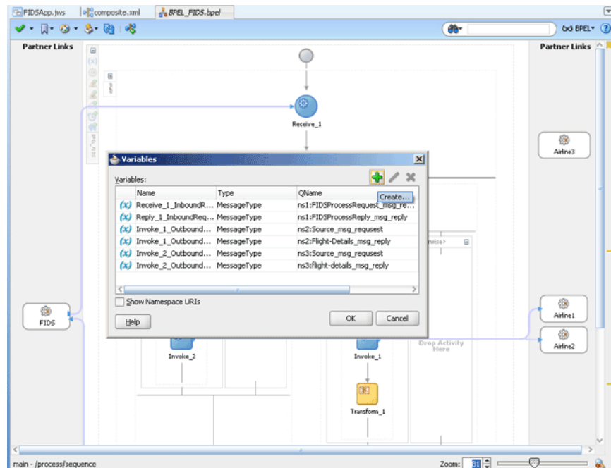
Figure 5–109 The Variables Dialog
