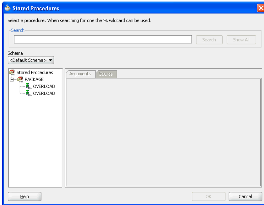
Figure 9–42 A Package with Two Overloaded Procedures
