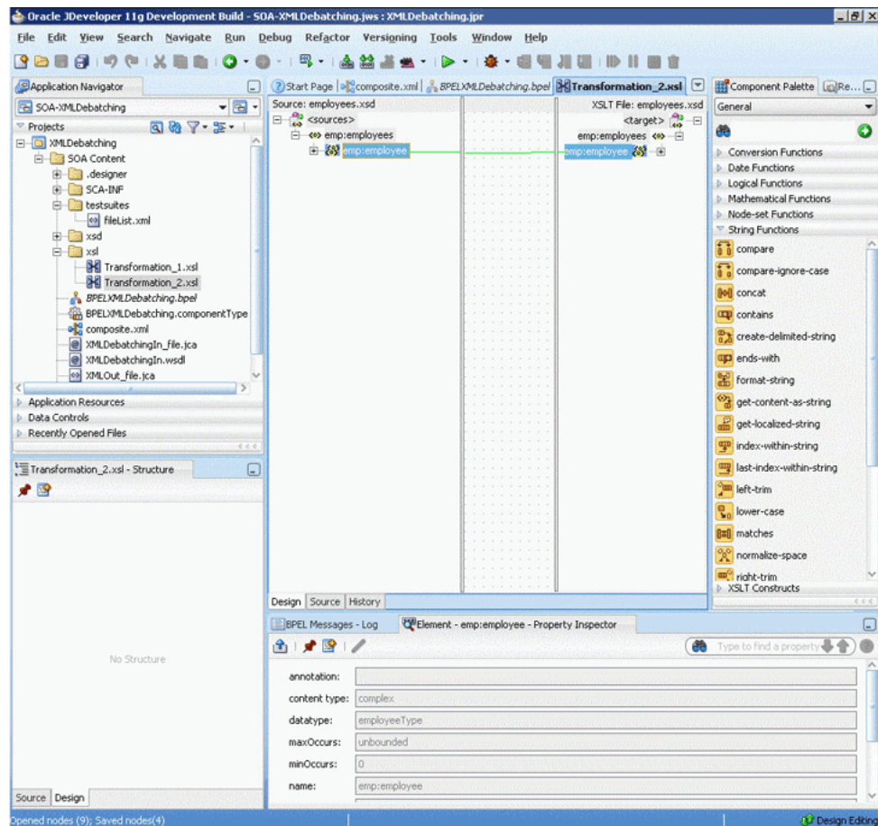
Figure 4–75 The JDeveloper - Transformation_2.xsl
