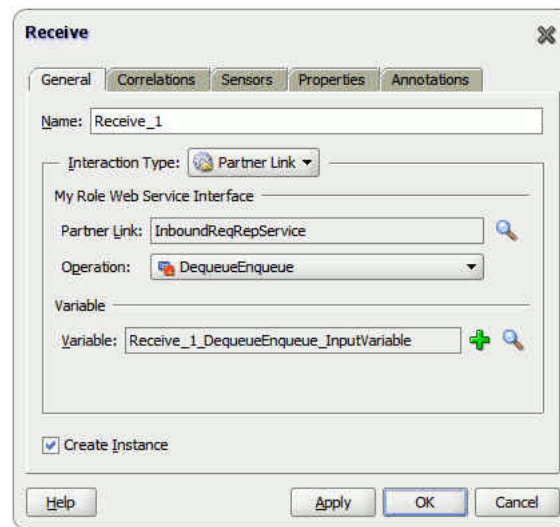
Figure 10–67 The Receive Dialog
