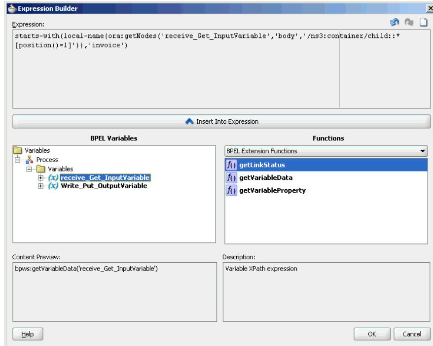
Figure 4-152 The Expression Builder Dialog
