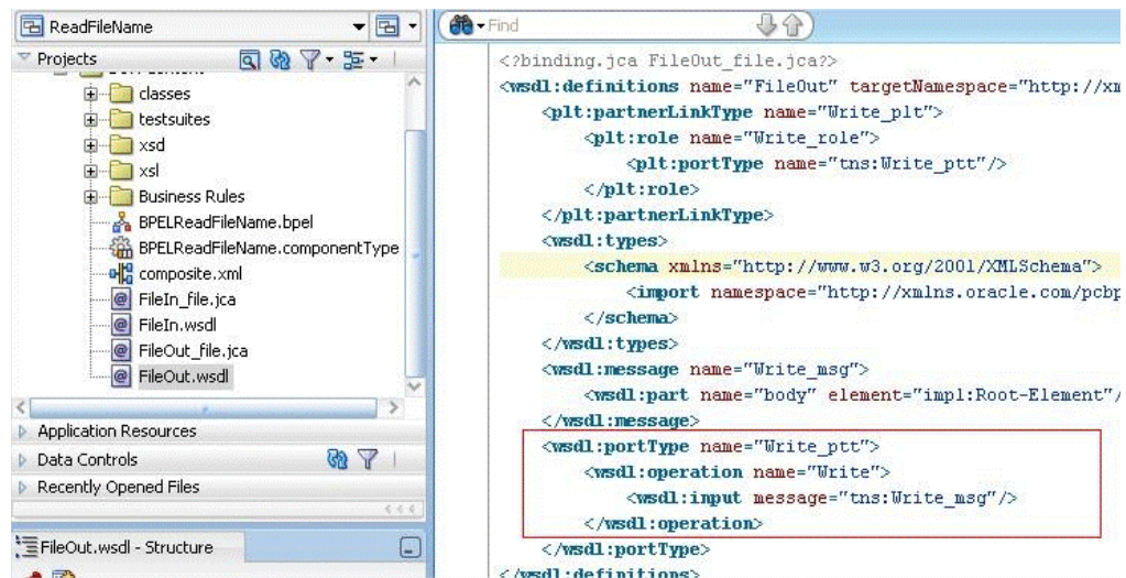
Figure 4–171 Editing the WSDL File So the File/FTP Adapter Returns File Metadata
