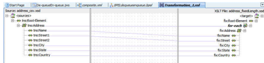
Figure 10–56 The Trasformation_xsl Page
