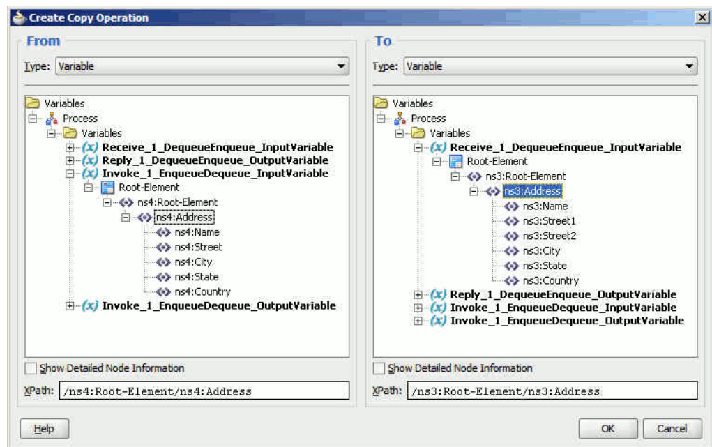
Figure 10–72 The Create Copy Operation Dialog
