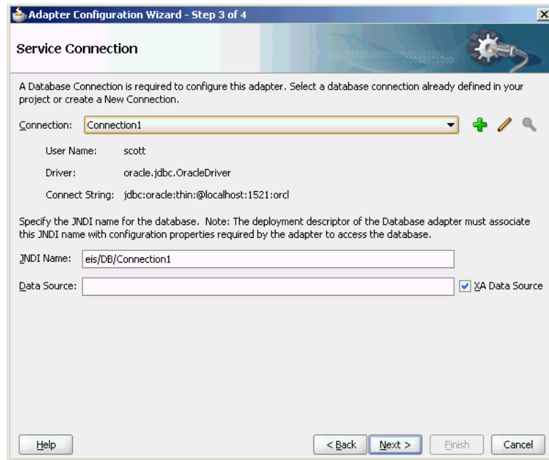
Figure 9–7 The Adapter Configuration Wizard: Service Connection Page
