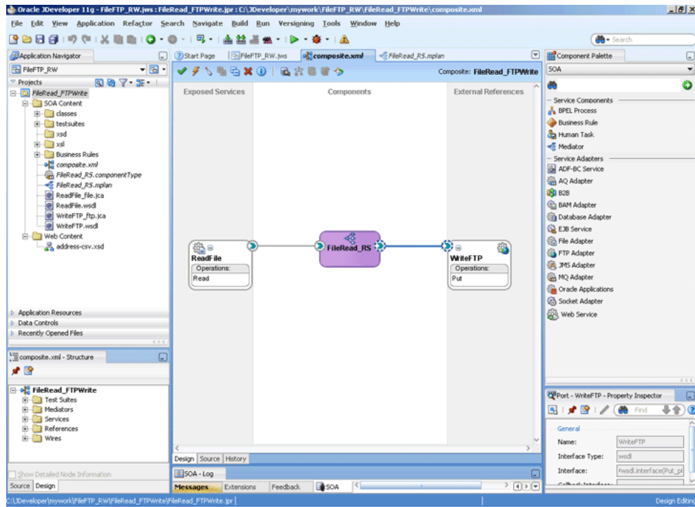
Figure 4–84 The JDeveloper - Composite.xml
