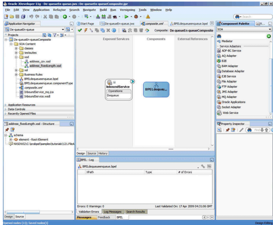
Figure 10–51 The JDeveloper Page - Composite.xml Page
