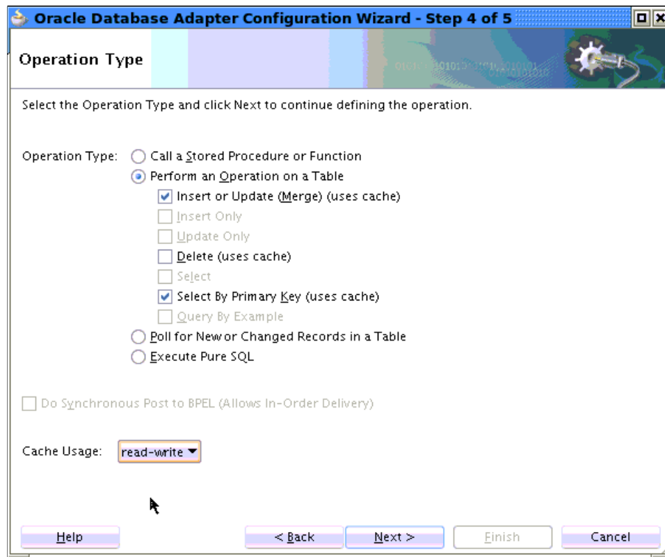
Figure 9–77 Enabling Read-Write Caching Using the Operation Type Screen
