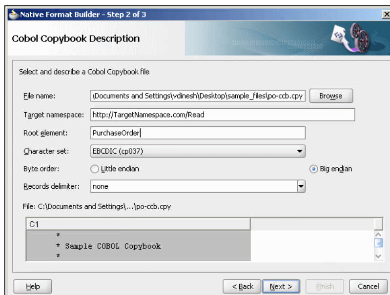
Figure 6-67 Native Format Builder Wizard File Description Page
