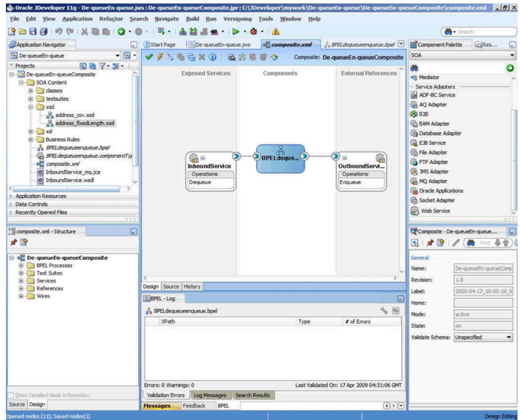
Figure 10–54 The JDeveloper - Composite.xml
