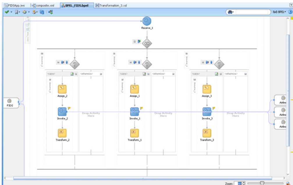
Figure 5–111 The JDeveloper - BPEL_FIDS.bpel
