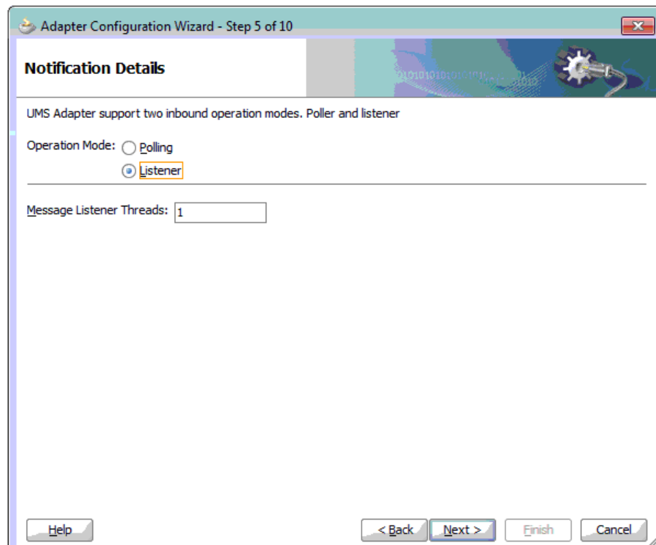
Figure 11–9 UMS Adapter Configuration Wizard Notification Details with Listener Mode Selected
