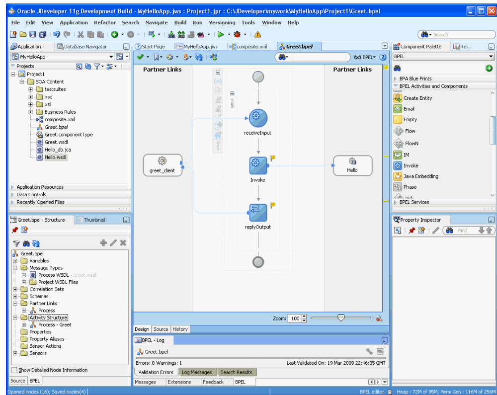
Figure 9–61 The Greet.bpel Page
