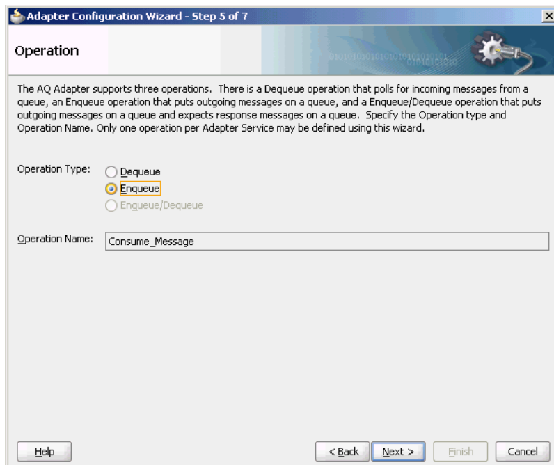
Figure 2–2 Operation Page for Oracle AQ Adapter with Fields Automatically Populated
