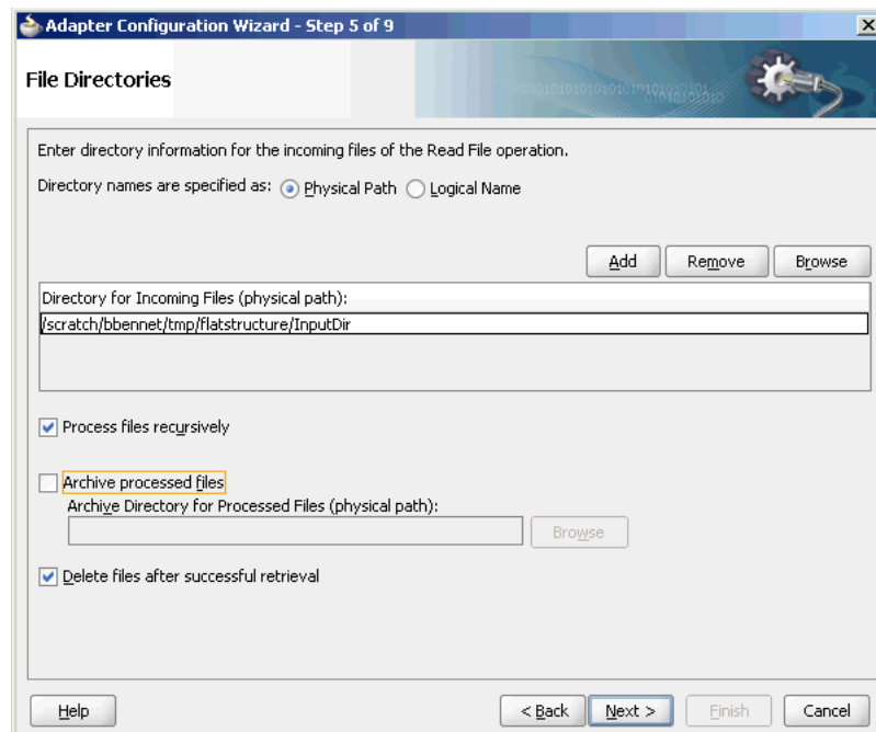
Figure 4–8 The Adapter Configuration Wizard - File Directories Page
