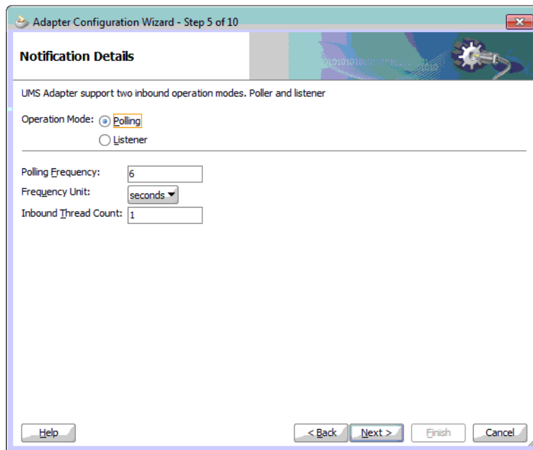
Figure 11–8 Notification Details Screen when Polling is Selected for an Inbound Receive Operation
