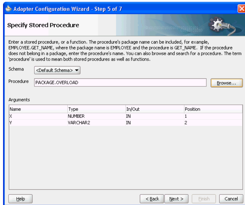
Figure 9–44 Viewing Procedure or Function Details in the Adapter Configuration Wizard
