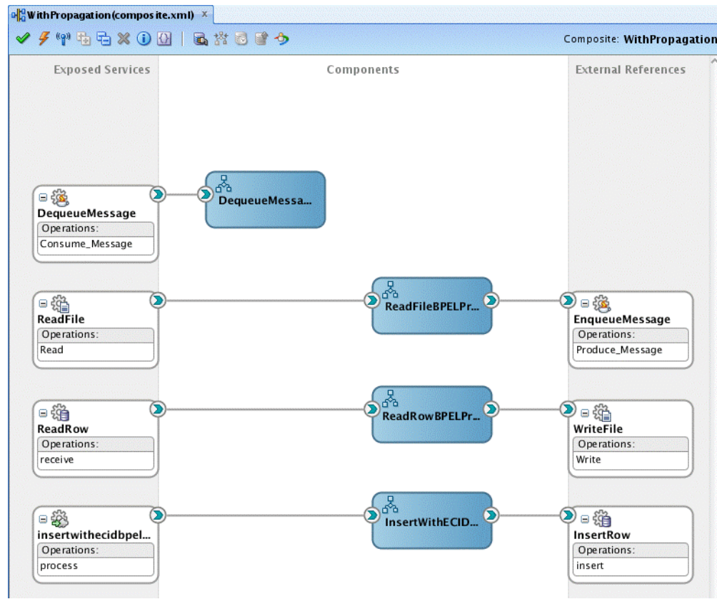
Figure 2–25 The Composite for the Example
