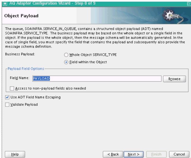
Figure 7-13 The Adapter Configuration Wizard Object Payload Page
