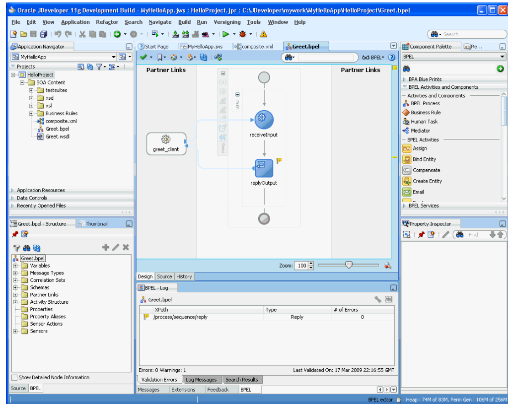
Figure 9–60 The JDeveloper - Composite.xml
