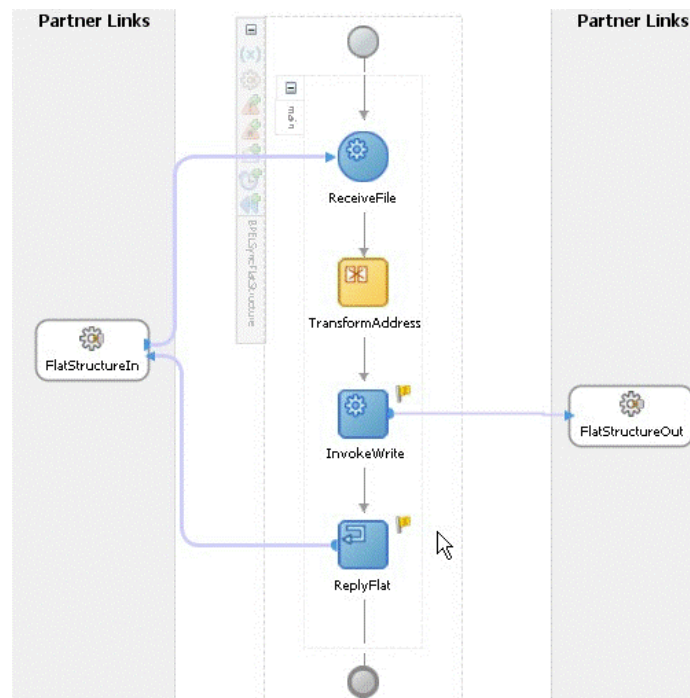
Figure 4–170 The Synchronous File Adapter Process with Receive and Reply BPEL Activities
