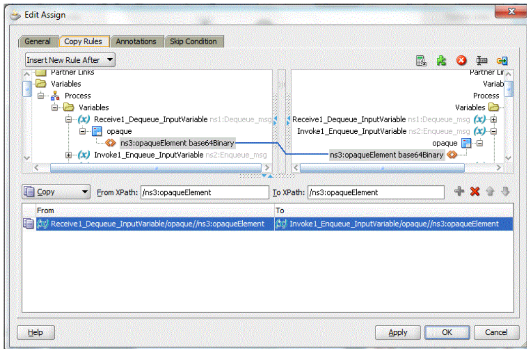
Figure 10–97 The Assign Activity Dialog
