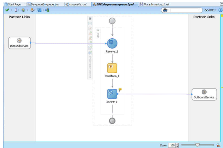
Figure 10–57 The BPELdequeueenqueue.bpel Page
