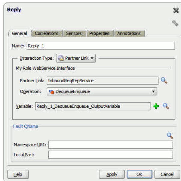
Figure 10–68 The Reply Dialog
