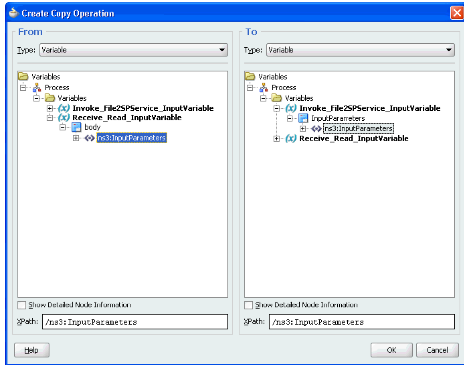
Figure 9–70 The Assign Dialog
