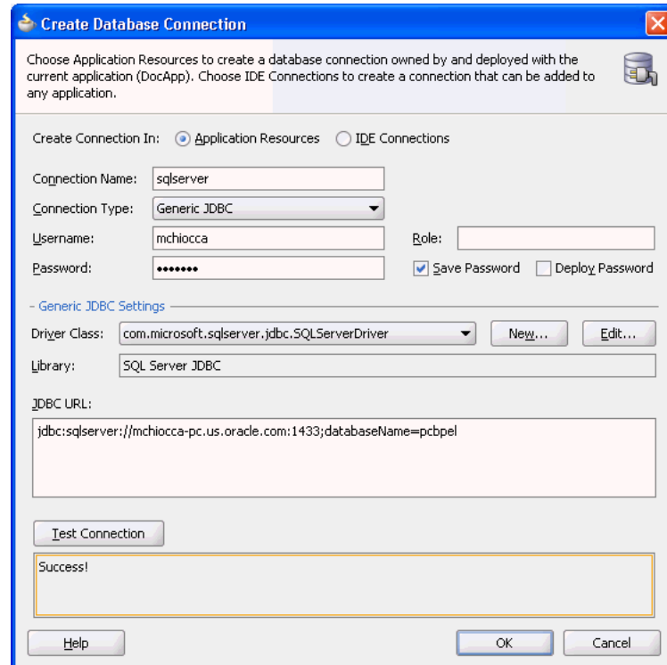
Figure 9–50 The Create Database Connection Dialog
