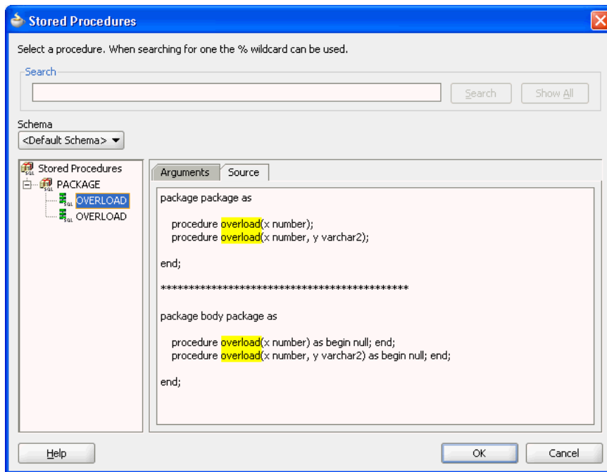
Figure 9–43 Viewing the Source Code of an Overloaded Procedure
