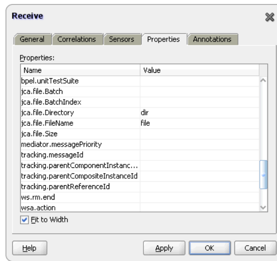
Figure 4–104 The Receive Dialog - Adapters Tab
