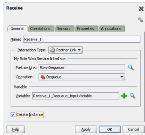
Figure 7–60 The Receive Dialog
