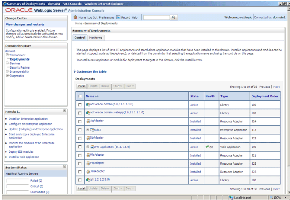
Figure 4–10 The Oracle WebLogic Server Administration Console - Summary of Deployments Page
