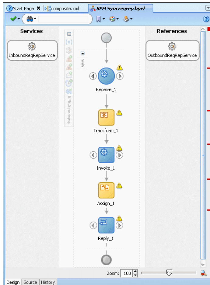
Figure 10–66 The BPELSyncreqrep.bpel Page
