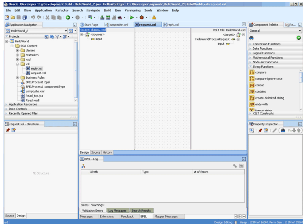
Figure 5–22 The JDeveloper - request.xsl Page
