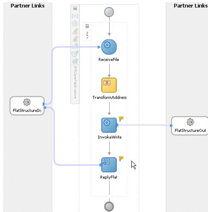
Figure 4–180 The Synchronous BPEL Process
