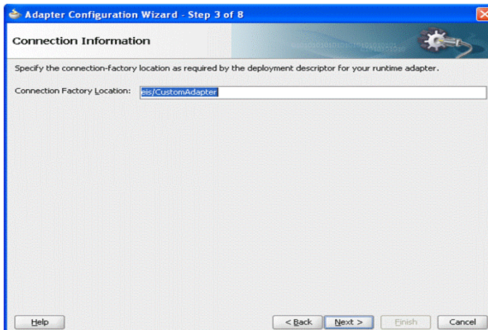
Figure 2–18 Adapter Configuration Wizard Connection Information Screen
