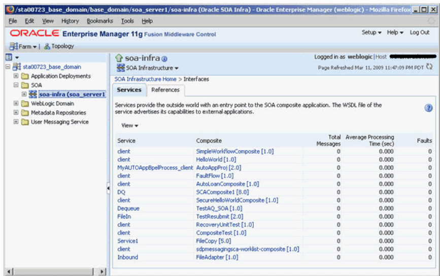
Figure 3–11 The SOA Infrastructure Home > Interfaces Page
