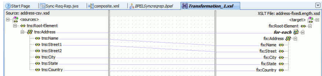
Figure 10–71 The Transformation.xsl Page with Mappings
