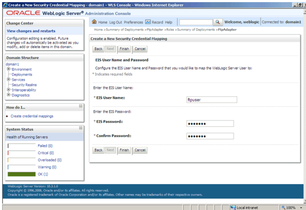
Figure 4–17 The Oracle WebLogic Server Administration Console - Create a New Security Credential Mapping Page
