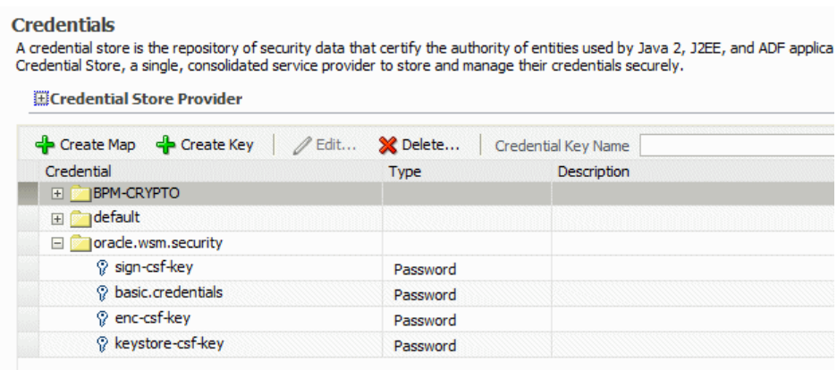
Figure 10–6 Keys Configured in Oracle WSM Credential Map
