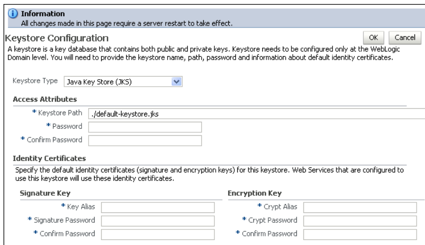
Figure 10–3 Web Services Manager Keystore Configuration
