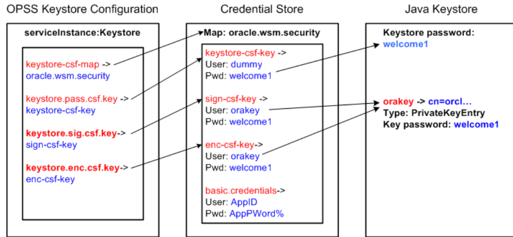
Figure 10–8 Oracle WSM Keystore Configuration for Message Protection
