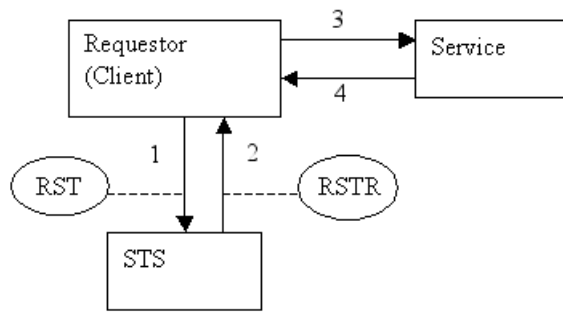
Figure 10–19 STS Use Case Message Flow
