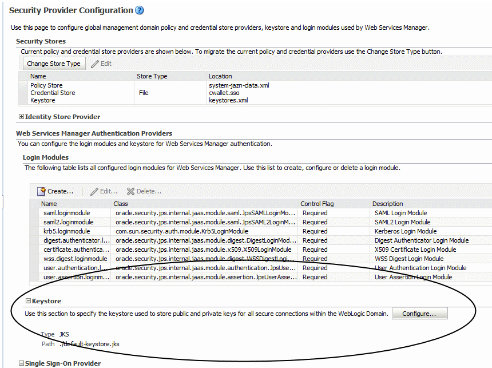
Figure 10–2 Security Provider Configuration Page
