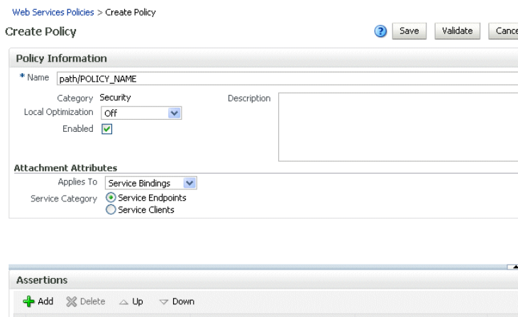
Figure 11-4 Local Optimization Control When Creating a Policy
