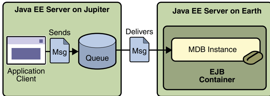
FIGURE 32–3 A Java EE Application That Consumes Messages from a Remote Server
