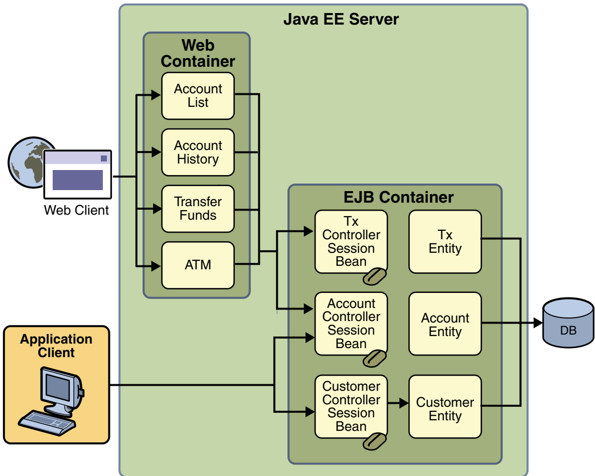
FIGURE 37-1 Duke's Bank Application
