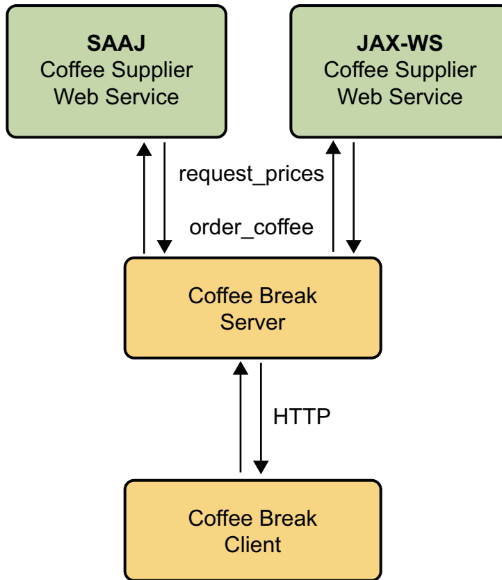
FIGURE 36-1 Coffee Break Application Flow
