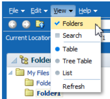
Figure 15–17 Grouped Menu Items Using the Type Attribute
