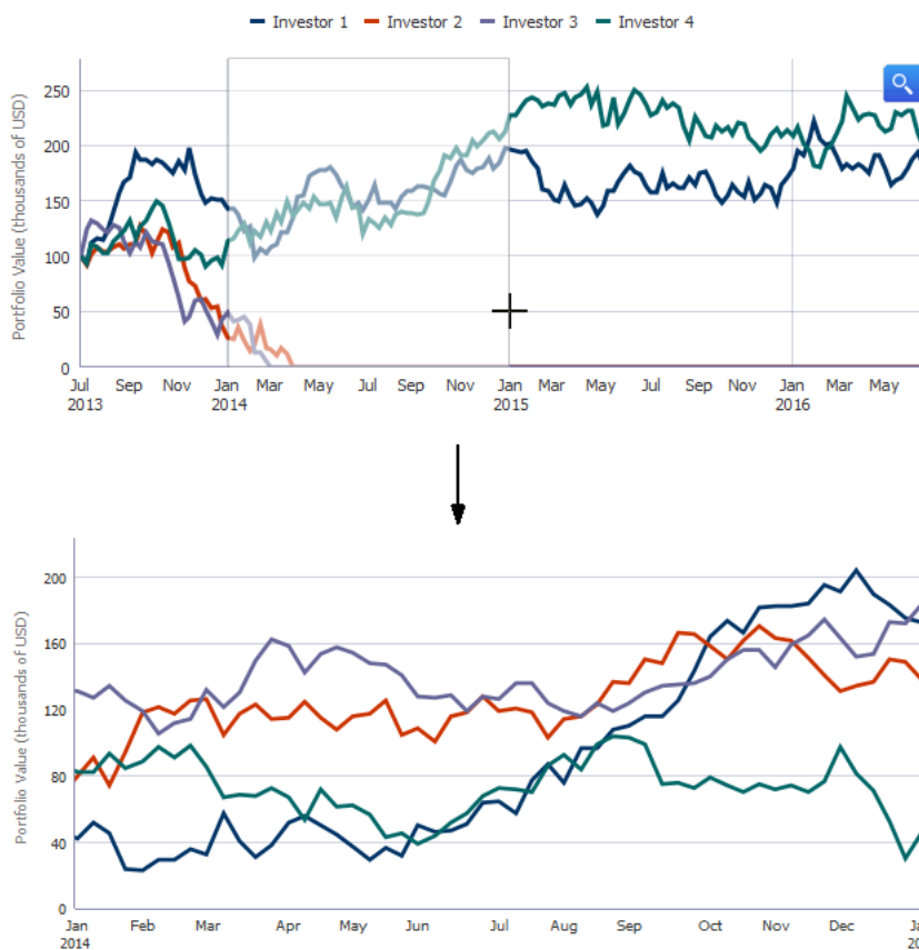
Figure 23–52 Line Chart Configured for Marquee Zoom and Scroll
