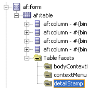
Figure 12–27 detailStamp Facet in the Structure Window
