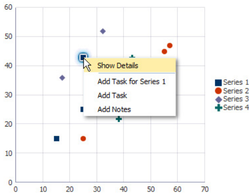
Figure H-10 Selected Marker Context Menu in Scatter Graph
