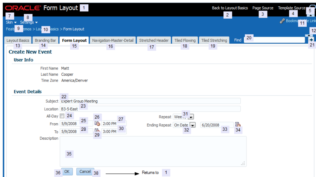
Figure C-1 Tab Traversal Sequence on a Page
