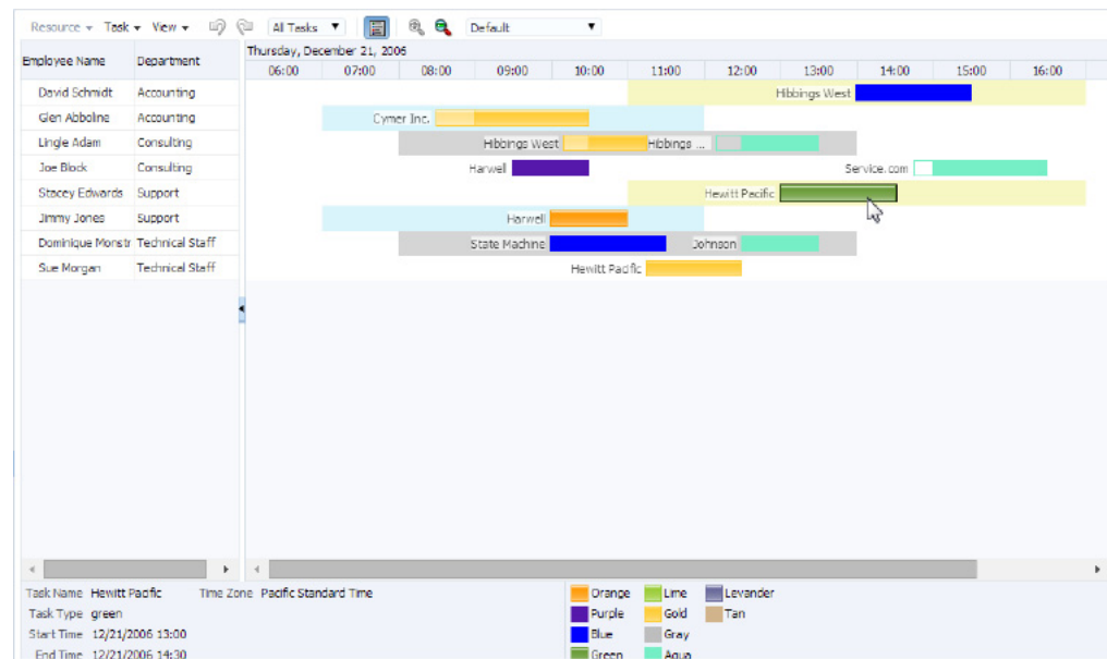
Figure 26–20 Scheduling Gantt Chart with Background Bars
