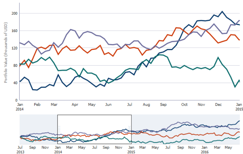
Figure 23–53 Line Chart Configured With Overview
