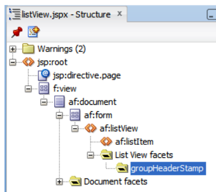
Figure 12–37 The groupHeaderStamp Facet in the Structure Window
