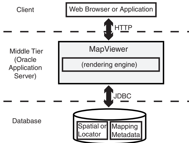
Figure 1–2 MapViewer Architecture
