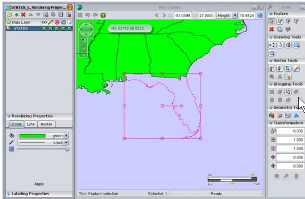
Figure 8–5 Feature Selected
