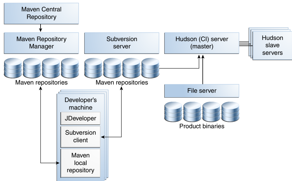
Figure 2–1 Reference Continuous Integration Environment Architecture
