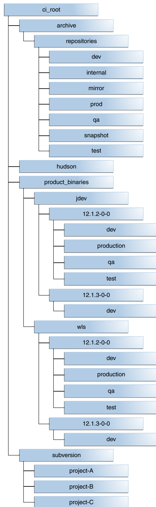
Figure 2-2 Directory Structure for a Shared Disk
