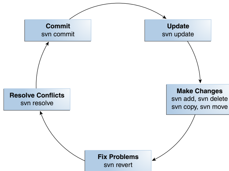
Figure 3–1 SVN Workflow
