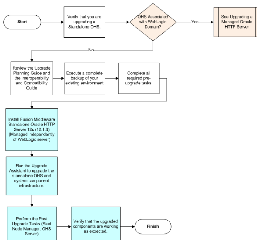
Figure 1–2 Standalone Oracle HTTP Server Upgrade from 11g to 12.1.3
