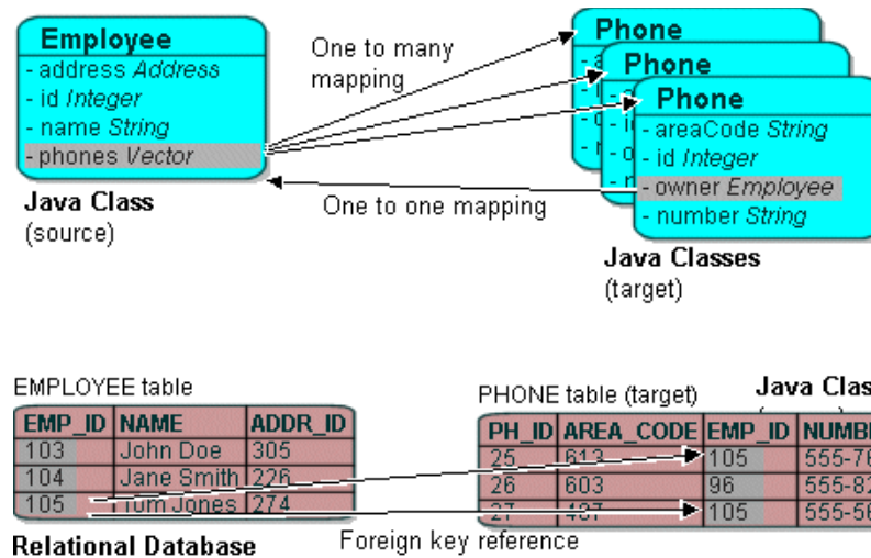
Figure 6–12 One-to-Many Relationships
