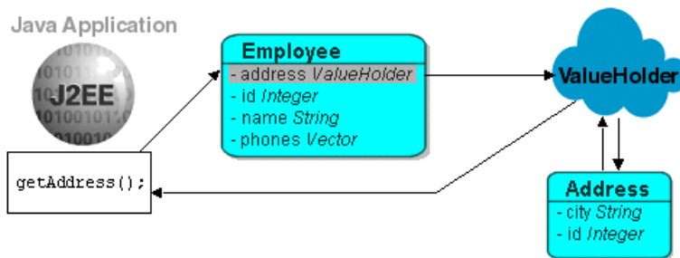
Figure 6–11 Subsequent Requests
