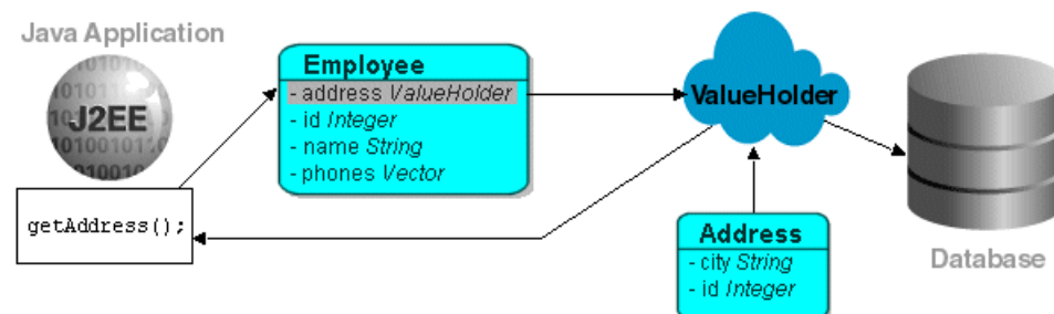
Figure 6–10 Initial Request
