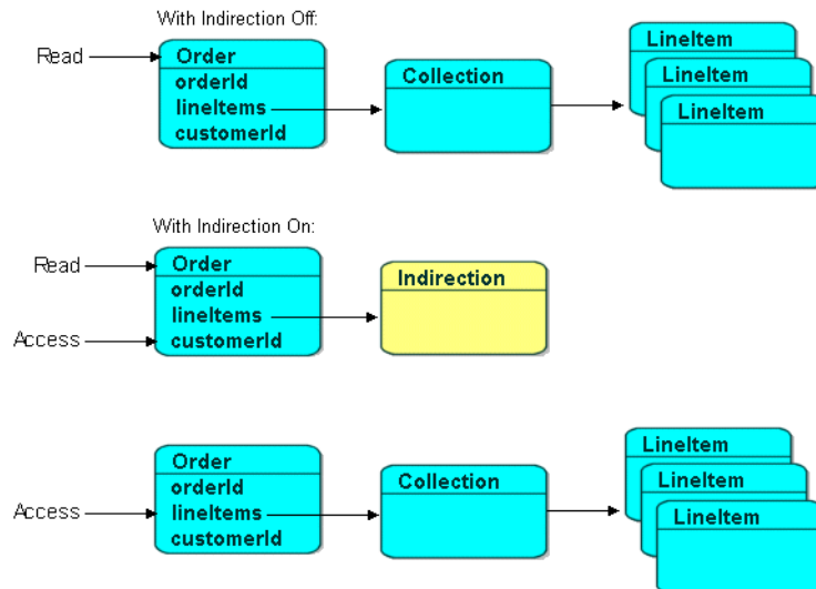
Figure 6–8 EclipseLink Indirection
