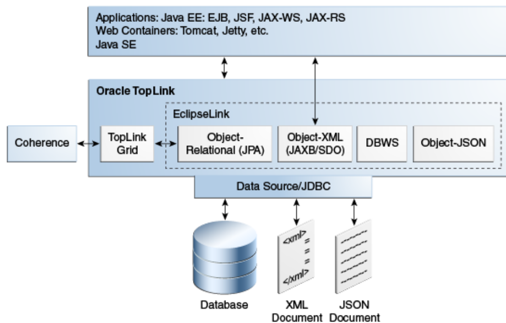
Figure 1-1 TopLink Components
