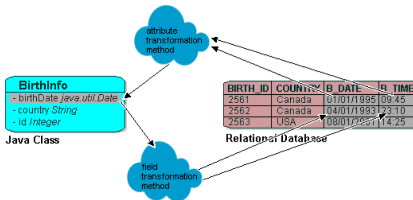
Figure 6–7 Transformation Mappings
