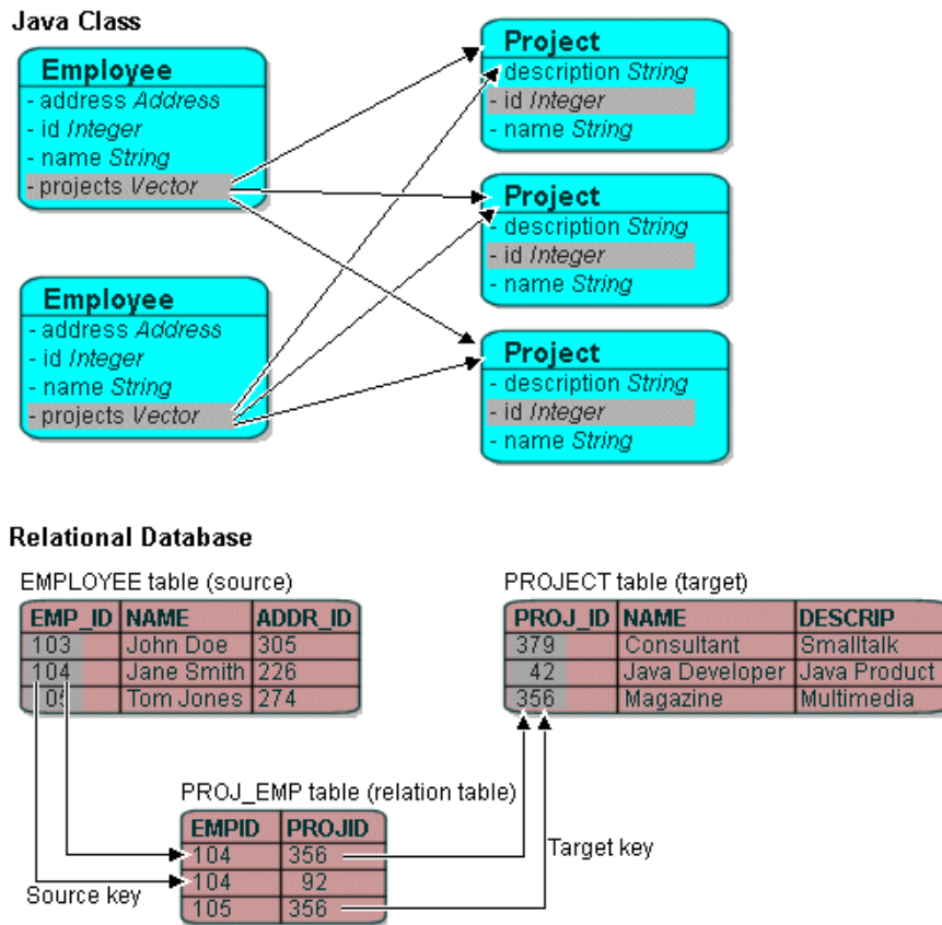
Figure 6–13 Many-to-Many Relationships
