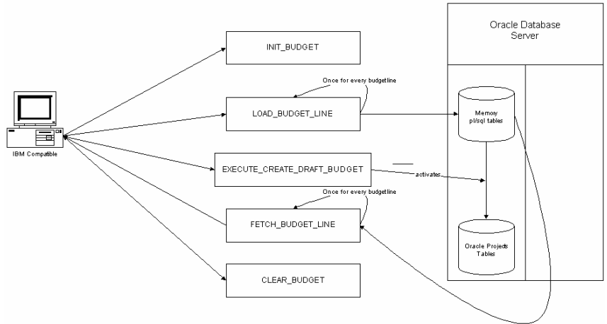
Figure 3-3: Load-Execute-Fetch Procedures for Budget APIs
