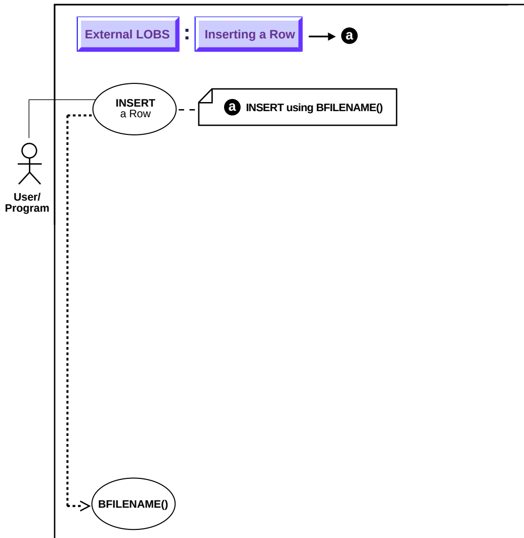
Figure 12–7 Use Case Diagram: INSERT a Row Using BFILENAME()
