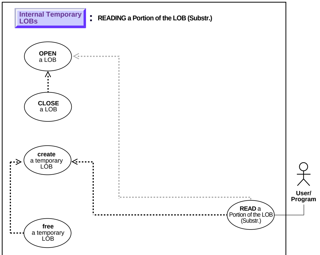
Figure 11-10 Use Case Diagram: Reading Portion of Temporary LOB from the Table (Substr)
