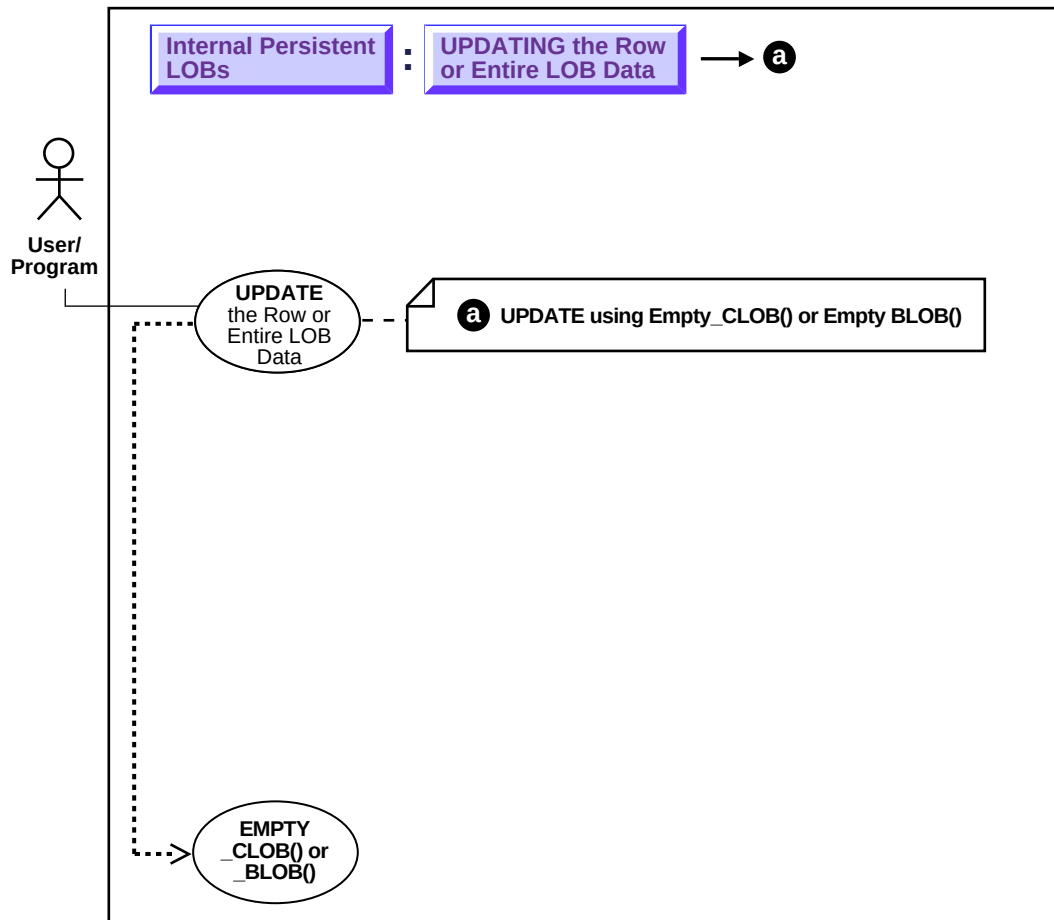
Figure 10–44 Use Case Diagram: Updating a LOB with EMPTY_CLOB() or EMPTY_BLOB()
