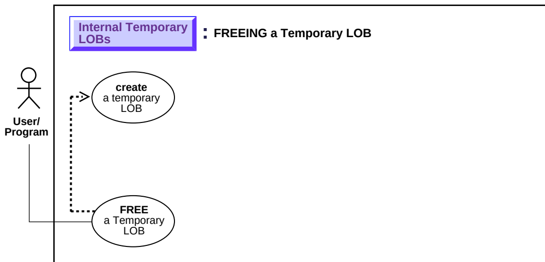
Figure 11-5 Use Case Diagram: Freeing a Temporary LOB
