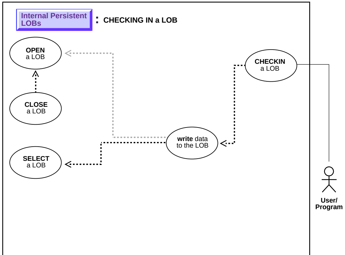
Figure 10–22 Use Case Diagram: Checking In a LOB
