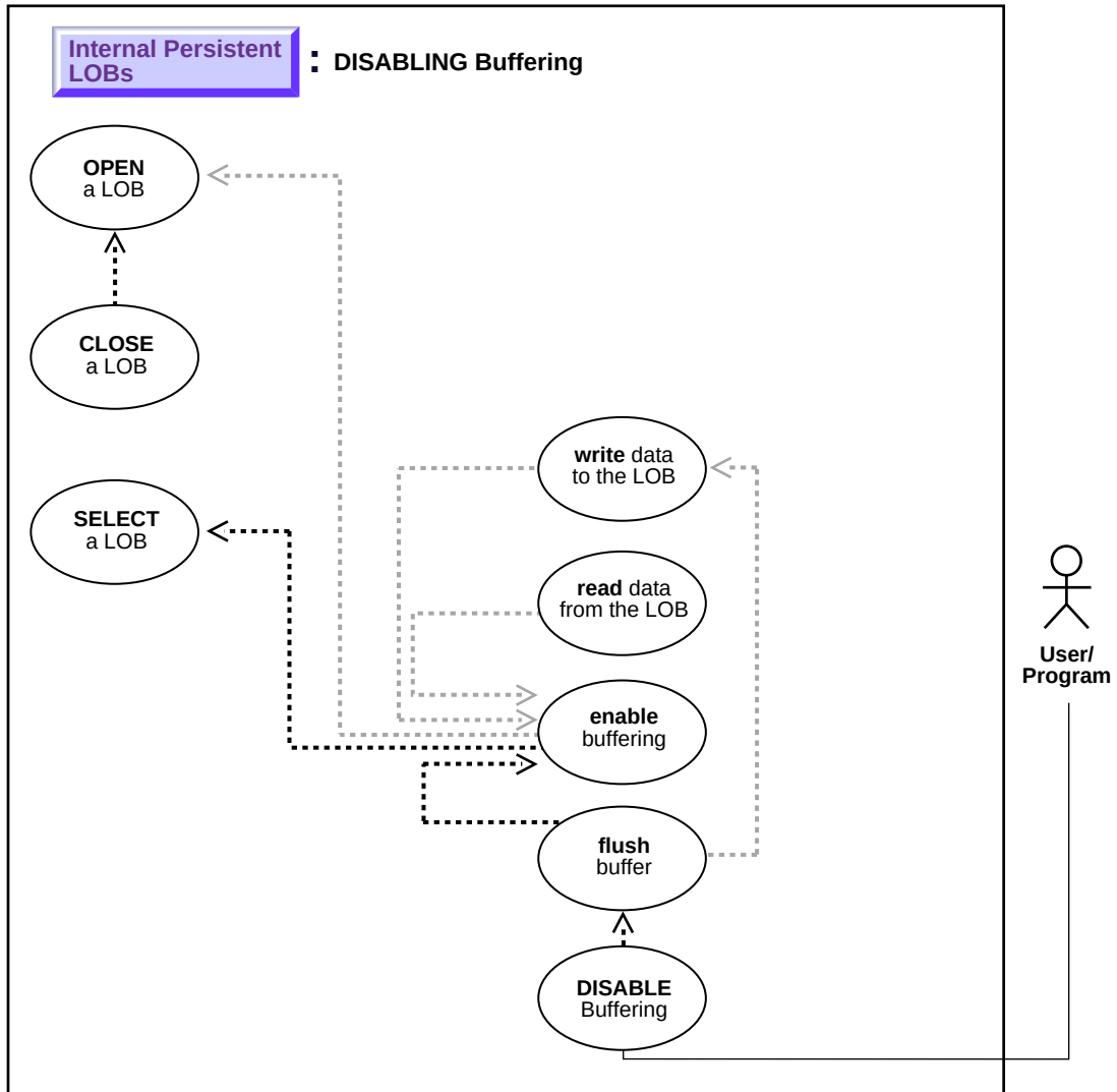
Figure 10-42 Use Case Diagram: Disabling LOB Buffering
