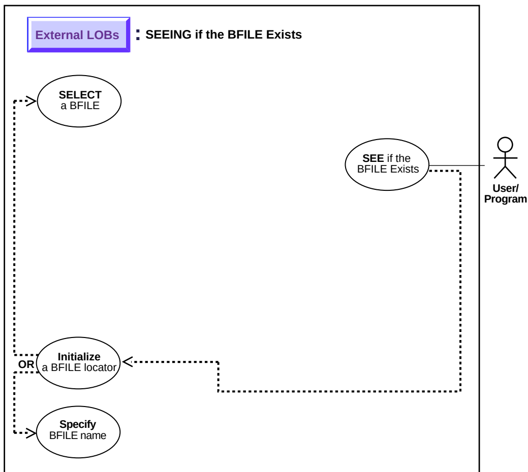
Figure 12–23 Use Case Diagram: Checking If the BFILE Exists
