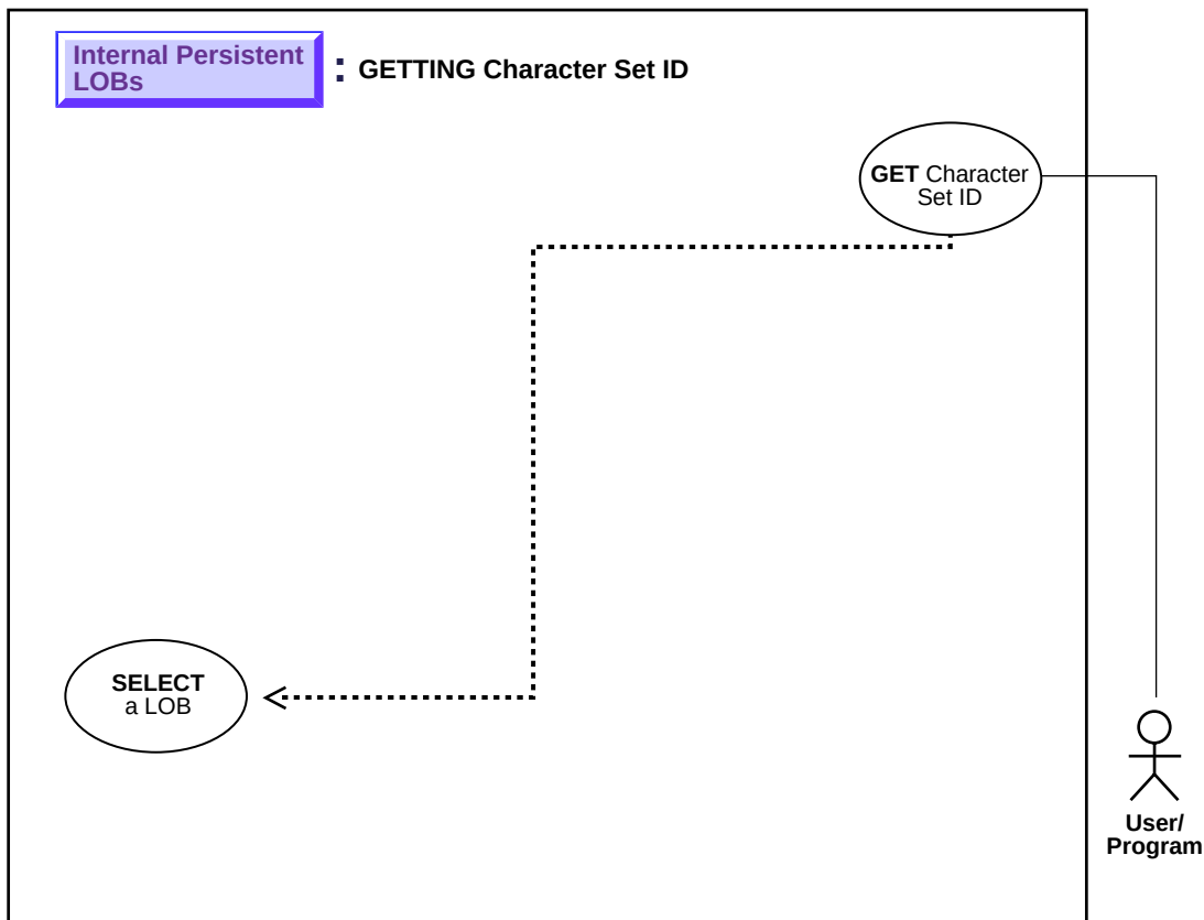
Figure 10–33 Use Case Diagram: Determining Character Set ID
