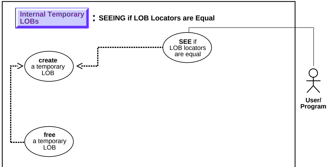
Figure 11–16 Use Case Diagram: Is One (Temporary) LOB Locator Equal to Another
