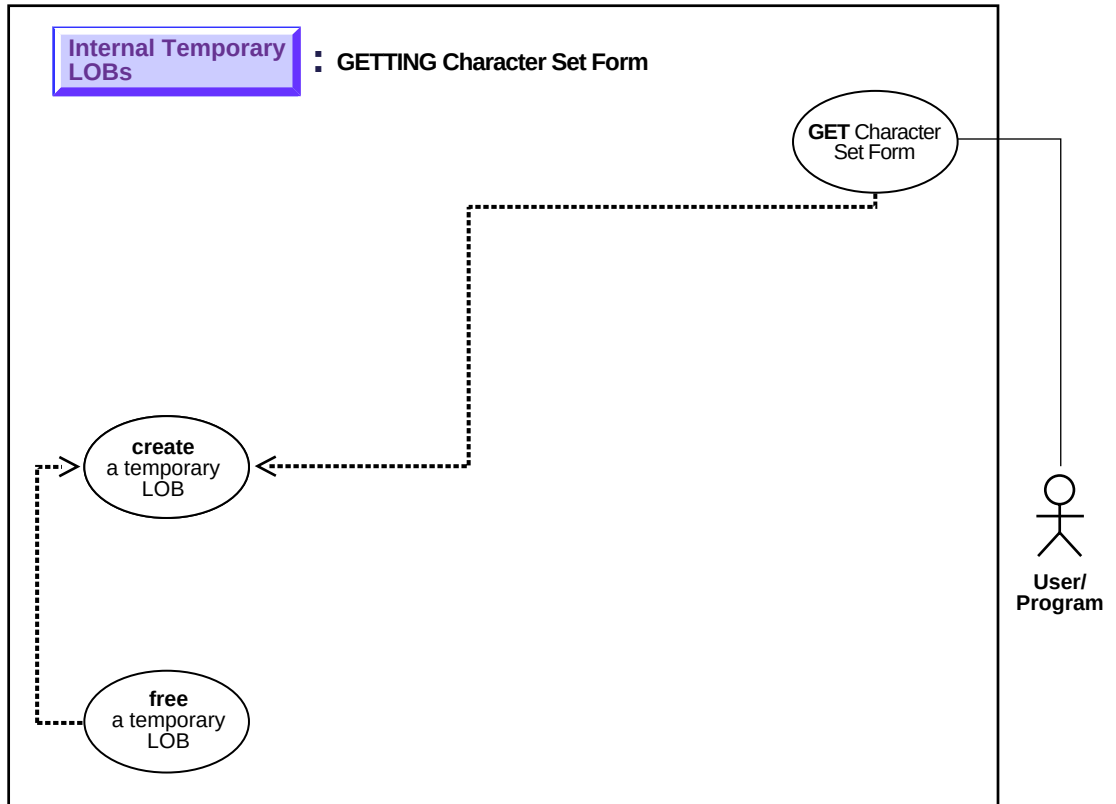
Figure 11-19 Use Case Diagram: Finding Character Set Form of a Temporary LOB
