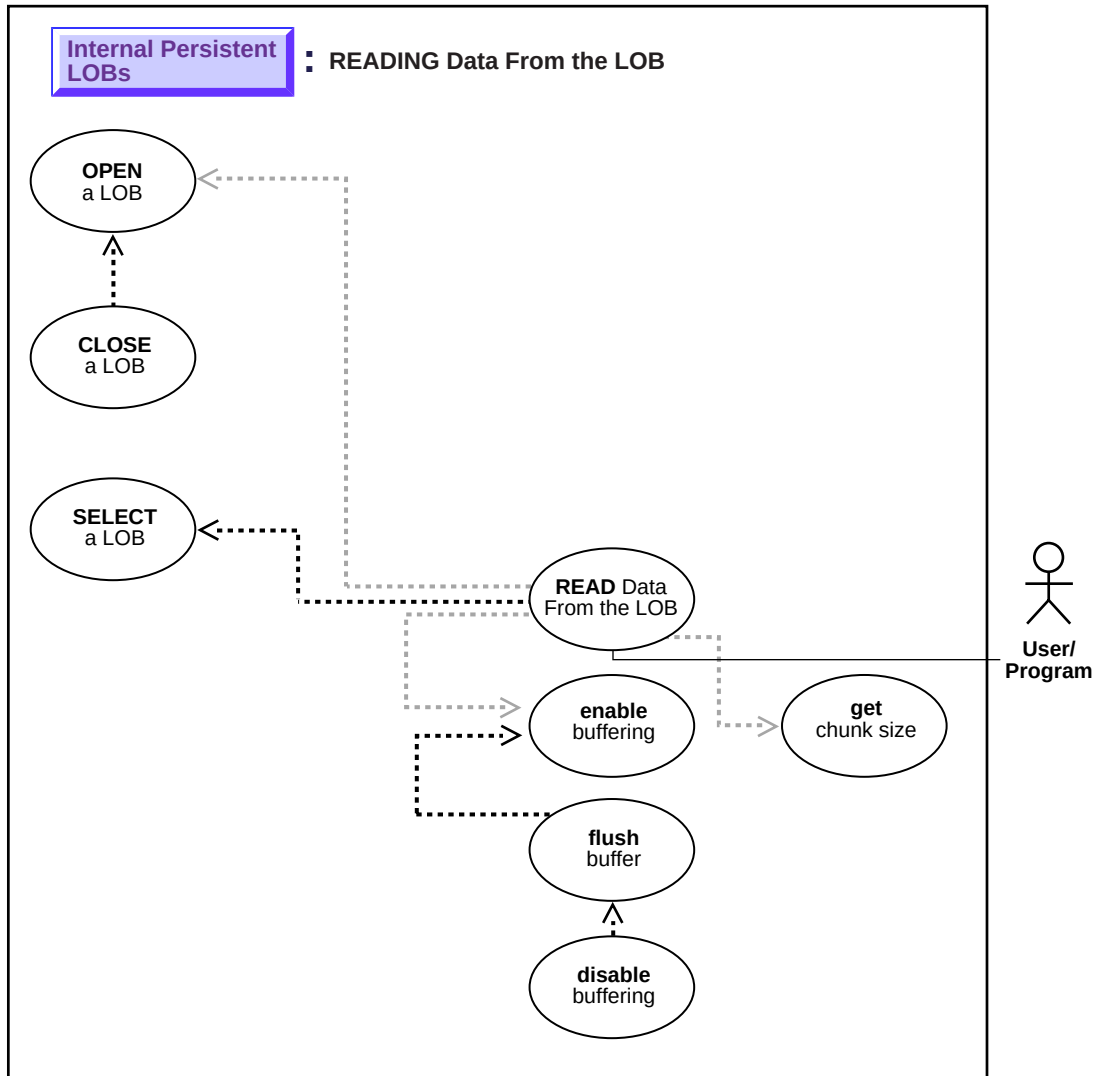
Figure 10–24 Use Case Diagram: Reading Data from a LOB
