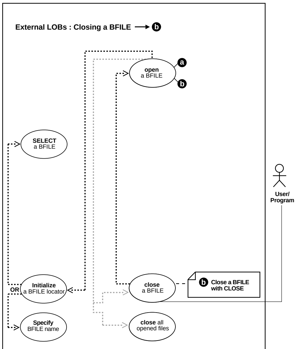
Figure 12–35 Use Case Diagram: Closing an Open BFILE with CLOSE
