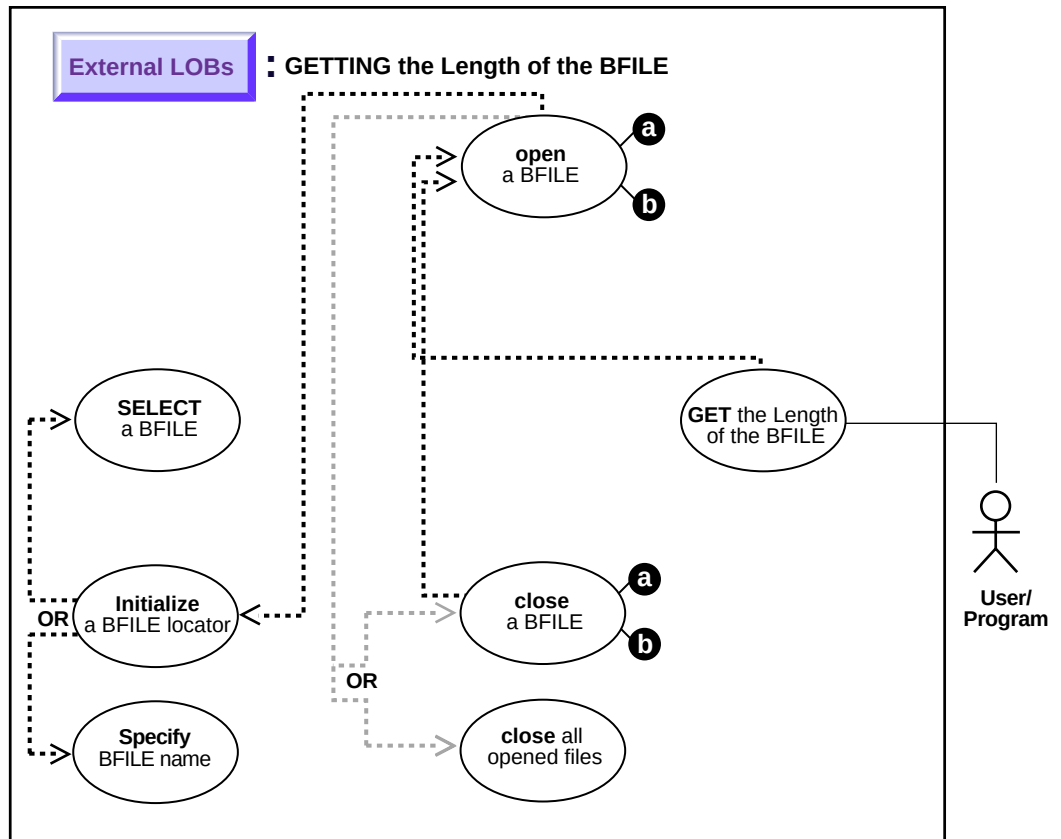
Figure 12–24 Use Case Diagram: Getting the Length of a BFILE
