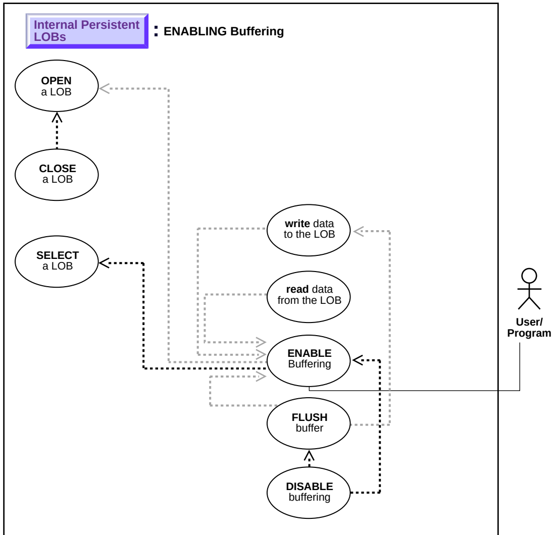
Figure 10-40 Use Case Diagram: Enabling LOB Buffering
