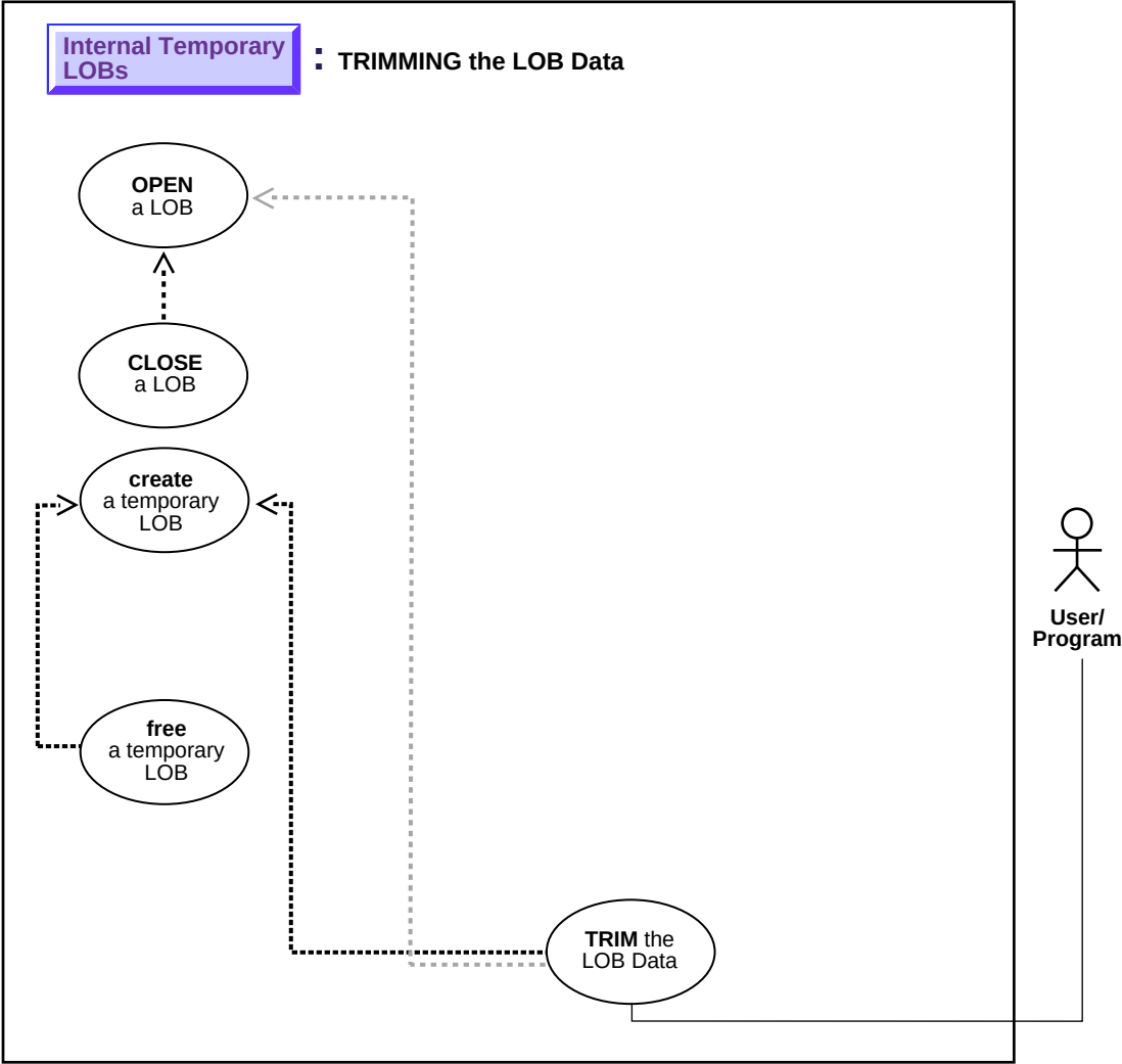
Figure 11-23 Use Case Diagram: Trimming Temporary LOB Data
