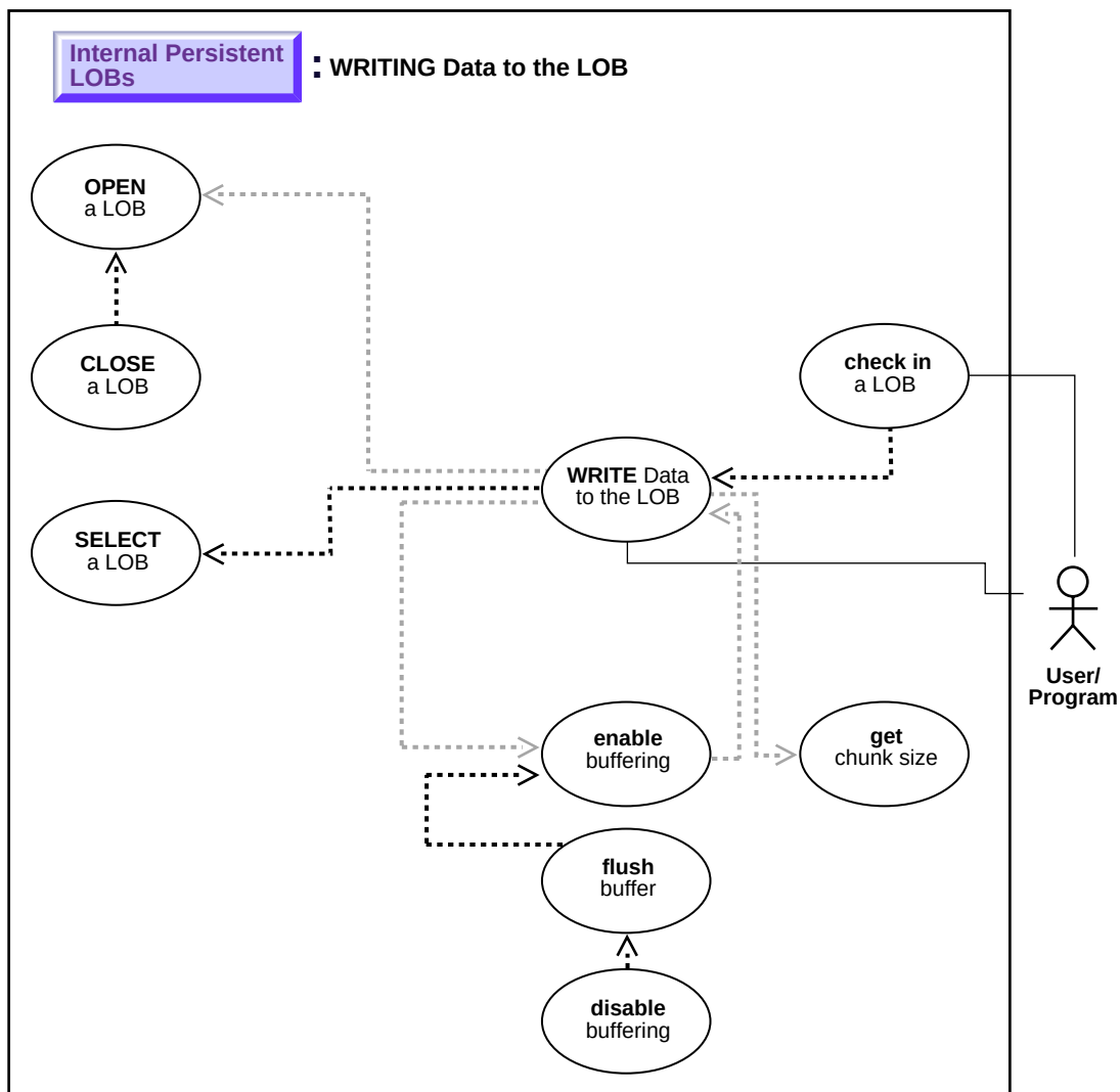
Figure 10–37 Use Case Diagram: Writing Data to a LOB
