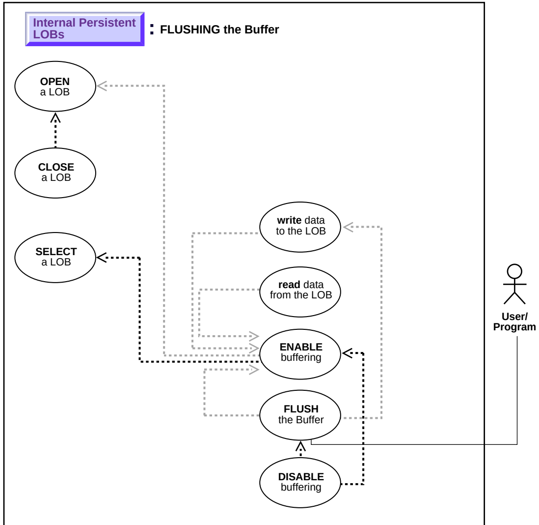
Figure 10-41 Use Case Diagram: Flushing the Buffer
