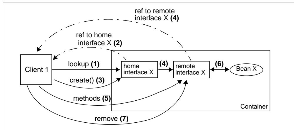
Figure 2-1 Sequence of events in a session bean lifecycle
