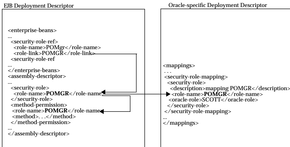
Figure A-4 Security Mapping
