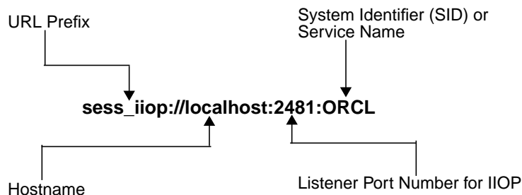
Figure 5-1 Service URL
