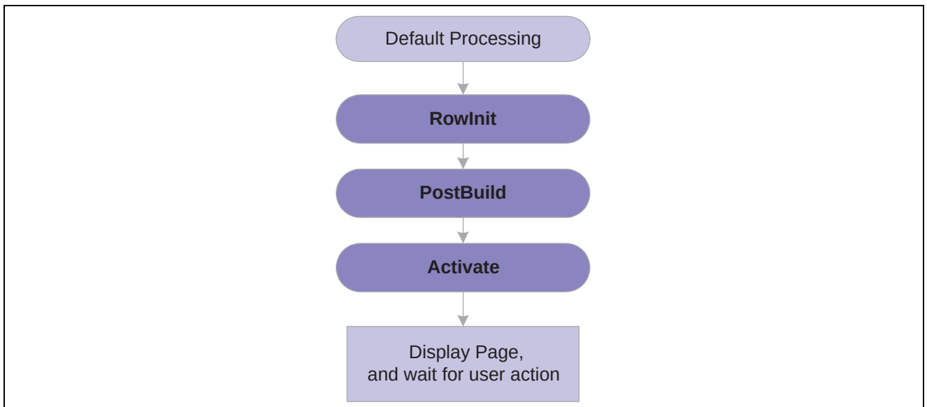
Logic of component build processing in add modes
