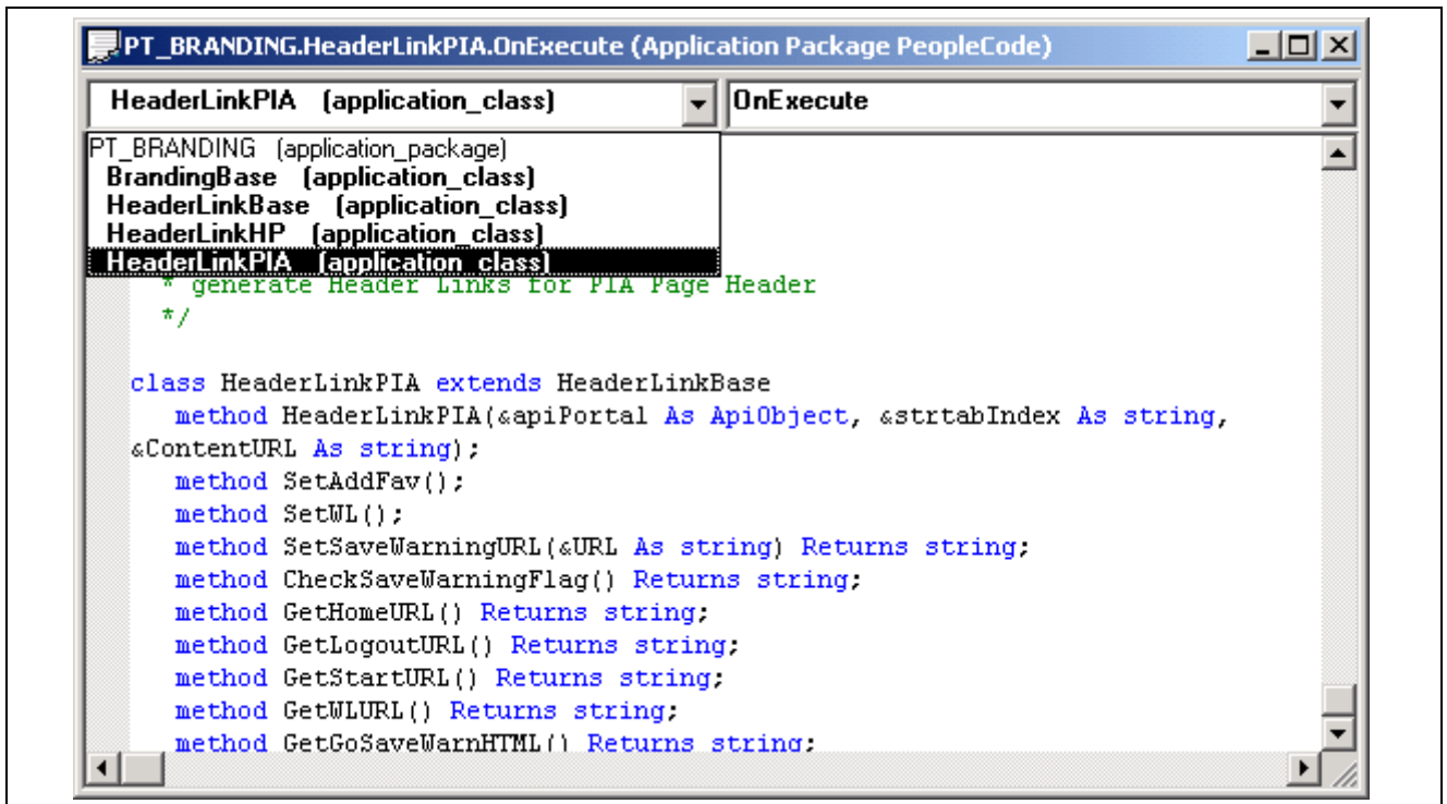
Application Packages Editor window
