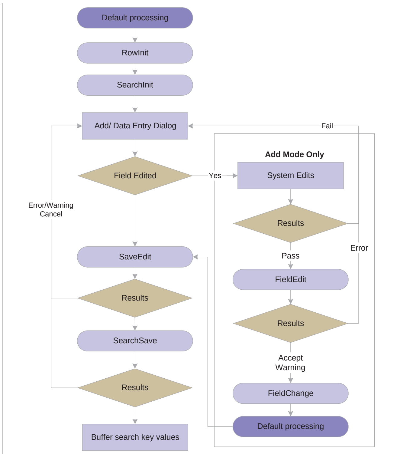
Search processing logic in add and data-entry modes
