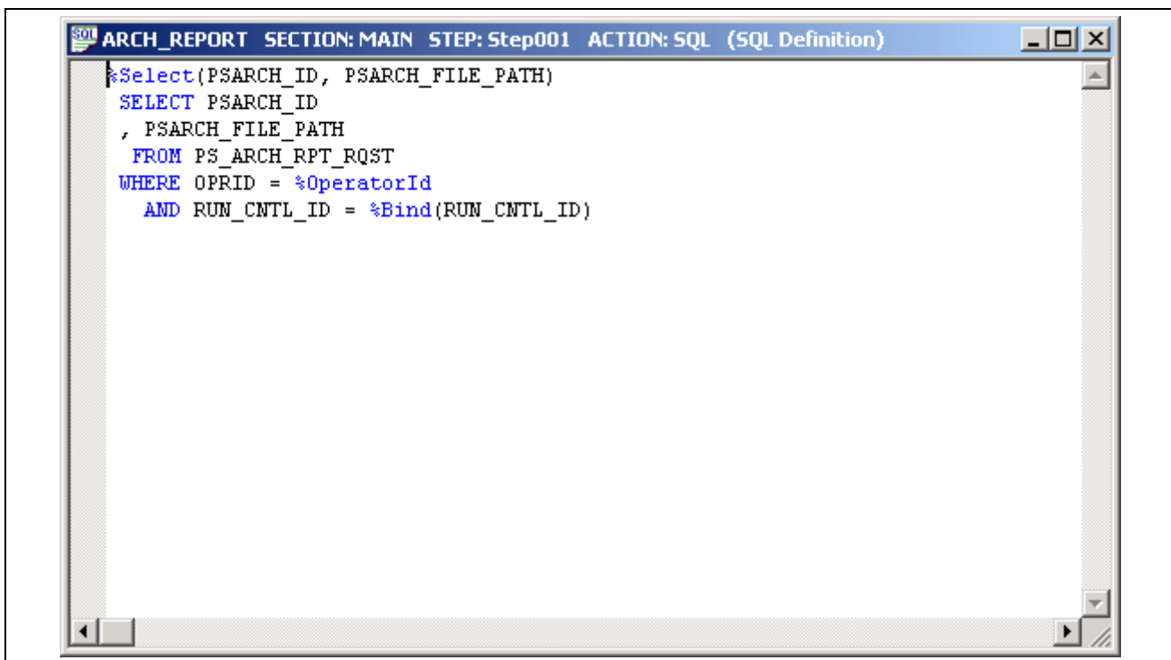
Application Engine SQL Editor window
