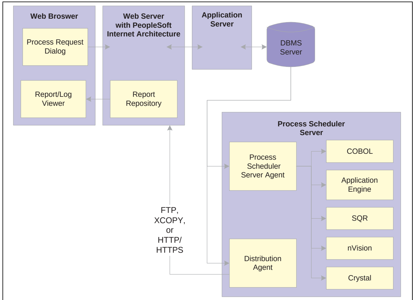
PeopleSoft Process Scheduler Architecture
