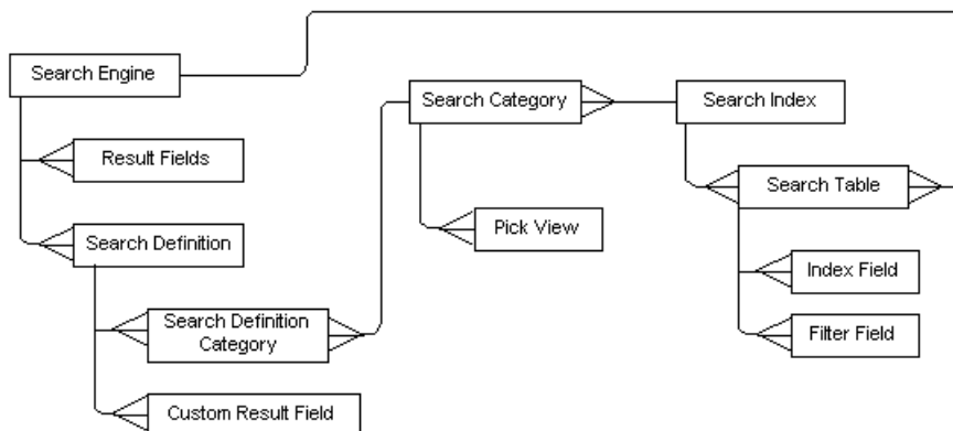
Figure 2. Search Objects in Siebel Tools
