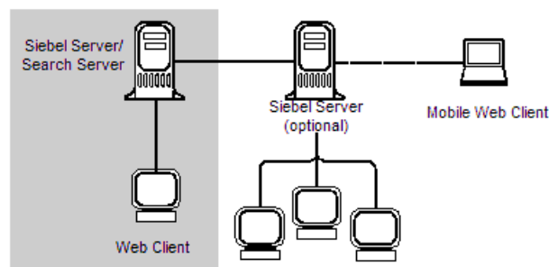
Figure 1. Siebel Search Architecture
