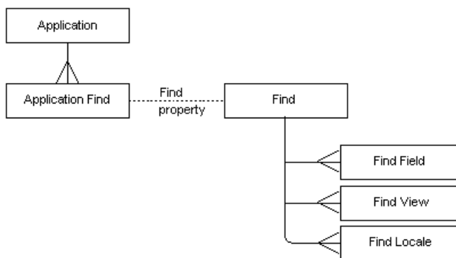
Figure 3. Find Tools Objects
