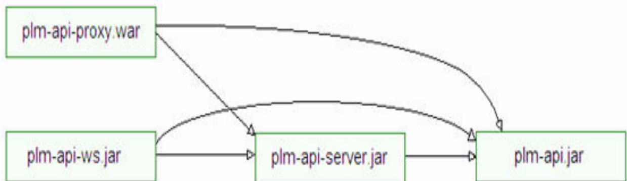
Figure 1-1: PLM-API component dependencies
