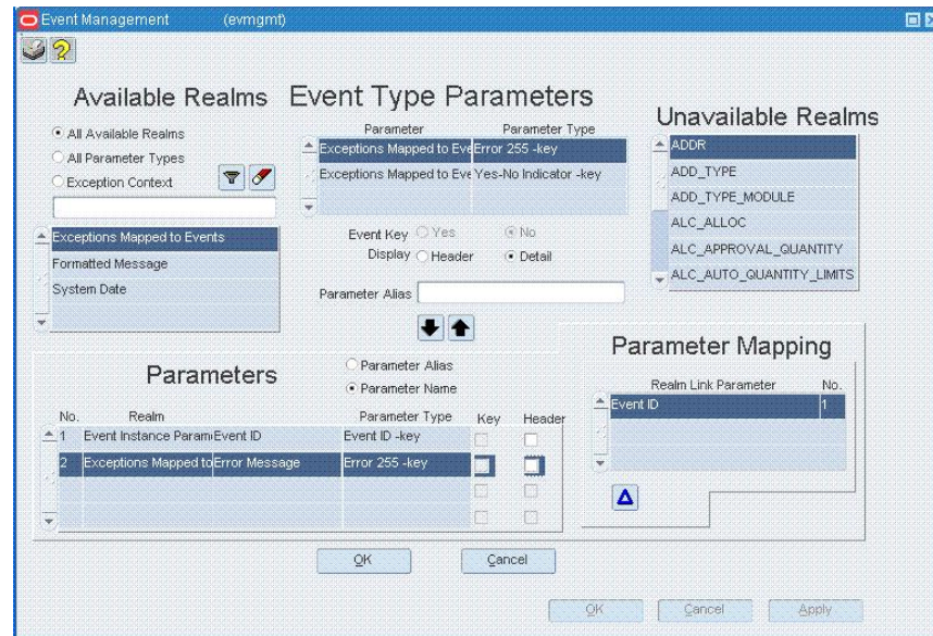
Figure 12–8 Exception Type Parameters Screen
