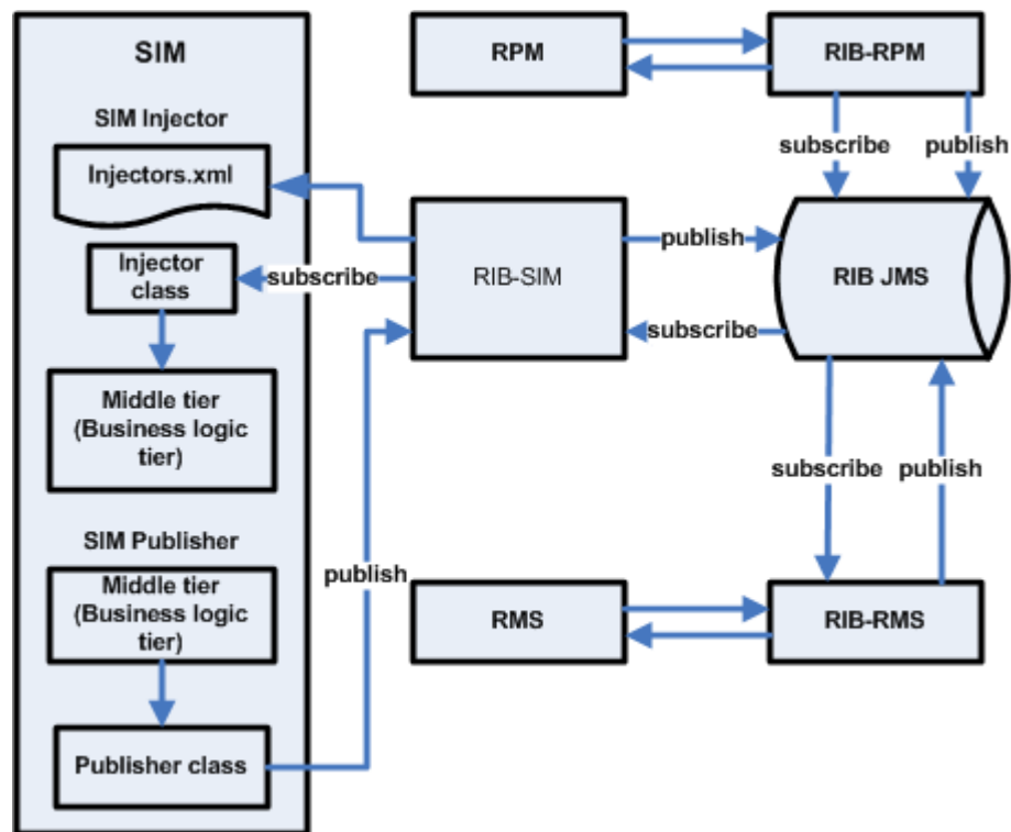
Figure 4–1 SIM/RIB Integration Diagram
