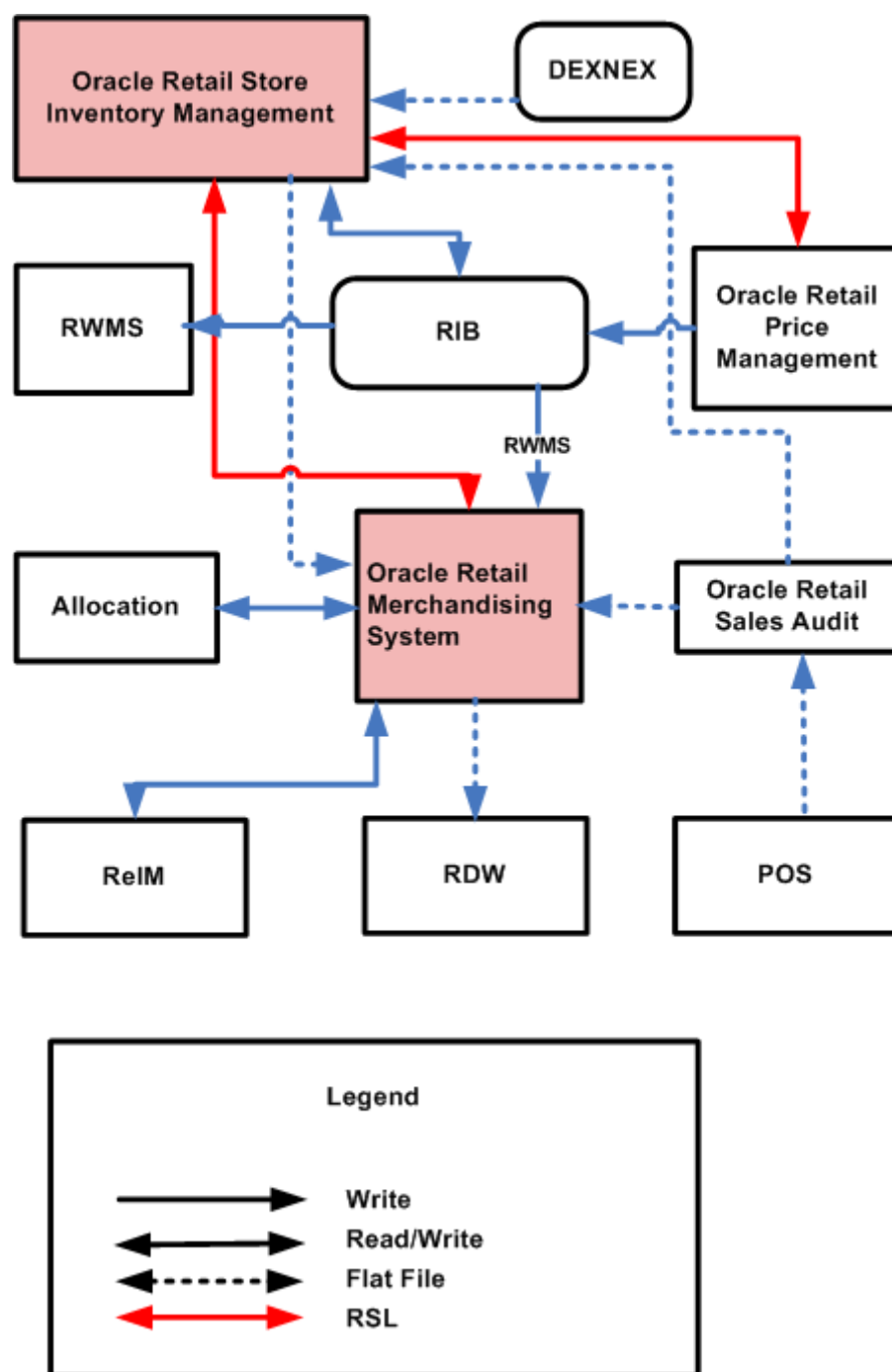
Figure 5–1 SIM Functional Dataflow
