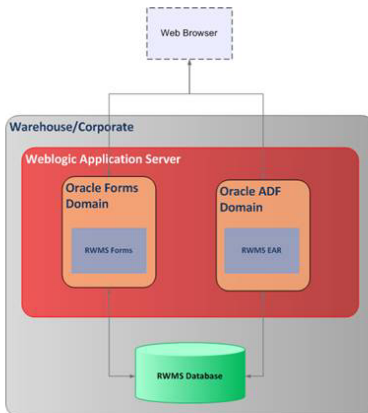
Figure 7-1 RWMS Architecture
