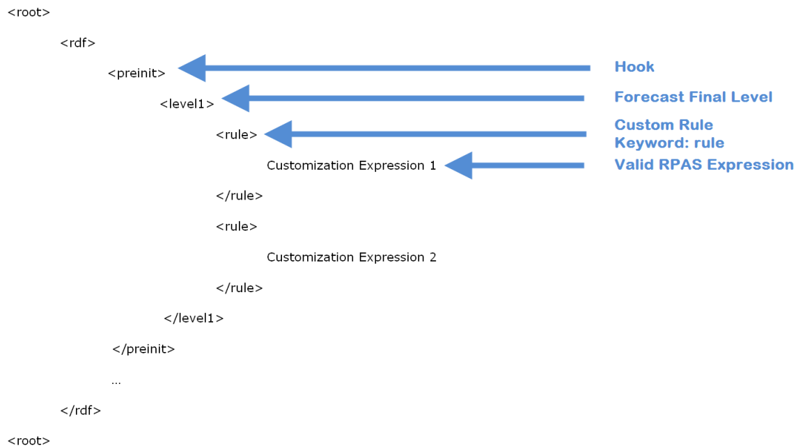
Figure D-1 Format of appcust.xml for RDF
