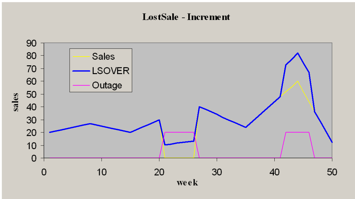
Example C-12 Lost Sales - Increment with delta = 0.5
