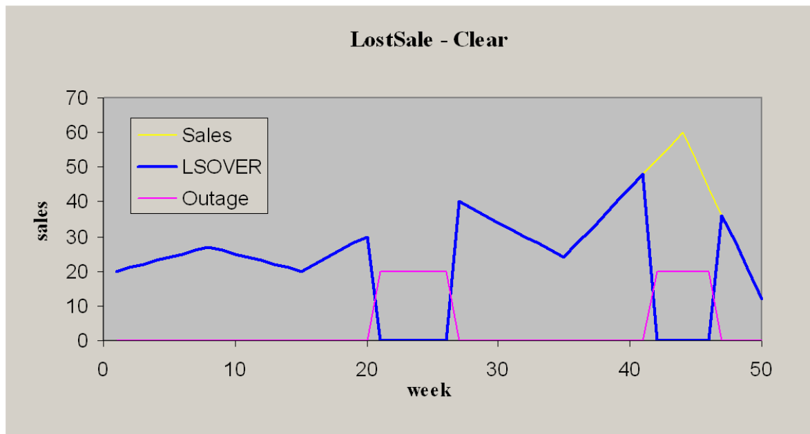
Figure C–9 LostSales - Clear with TS_Mask
