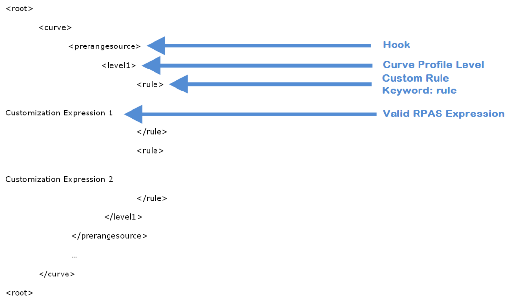
Figure D–2 Format of appcust.xml for Curve
