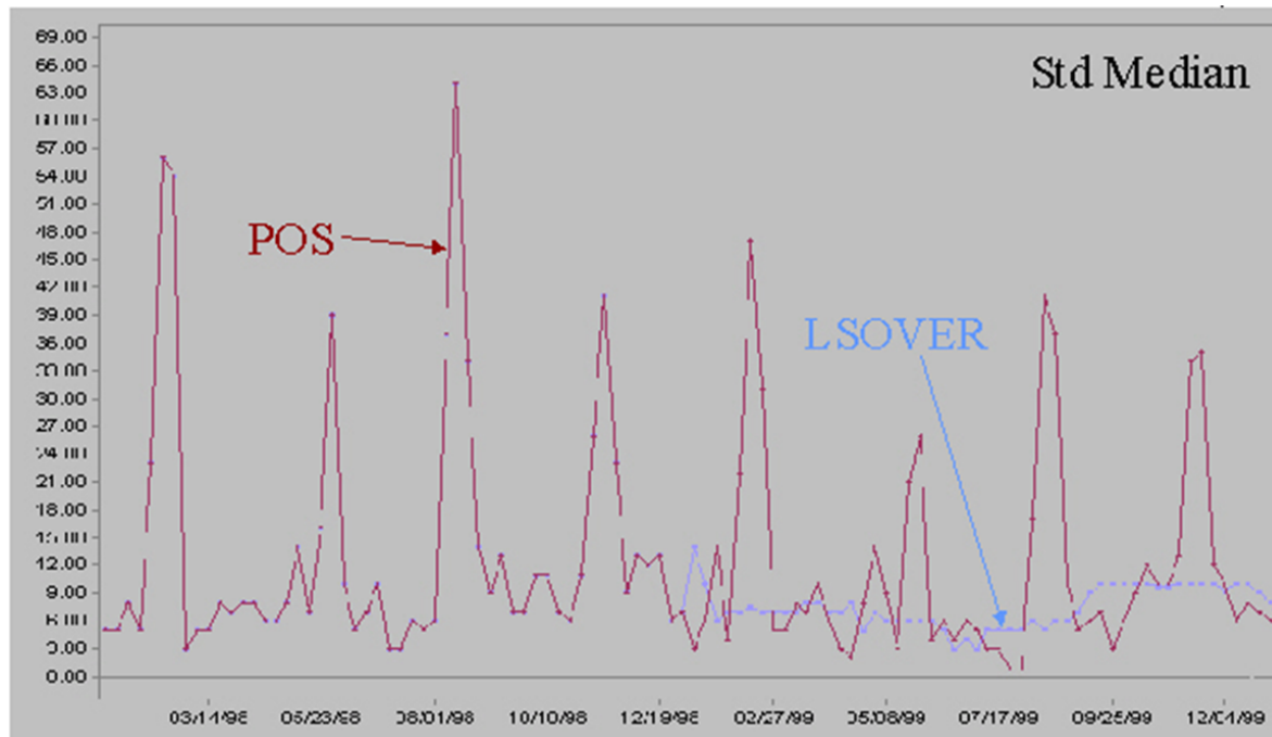
Example C-5 Std Median with window = 13 points
