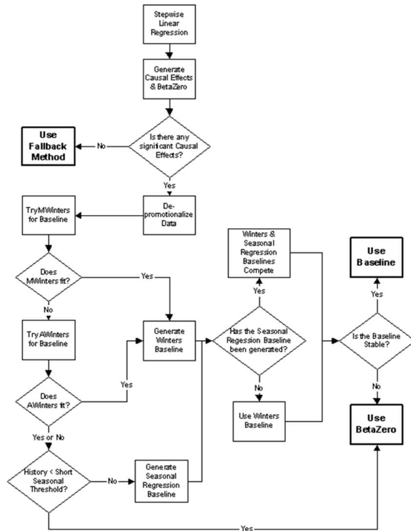
Figure 6–7 Causal Forecasting Process.
