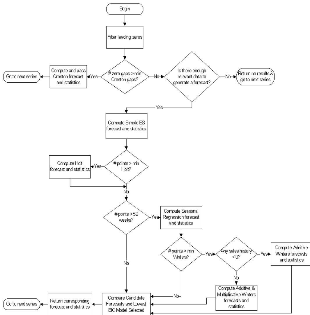
Figure 6–5 AutoES Flowchart
