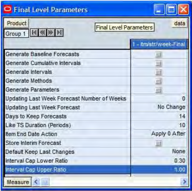
Figure 2–3 Final Level Parameters Worksheet
