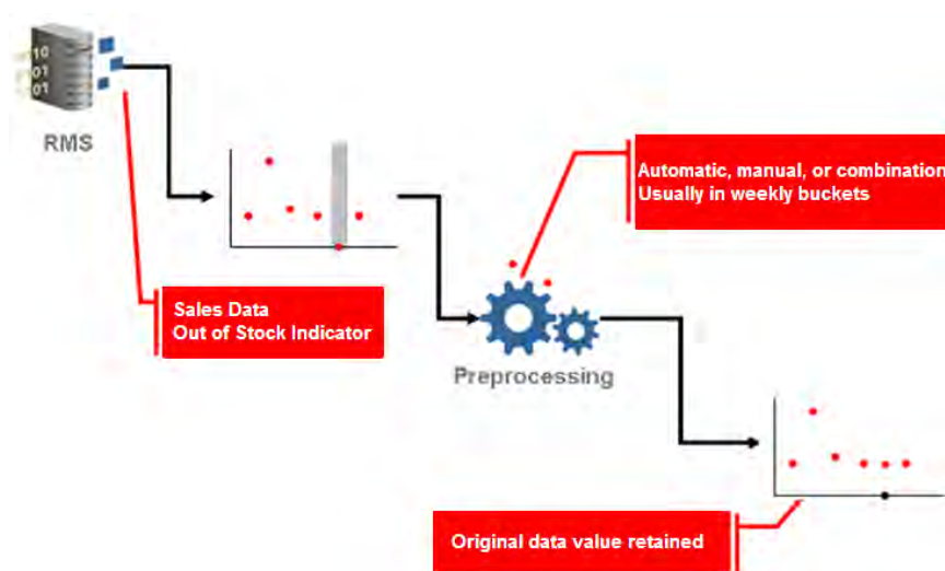
Figure 7-1 Preprocessing for Stock-outs
