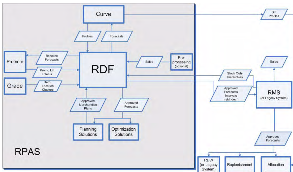
Figure 1–4 RDF and the Oracle Retail Enterprise
