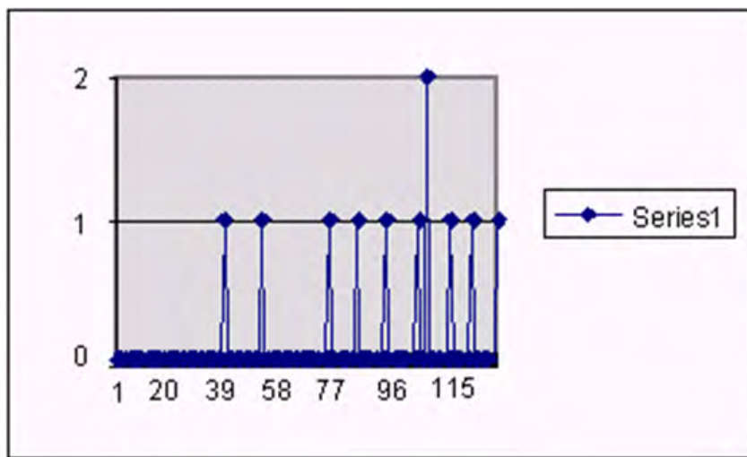
Figure 6–2 Croston's Method
