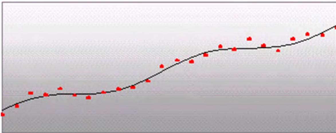
Figure 6–4 Multiplicative Winters Exponential Smoothing
