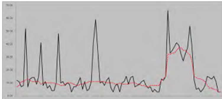
Figure 7–3 Standard Median Example
