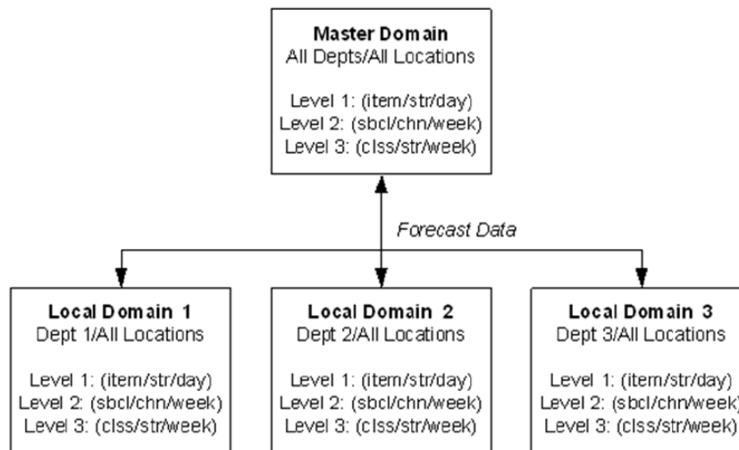
Figure 1–2 Global Domain versus Simple Domain Environment
