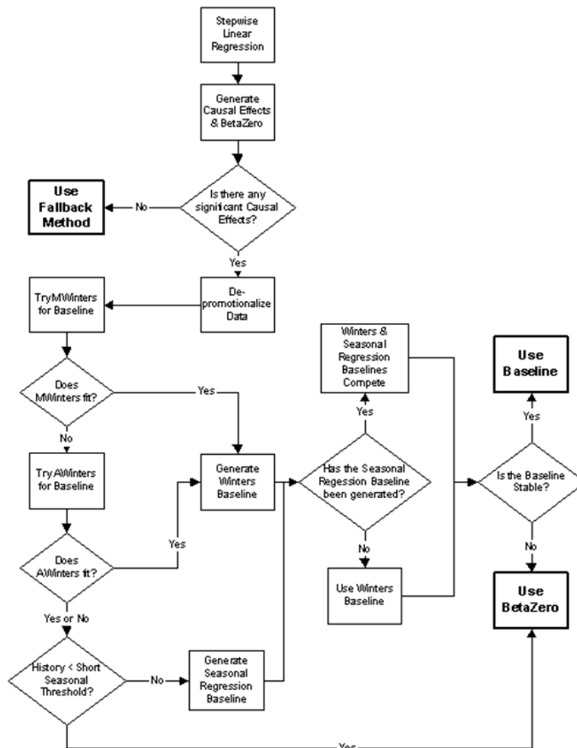
Figure 2–7 Causal Forecasting Process
