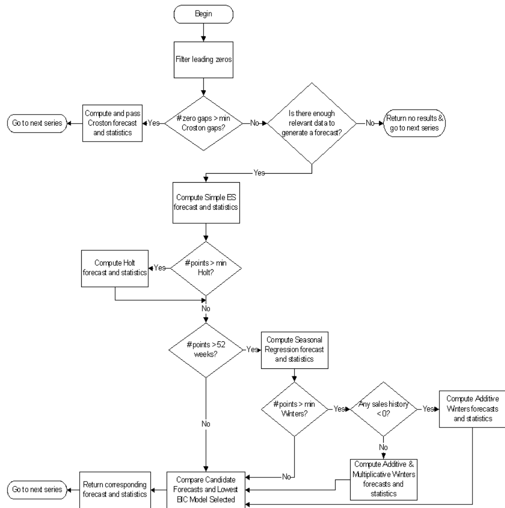
Figure 3-1 AutoES Flowchart
