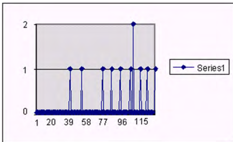
Figure 3-4 Croston's Method
