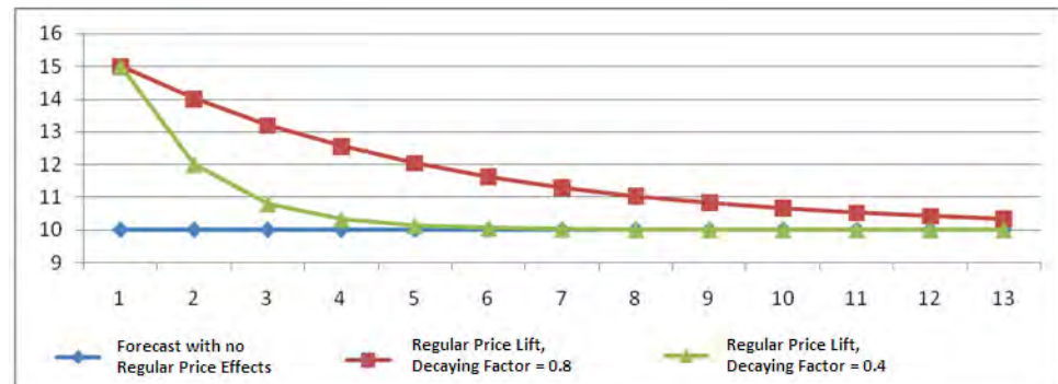
Figure 9–9 Regular Price Decaying Effect
