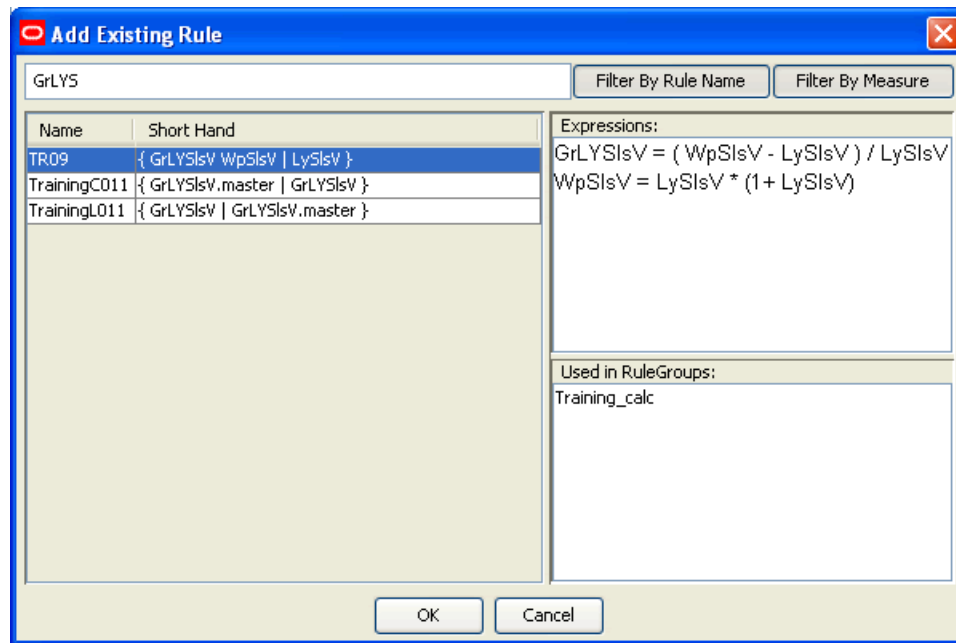
Example of Filter on GrLYS
