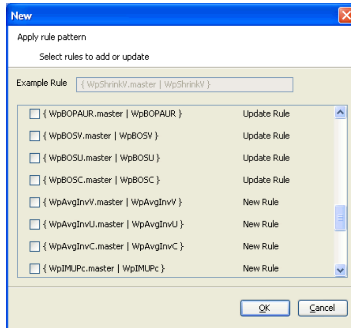
New – Apply New Pattern Dialog Box
