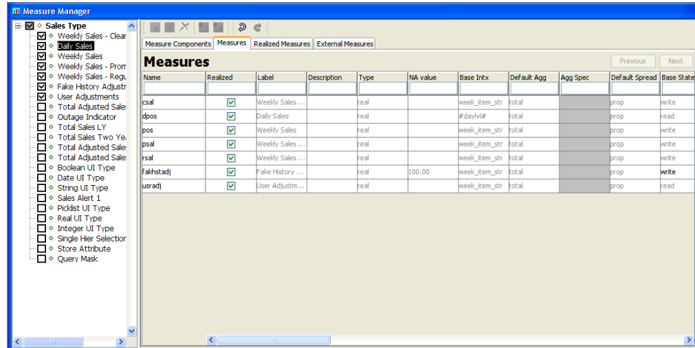
Example of Measure Manager - Measures Tab
