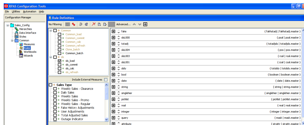
Rule Definition Window
