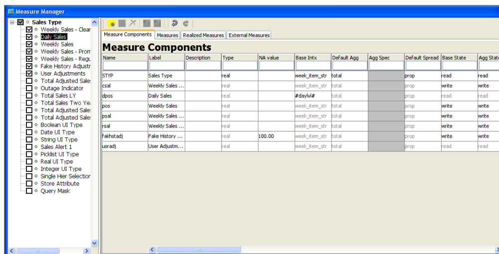
Example of Measure Manager Window - Measure Components Tab
