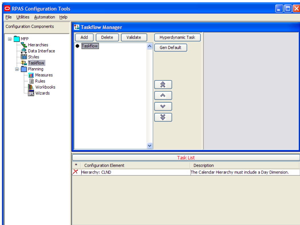
Taskflow Manager
