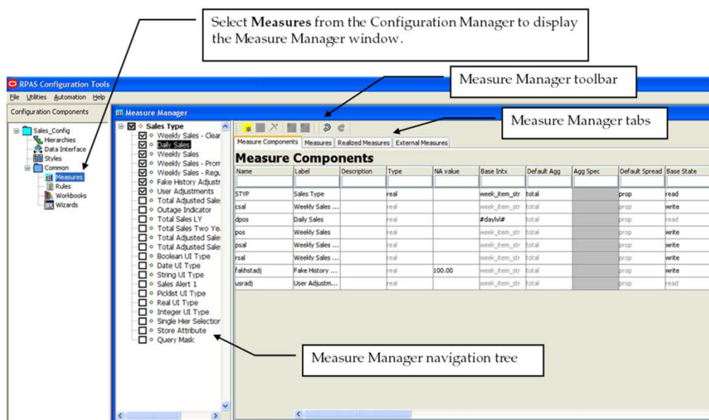
Example of Measure Manager Window
