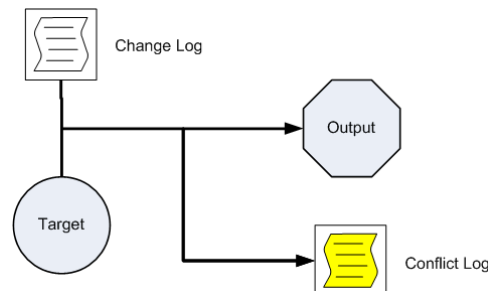
Merge Process
