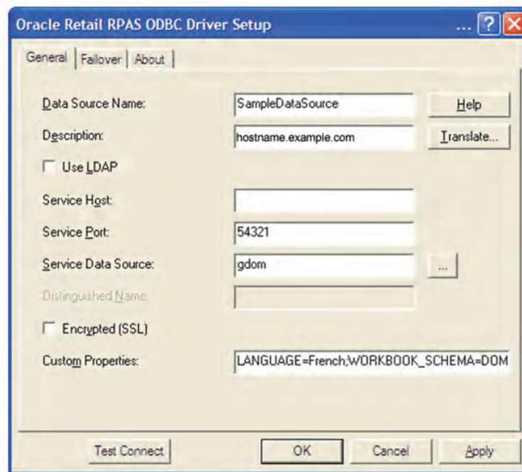
Figure 9–5 RPAS ODBC Driver Setup (Versions 13.1.2 and Later)
