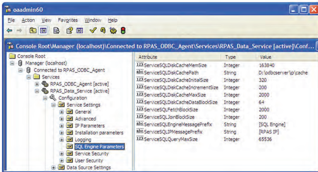
Figure 9–1 Server Configuration Attributes (Versions 13.1.2 and Later)
