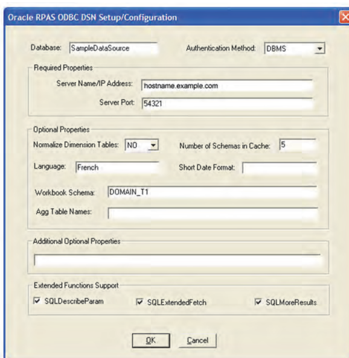
Figure 9–4 RPAS ODBC DSN Setup/Configuration for 13.0.x
