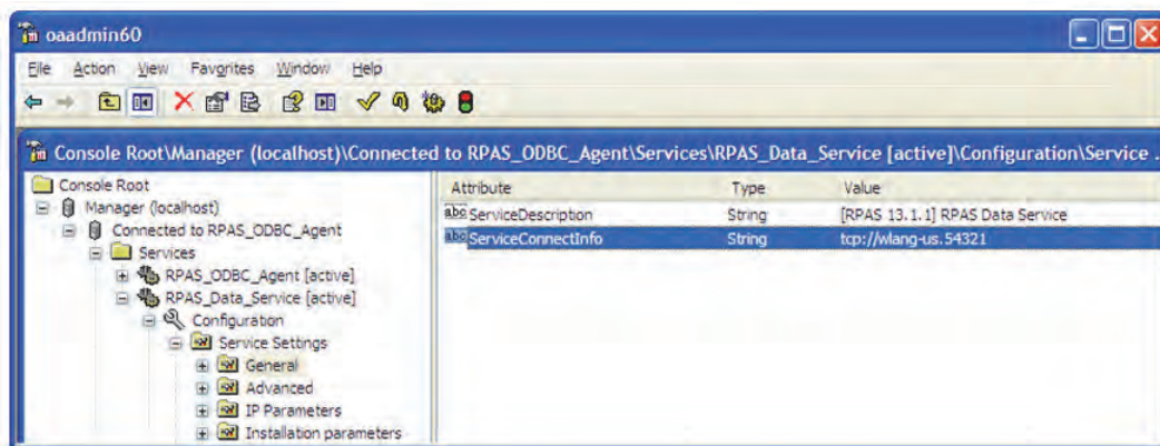
Figure 9–2 Server Address and Port Number (Versions 13.1.2 and Later)
