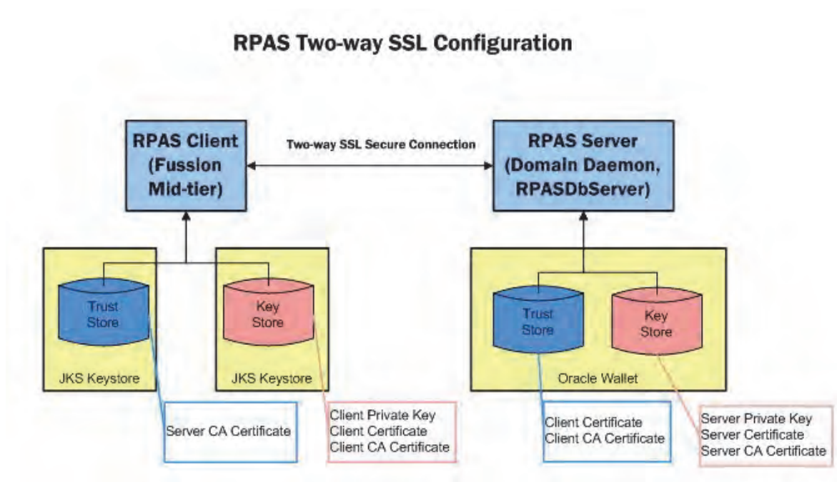
Figure 5–18 Configuration of Two-way SSL for RPAS
