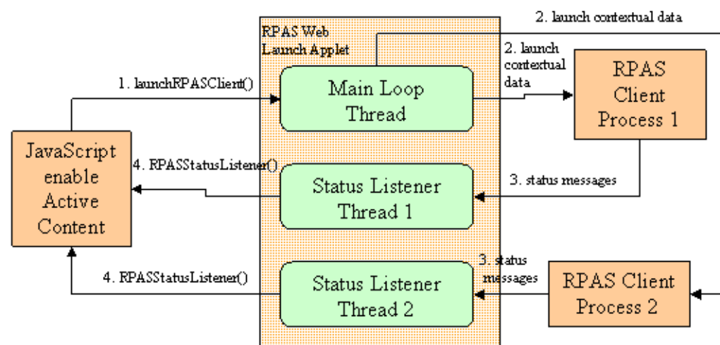
Figure 16-2 Two RPAS Clients Being Launched
