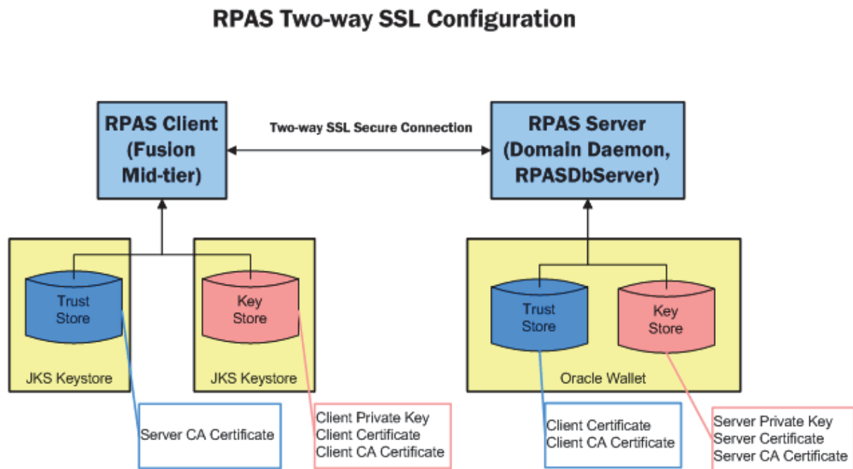
Figure 5–19 Configuration of Two-way SSL for RPAS
