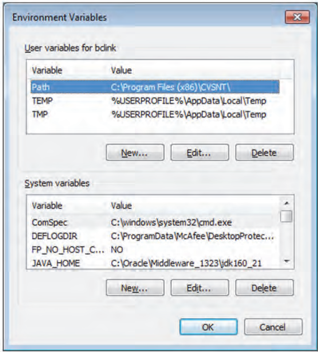
Figure 4-8 Environment Variables
