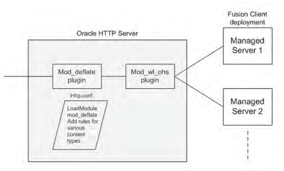
Figure 5-25 Implementing Gzip Compression
