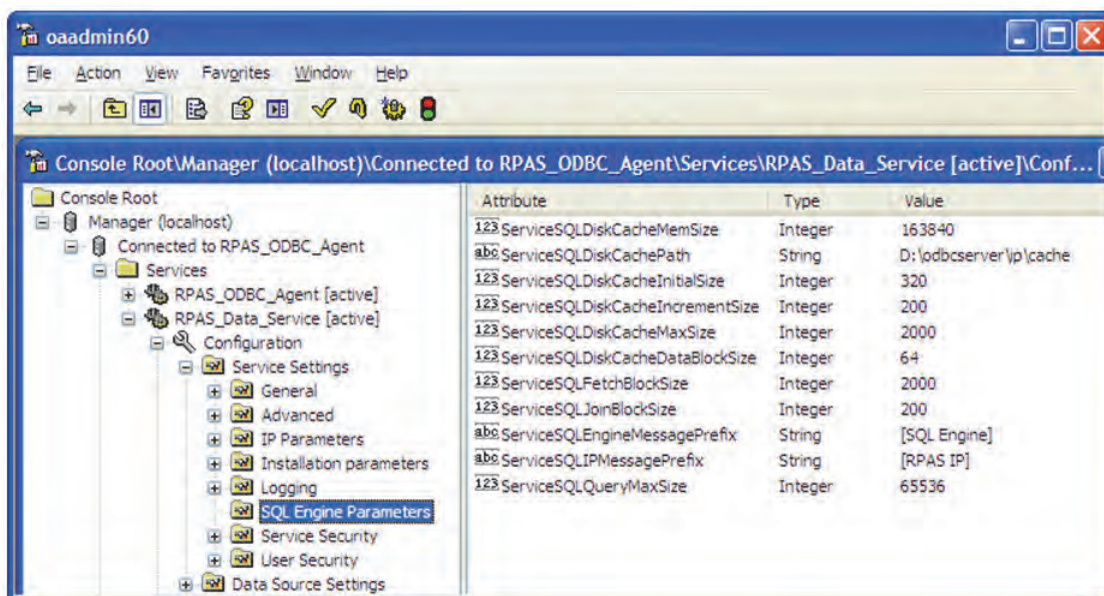
Figure 10–1 Server Configuration Attributes (Versions 13.1.2 and Later)
