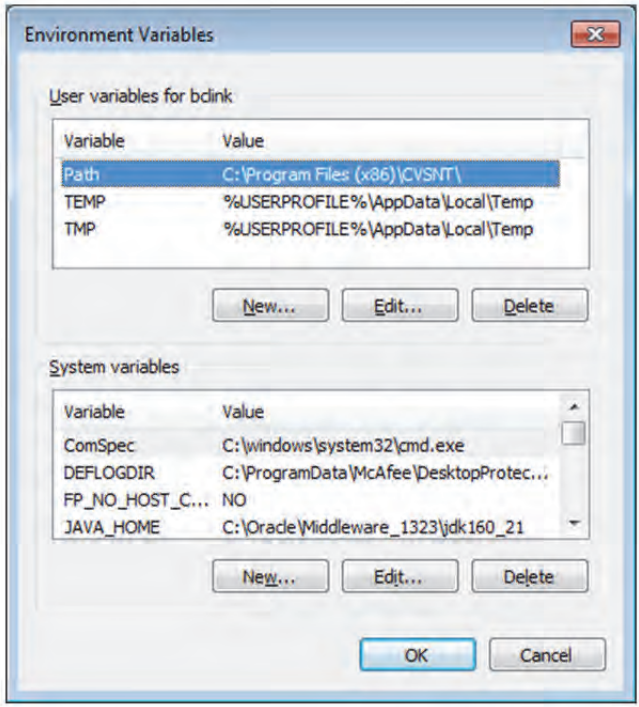
Figure 4-8 Environment Variables
