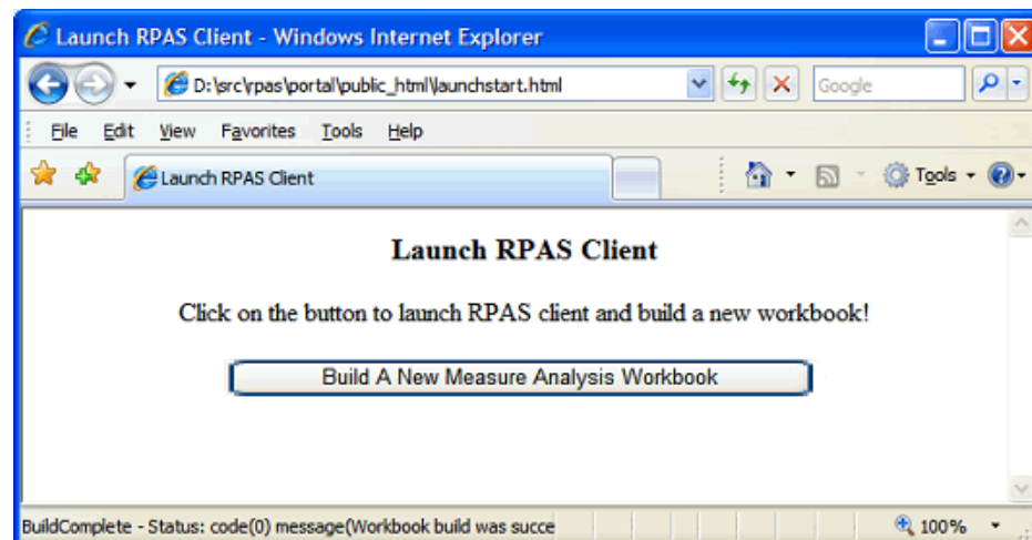
Figure 1-7 Guided Launch
