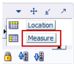
Figure 7-7 Measure Tile
