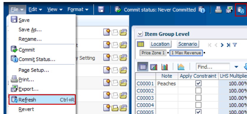
Figure 3–8 Single Refresh
