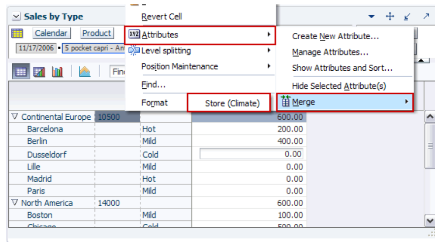
Figure 11-20 Merging Attributes
