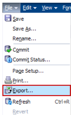
Figure 15–10 Export Option
