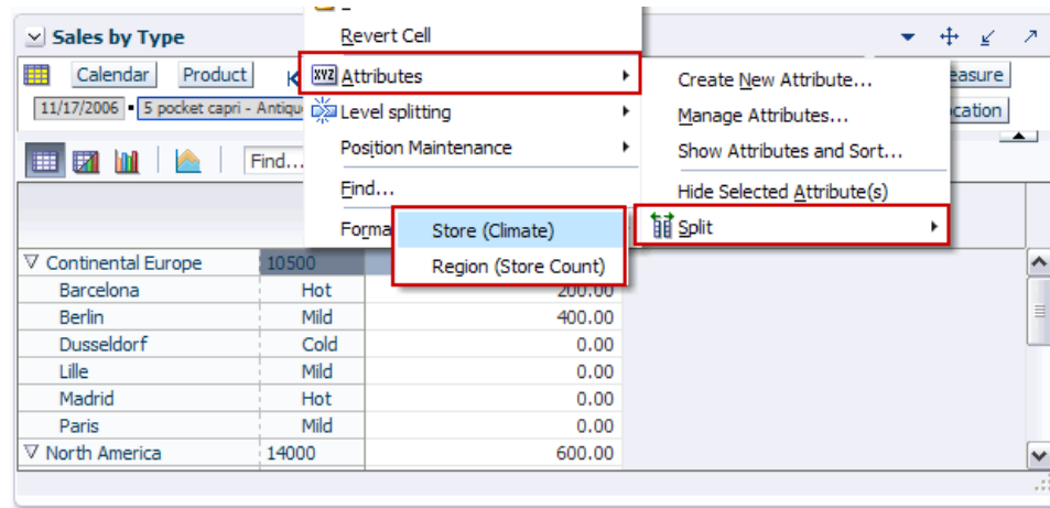
Figure 11–22 Splitting Attributes
