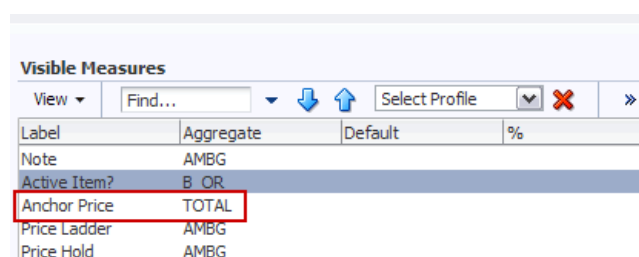
Figure 7-12 Inserted Measure
