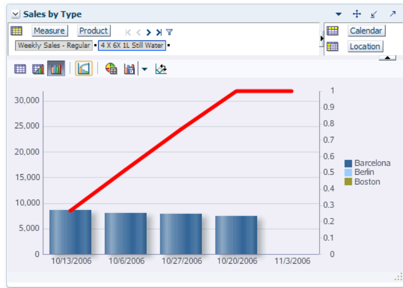
Figure 12-45 Pareto Chart
