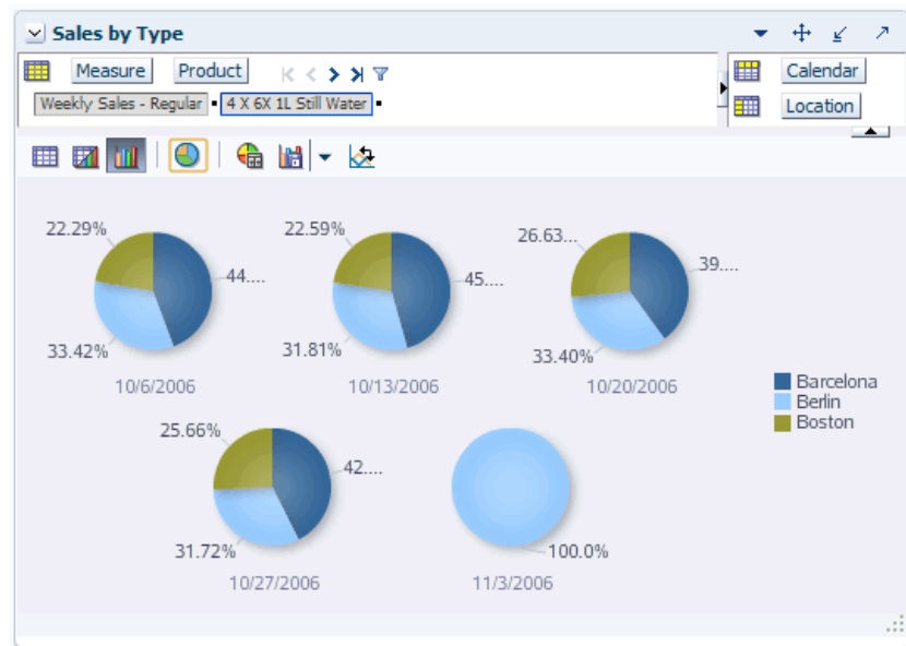
Figure 12-46 Pie Chart
