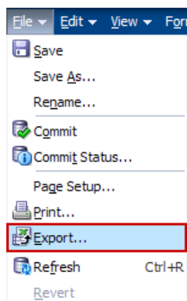
Figure 15–16 Export Option
