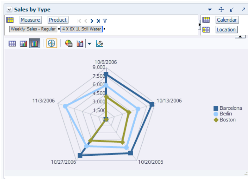
Figure 12–48 Radar Chart
