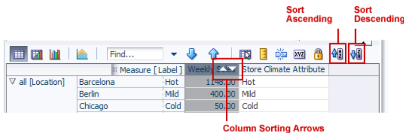
Figure 11-1 Sort Arrows
