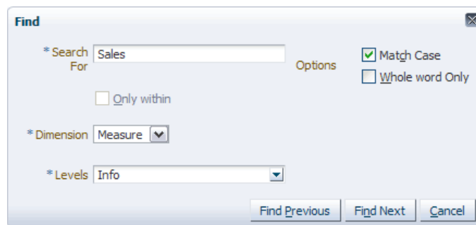
Figure 11–30 Find Window
