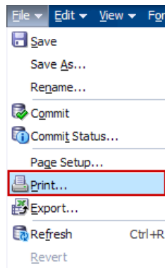
Figure 15–25 Print Option
