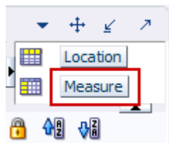
Figure 7-1 Measure Tile
