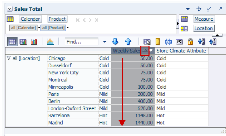
Figure 11-2 Sort Ascending
