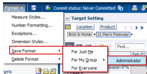
Figure 5–18 Save Format
