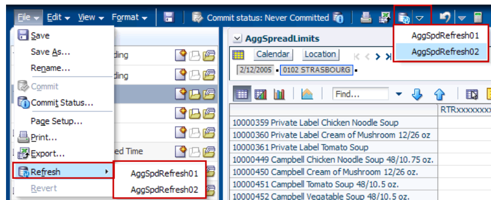
Figure 3–9 Multiple Refresh
