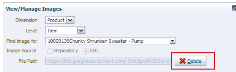
Figure 13–8 Delete Button
