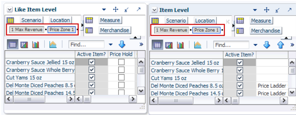
Figure 3–18 Synchronized Views
