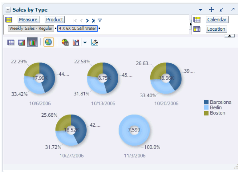
Figure 12–47 Ring Chart
