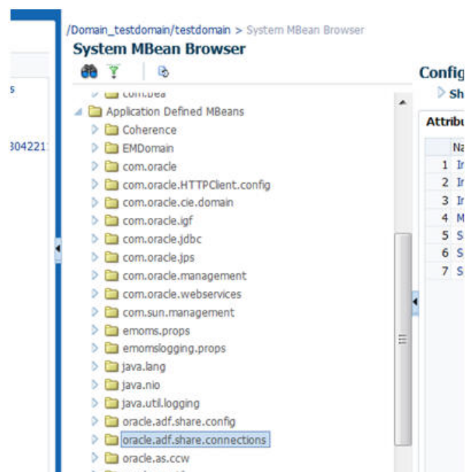
Figure 20–2 Node: oracle.adf.share.connections
